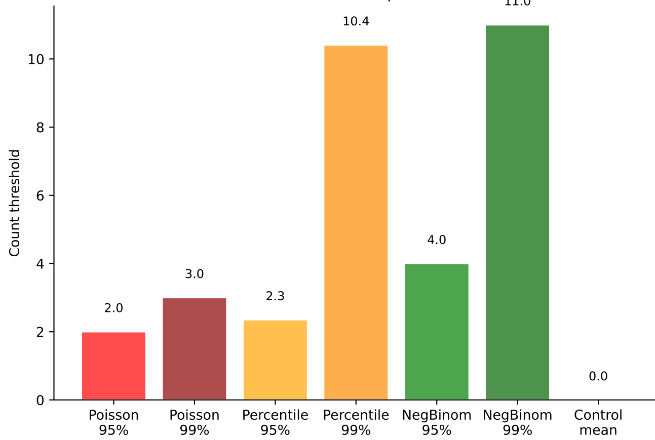
Threshold Comparison
