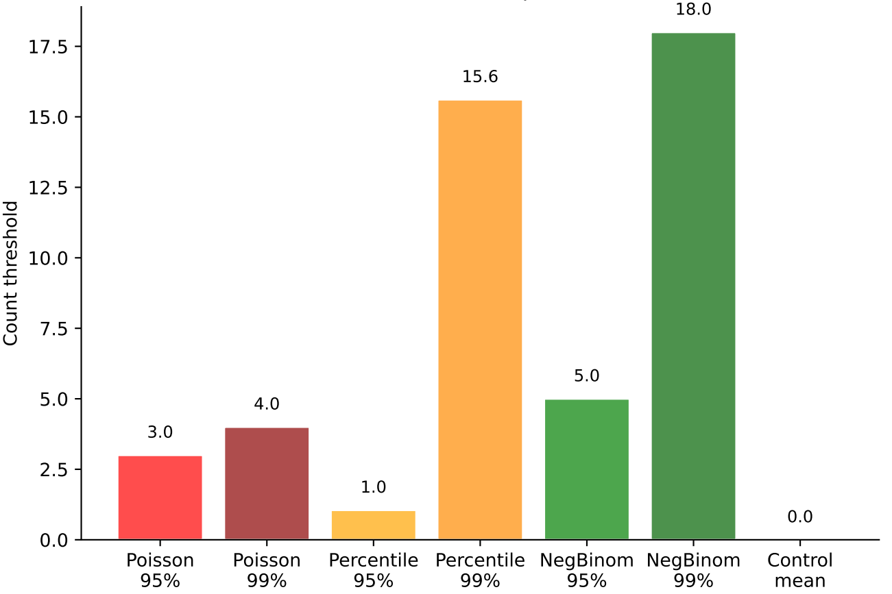
Threshold Comparison
