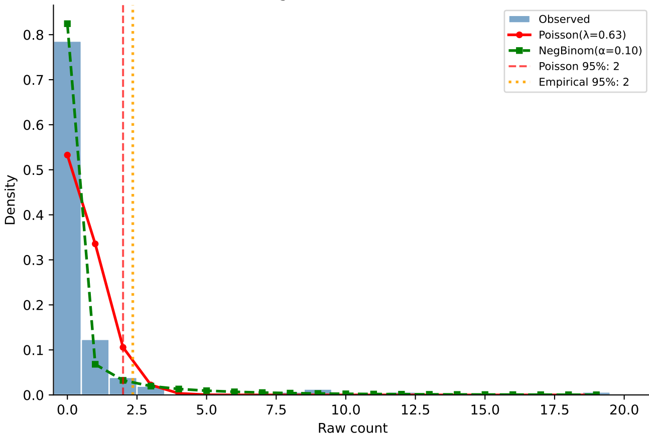
Threshold Comparison
