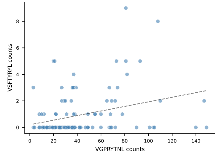
VSFTYRYL r=0.309 , p=7.29e-04
