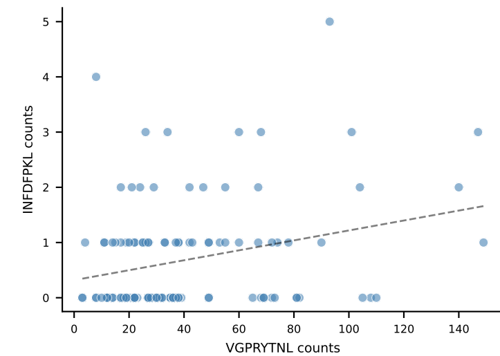
SSYTFPKM r=0.114 , p=2.21e-01
