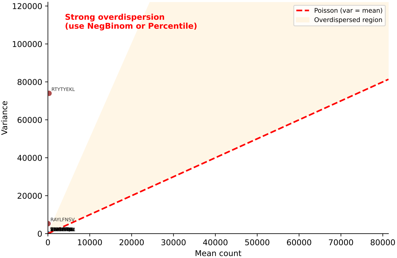
Variance vs Mean (Dispersion index: 16.42)
