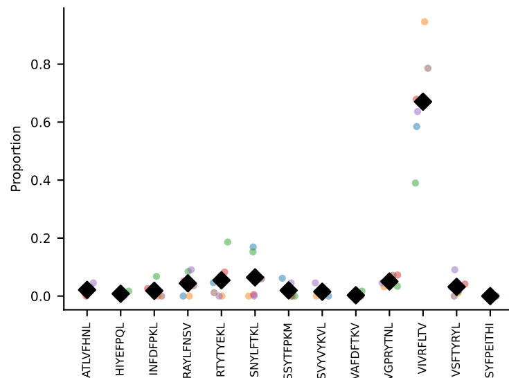
#91 AV6D-7-CALSEVSGGNYPKTF-AJ6_BV14-CASSLGANSYDTF-BJ1-2 coh=0.931, n=14
