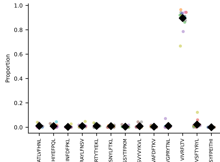
#24 AV16D/DV11-CAMREGLNNRIFF-AJ31_BV30-CSSRGLGGYEQYF-BJ2 coh=0.995, n=10
