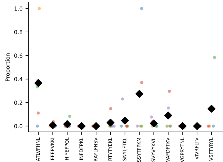
#36 AV8-1-CATSASSGSWQLIF-AJ22_BV13-2-CASGDEVSNERLFF-BJ1-4 coh=0.310, n=16
