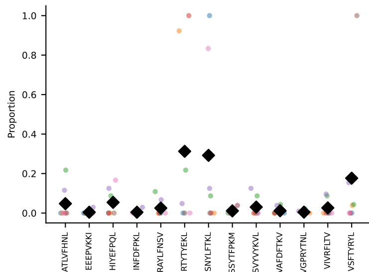
#43 AV16N-CAMREGTGGNNKLTF-AJ56_BV1-CTCRTGTDSYNSPLYF-BJ1-6 coh=0.258, n=5
