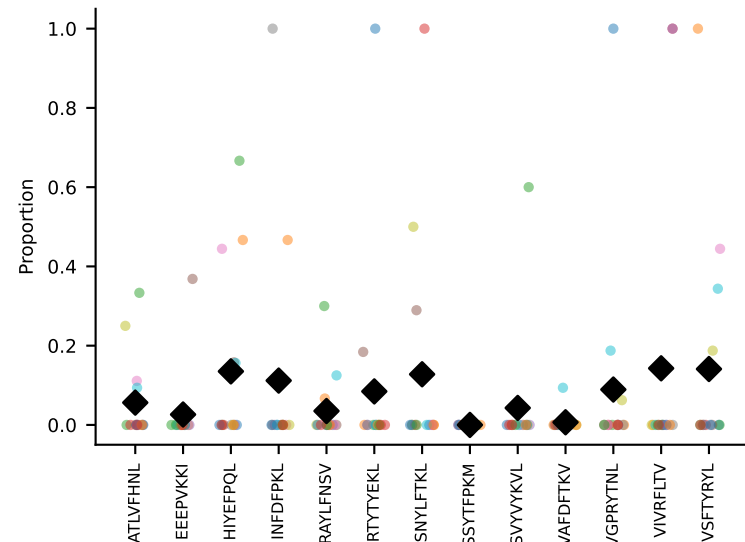
#129 AV12-2-CALSDDGSGGKLT-L-AJ44_BV1-CTCSADGGATEVFF-BJ1-1 coh=0.118, n=28
