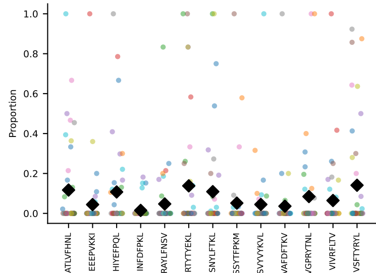
#90 AV7-3-CAVSPGGYKVVF-AJ12_BV13-2-CASGDAQGAGQLYF-BJ2-2 coh=0.170, n=19
