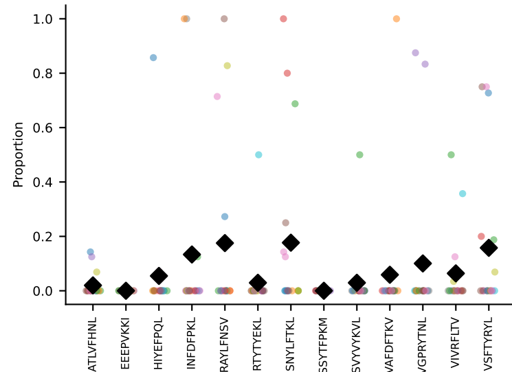
#125 AV15-1/DV6-1-CALWEPPHNNNAPRF-AJ43_BV16-CASSLRTGVYEQYF-BJ2-7 coh=0.126, n=14
