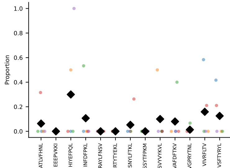
#127 AV7-2-CAAHNYAQLTF-AJ26_BV13-1-CASSDAGQGSGNTLYF-BJ1-3 coh=0.122, n=6
