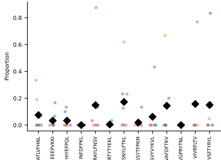
#83 AV8-1-CATDDGTNAYKVIF-AJ30_BV13-2-CASGAETLYF-BJ2-3 coh=0.176, n=7
