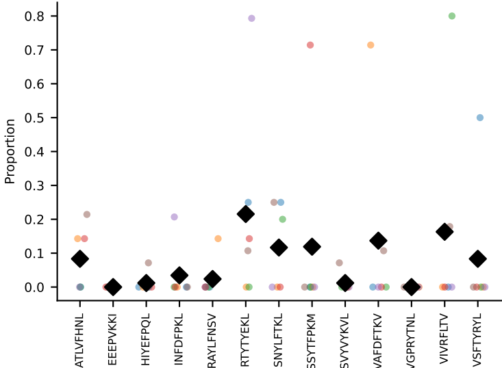
#101 AV8D-2-CATDQGQGRALIF-AJ15_BV3-CASSPQGHSDYTF-BJ1-2 coh=0.157, n=12
