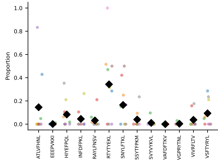
#29 AV9N-4-CALSIDTNAYKVIF-AJ30_BV31-CAWTDWGDQNTLYF-BJ2-4 coh=0.357, n=6
