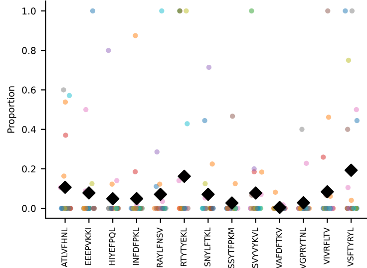
#106 AV16N-CAMREVYQGGRALIF-AJ15_BV16-CASSFVGNQDTQYF-BJ2-5 coh=0.153, n=22
