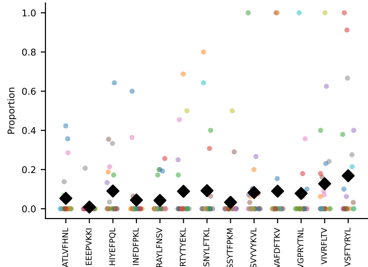
#84 AV14-3-CAARQGTQVVGQLTF-AJ5_BV1-CTCSGTGGDEQYF-BJ2-7 coh=0.175, n=24
