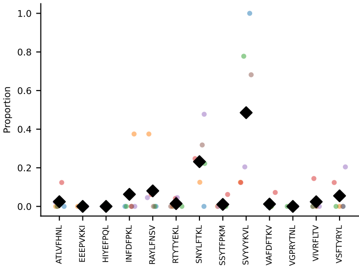
#17 AV16-CAMREANTGYQNfYF-AJ49_BV13-2-CASGTGGQNTLYF-BJ2-4 coh=0.498, n=36
