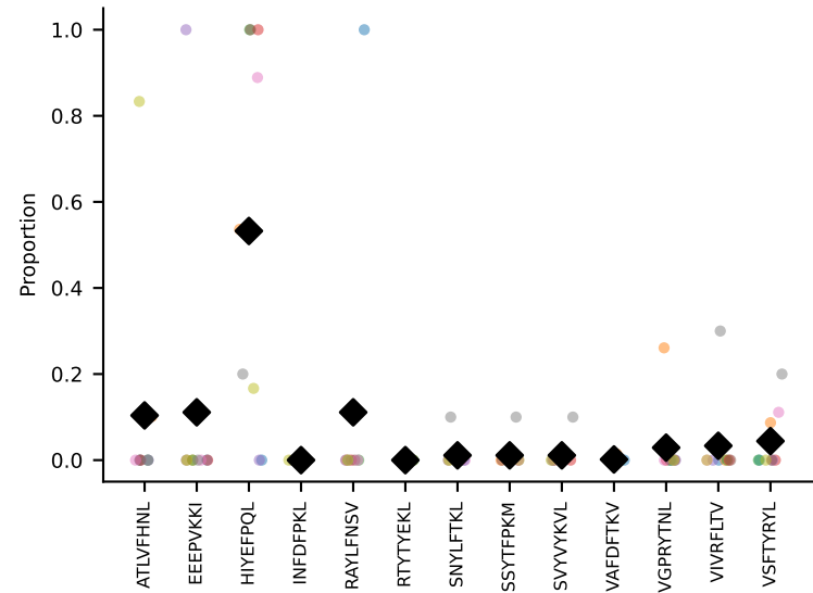
#32 AV8D-2-CATDNSNNRIFF-AJ31_BV5-CASSQGLGYAEQFF-BJ2-1 coh=0.329, n=5
