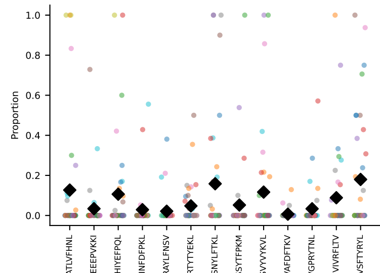
#69 AV14-3-CAASAGSGGKLTAL-AJ44_BV3-CASSLDFGQNTLYF-BJ2-4 coh=0.187, n=37
