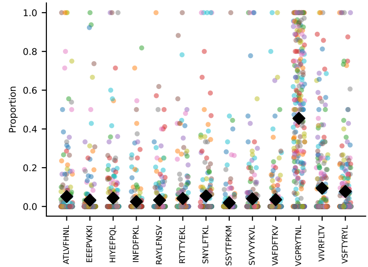
#24 AV16N-CAMRDNYAQGLTF-AJ26_BV3-CASSLGPSSYEQYF-BJ2-7 coh=0.403, n=279
