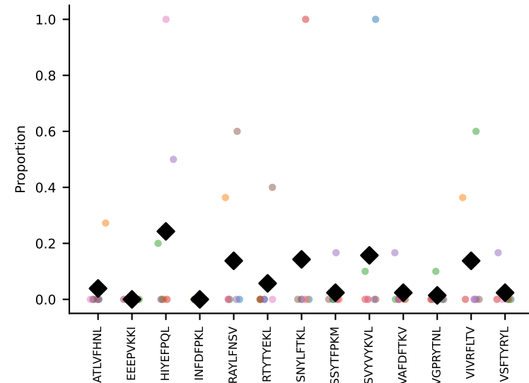
#128 AV4D-4-CAAEAVTGGYKVVF-AJ12_BV5-CASSPREGTGQLYF-BJ2-2 coh=0.119, n=9
