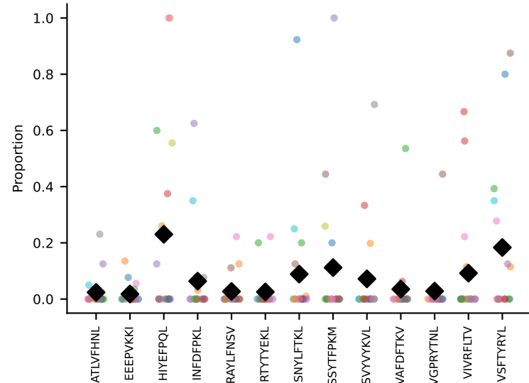
#66 AV4D-3-CAAYQGGRALIF-AJ15_BV1-CTCSGDRVAEQFF-BJ2-1 coh=0.200, n=5
