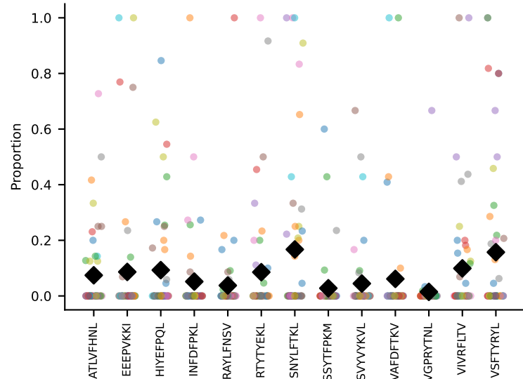
#79 AV7-2-CAAGNTGKLIF-AJ37_BV1-CTCSAVRVGYEQYF-BJ2-7 coh=0.179, n=49
