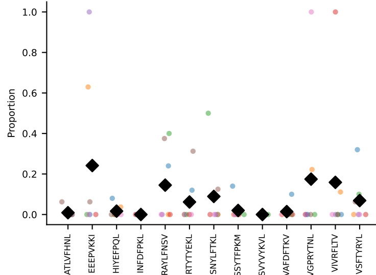
#102 AV7-6-CAVYGNEKITF-AJ48_BV5-CASSPDRGYTQYF-BJ2-5 coh=0.156, n=12
