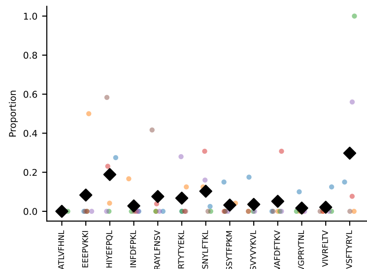
#48 AV14-2-CAASPYTGNYKYVF-AJ40_BV13-2-CASTNNNQAPLF-BJ1-5 coh=0.236, n=20
