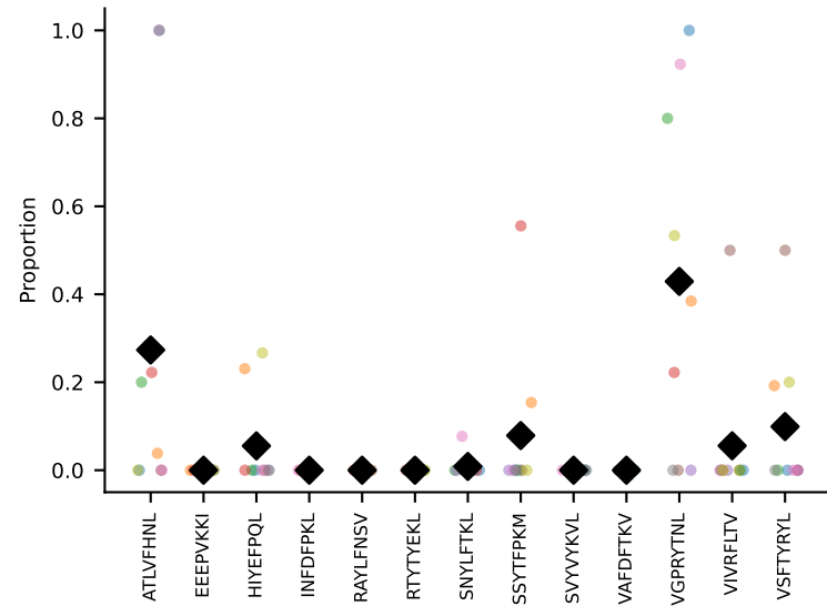
#30 AV4-4/DV10-CADMDYANKMIF-AJ47_BV2-CASSQDRGYNNQAPLF-BJ1-5 coh=0.350, n=87
