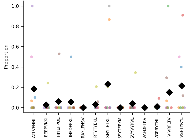
#103 AV9D-2-CVLSAANSAGNKLTF-AJ17_BV16-CASSLGEDTQYF-BJ2-5 coh=0.156, n=6
