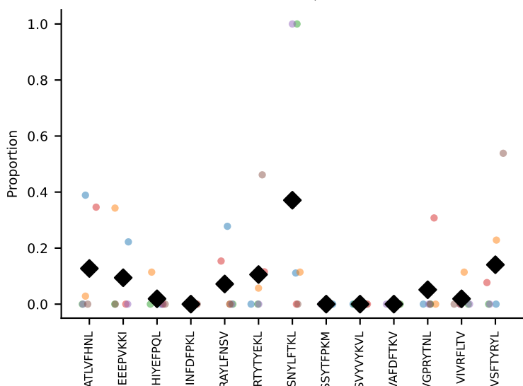
#45 AV13-2-CAIDGNTGKLIF-AJ37_BV31-CAWSLGHAEQFF-BJ2-1 coh=0.255, n=6
