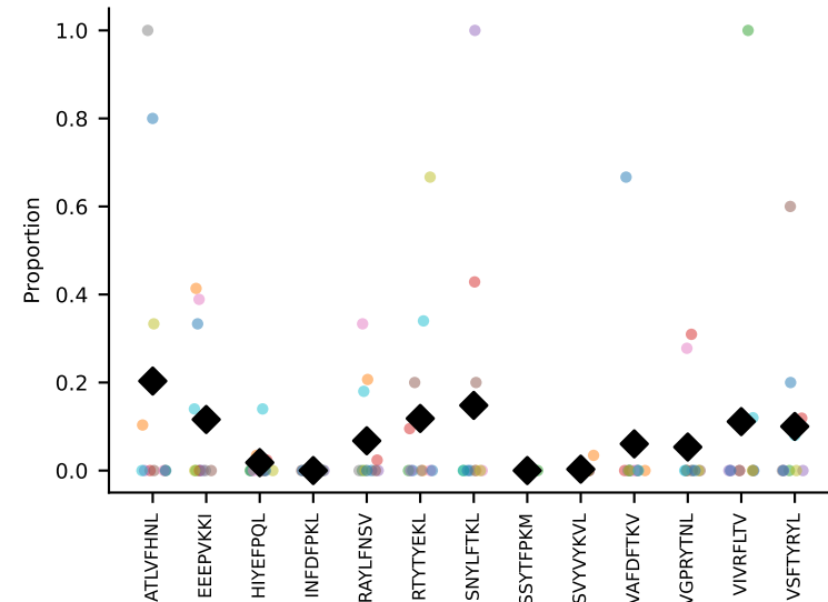
#92 AV16N-CAMREDQGGRALIF-AJ15_BV16-CASSLVGAQDTQYF-BJ2-5 coh=0.169, n=17
