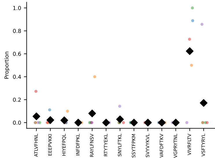
#19 AV15-2/DV6-2-CALSELGGNYKYVF-AJ40_BV13-2-CASGTGGENTLYF-BJ2-4 coh=0.481, n=74
