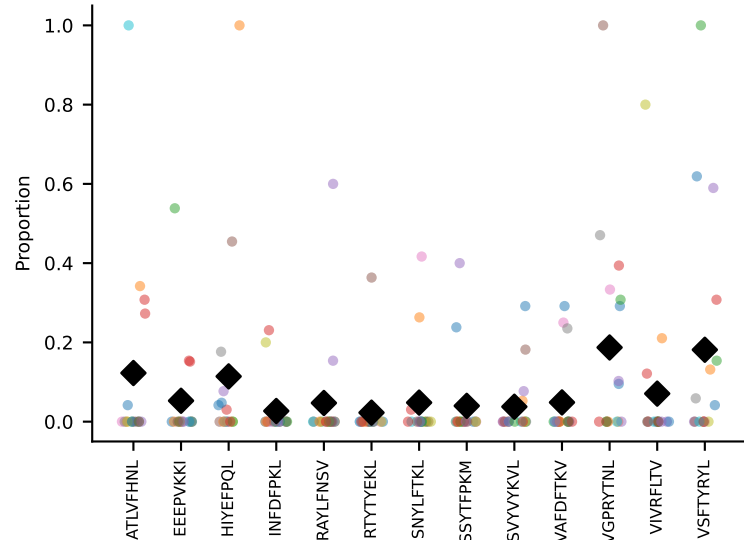
#67 AV8D-2-CATDTGGLSGKLTF-AJ2_BV13-1-CASSPGQYAEQFF-BJ2-1 coh=0.193, n=11
