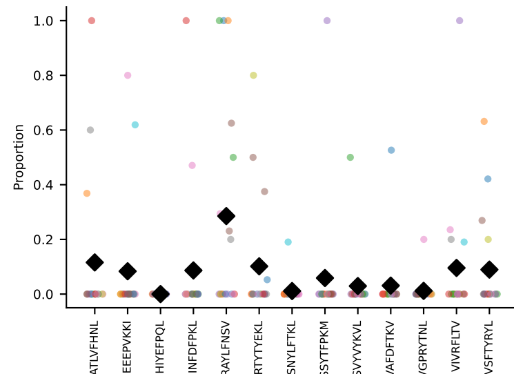
#95 AV14D-3/DV8-CAANYGSSGNKLI-AJ32_BV1-CTCSAVRVQDTQYF-BJ2-5 coh=0.165, n=17
