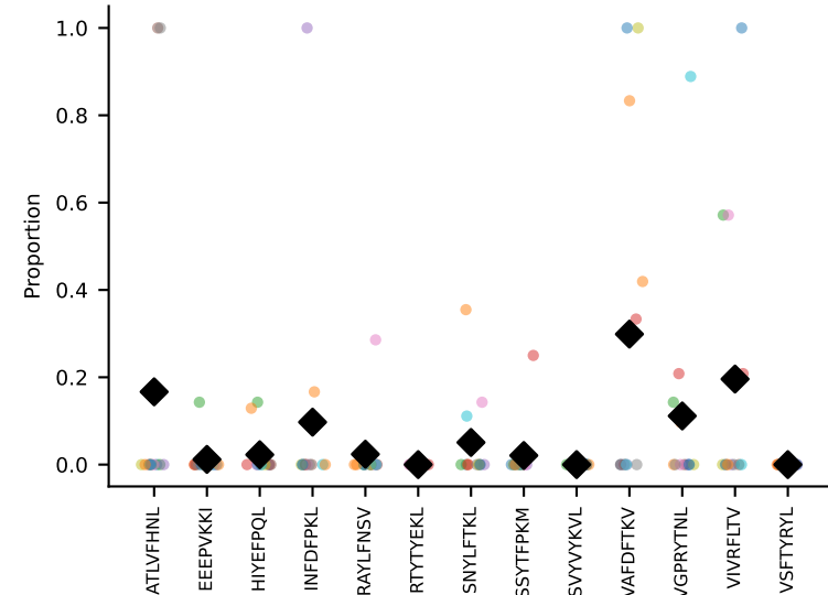
#65 AV9D-2-CVLSAVGDN SKLIW-AJ38_BV19-CASSIGRFGNTLYF-BJ1-3 coh=0.200, n=7
