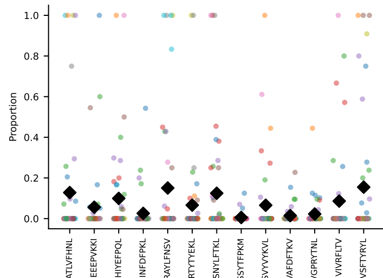
#94 AV9-2-CVLSVTGSGGKLT-L-AJ44_BV14-CASSFANTGQLYF-BJ2-2 coh=0.167, n=45
