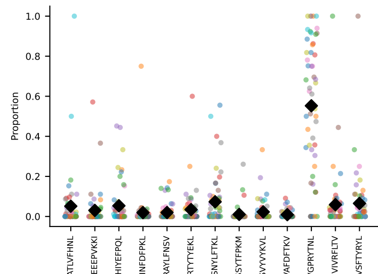
#9 AV14-2-CAASGDYAQGLTF-AJ26_BV3-CASSLGQDTQYF-BJ2-5 coh=0.595, n=53
