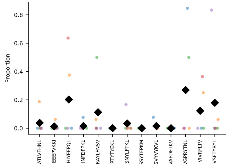
#138 AV7D-6-CAGNYSNNRLTL-AJ7_BV16-CASSLNWGAN YAEQFF-BJ2-1 coh=0.176, n=11
