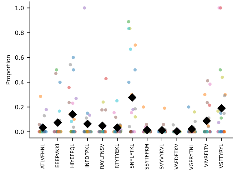
#53 AV3D-3-CAVSDYNVLYF-AJ21_BV3-CASSQYLRLDNQDTQYF-BJ2-5 coh=0.321, n=39
