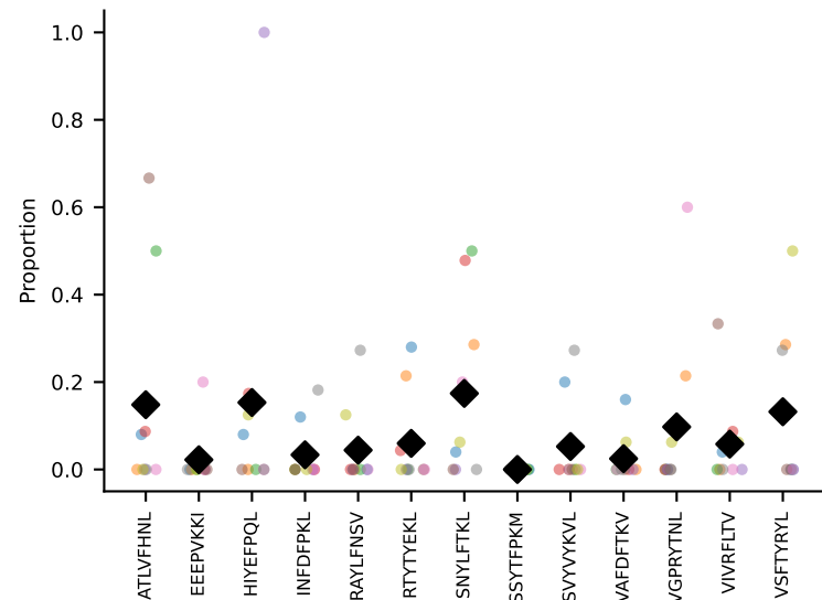
#114 AV13D-2-CAIDTNTGKLT-F-AJ27_BV26-CASSLDRAITGQLYF-BJ2-2 coh=0.226, n=6
