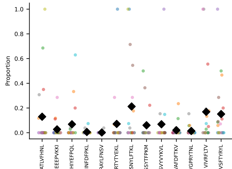
#126 AV7-2-CAADNVGDNSKLIW-AJ38_BV4-CASSPGTGYSYTF-BJ1-2 coh=0.205, n=6
