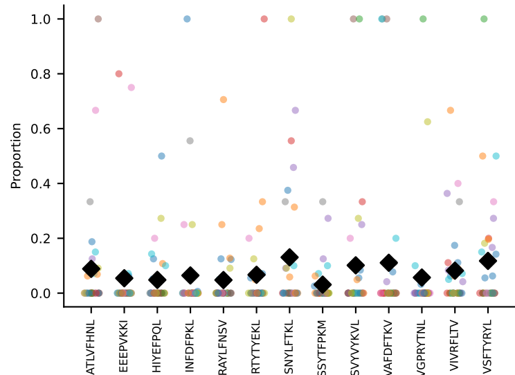
#139 AV3-1-CAVSGQGGRALIF-AJ15_BV13-1-CASRGTA YE QYF-BJ2-7 coh=0.168, n=5
