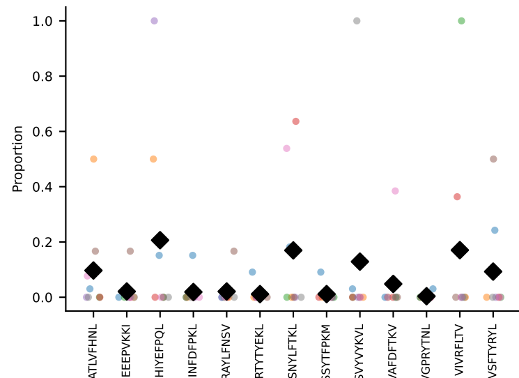
#141 AV14-2-CAATASSGSWLQIF-AJ22_BV13-2-CASGDWGG EVETLYF-BJ2-3 coh=0.156, n=6
