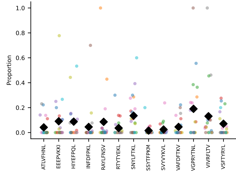
#56 AV14D-3/DV8-CAASASSGSWQLIF-AJ22_BV31-CAWSPLQGANTTEVFF-BJ2-1 coh=0.316, n=12
