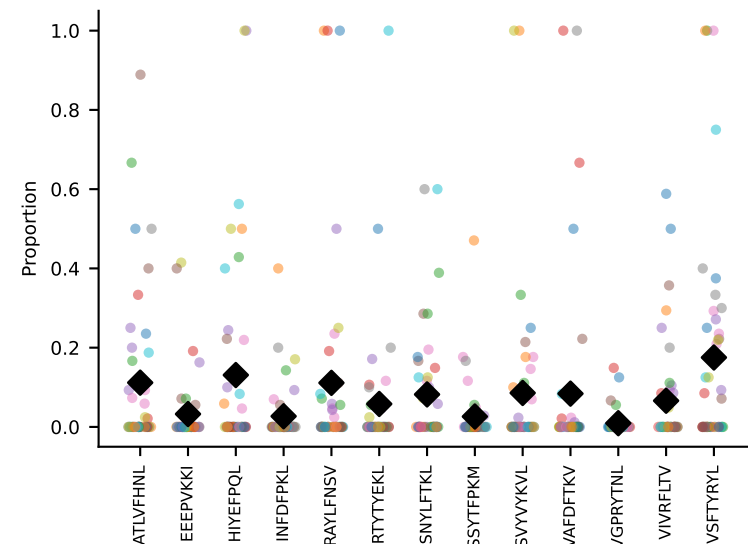
#117 AV7-5-CAVSMDYANKMIF-AJ47_BV3-CASSFGATYEQYF-BJ2-7 coh=0.222, n=27
