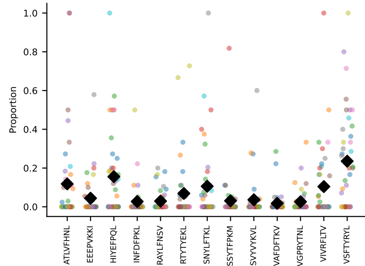
#57 AV3-3-CAVRITGNTGKLIF-AJ37_BV17-CASSSGYEQYF-BJ2-7 coh=0.315, n=5
