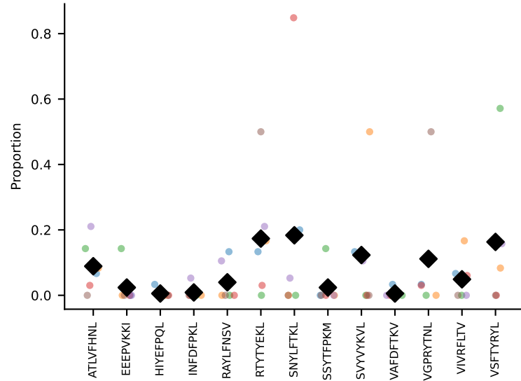
#55 AV6D-7-CALGANYNQGKLIF-AJ23_BV1-CTCSAGLGKDTQYF-BJ2-5 coh=0.317, n=6
