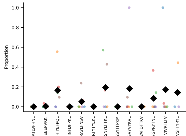
#118 AV16-CAMREAEGNEKITF-AJ48_BV1-CTCSAVRVGSDYTF-BJ1-2 coh=0.218, n=5
