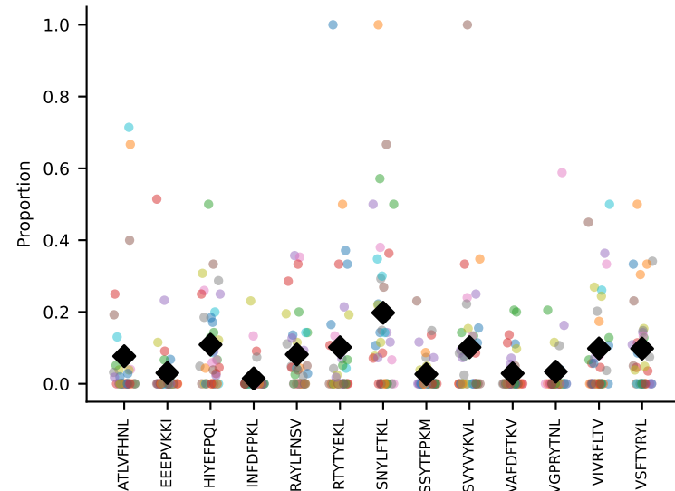
#41 AV16N-CAMREETGNTGKLIF-AJ37_BV1-CTCSANRVDLTQYF-BJ2-5 coh=0.351, n=10
