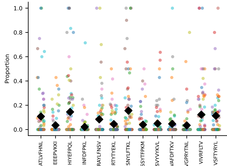
#107 AV7-3-CAGQGGRALIF-AJ15_BV1-CTCSADQNSGNTLYF-BJ1-3 coh=0.234, n=6
