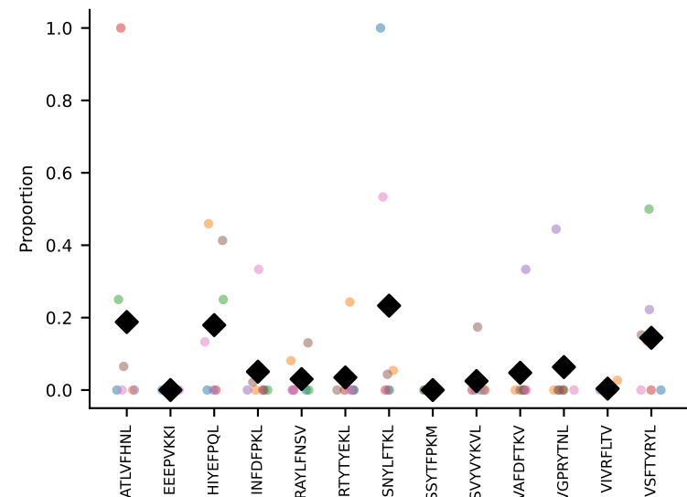
#120 AV14-2-CAASGTGYQNIFY-AJ49_BV2-CASSQAWGNQDTQYF-BJ2-3 coh=0.216, n=11
