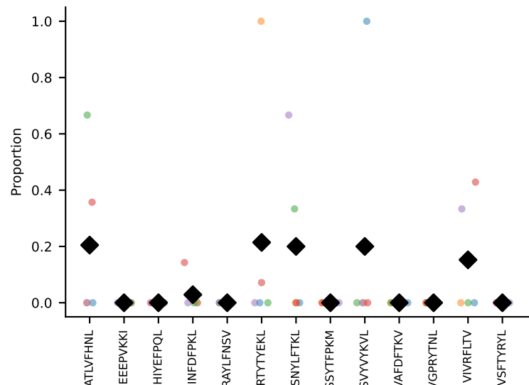
#142 AV11-CVVGRRYRGSSGNKLIF-AJ32_BV19-CASSTDRGLNSPLYF-BJ1-6 coh=0.155, n=8
