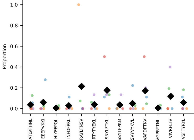
#81 AV9-2-CVLSARSGGSNAKLTf-AJ42_BV1-CTCSSQNTLYF-BJ2-4 coh=0.270, n=5
