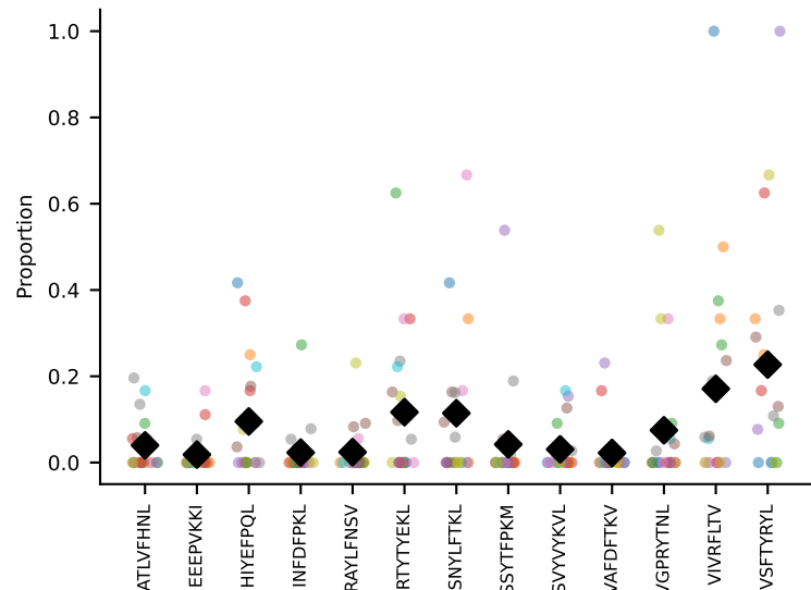
#48 AV7-4-CAASSDTNAYKVIF-AJ30_BV2-CASSQRTGVNTLYF-BJ2-4 coh=0.338, n=7
