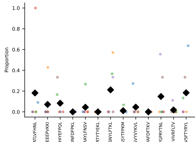
#130 AV8N-2-CATVIRGGRALIF-AJ15_BV19-CASSIGTGENTLYF-BJ2-4 coh=0.194, n=6
