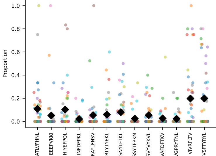
#77 AV7D-5-CAVRDTGGLSGKLTf-AJ2_BV1-CTCSADRLGSAETLYF-BJ2-3 coh=0.272, n=7
