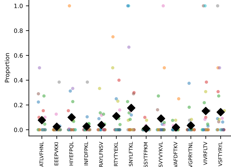
#83 AV14-2-CAAGASSGSWQLIF-AJ22_BV31-CAWSLAGSGNTLYF-BJ1-3 coh=0.269, n=44
