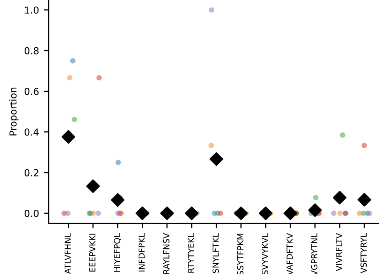
#80 AV13D-2-CAIYQGGRALIF-AJ15_BV1-CTCSADRGNSYNSPLYF-BJ1-6 coh=0.270, n=11
