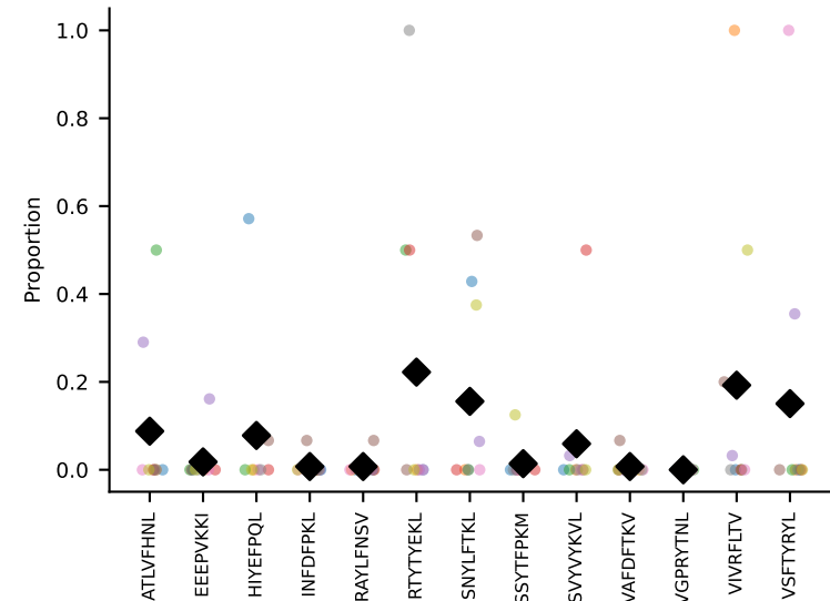
#137 AV6-6-CALGDLTGGNKLTf-AJ56_BV13-3-CASKDRGREQYF-BJ2-7 coh=0.176, n=21
