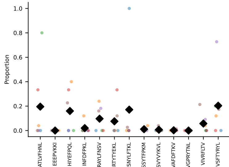
#102 AV8N-2-CATESQGGRALIF-AJ15_BV3-CASSDRAGQDTQYF-BJ2-5 coh=0.247, n=11
