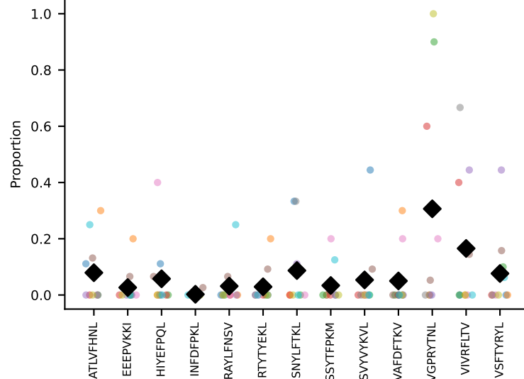
#78 AV12D-2-CALDYANKMIF-AJ47_BV14-CASSFRAEQFF-BJ2-1 coh=0.272, n=13
