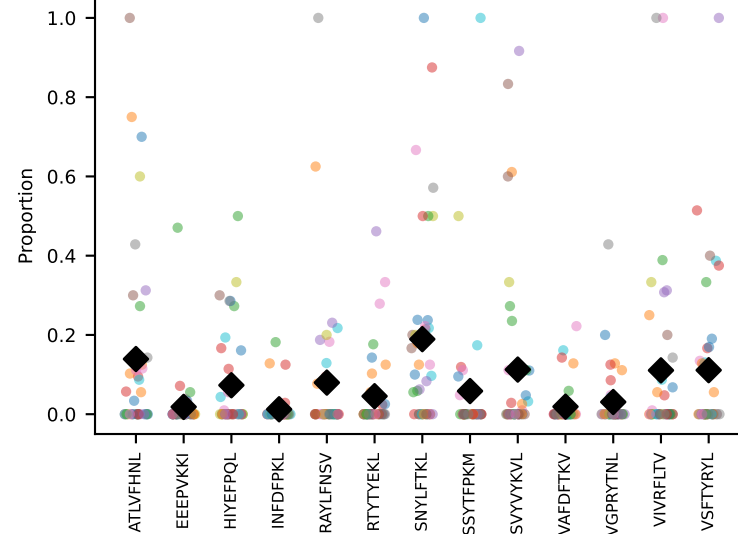
#84 AV17-CALEGSYGNEKITf-AJ48_BV1-CTCSADRVGSDYTF-BJ1-2 coh=0.266, n=38
