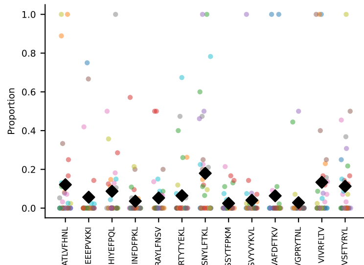
#127 AV12D-3-CALSGPGTGSNRLTF-AJ28_BV29-CASTANTEVFF-BJ1-1 coh=0.205, n=36
