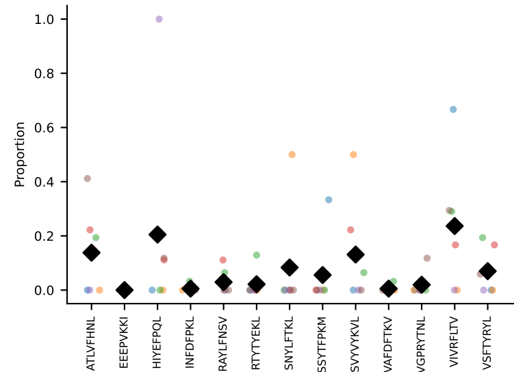
#60 AV7-5-CAVSLTGNTGKLIF-AJ37_BV19-CASSKDRFAEQFF-BJ2-1 coh=0.312, n=6
