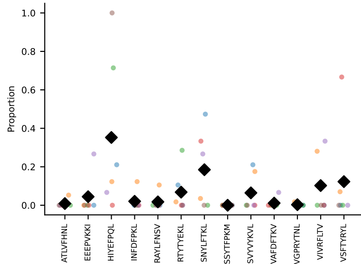
#59 AV16/DV11-CAMREVDTNAYKVIF-AJ30_BV13-1-CASSDGLNSDYTF-BJ1-2 coh=0.313, n=5
