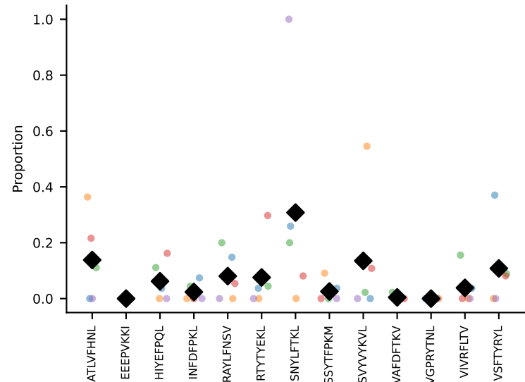
#42 AV13D-1-CAMEDNYAQLTF-AJ26_BV13-1-CASSDKGWVFF-BJ1-1 coh=0.350, n=7
