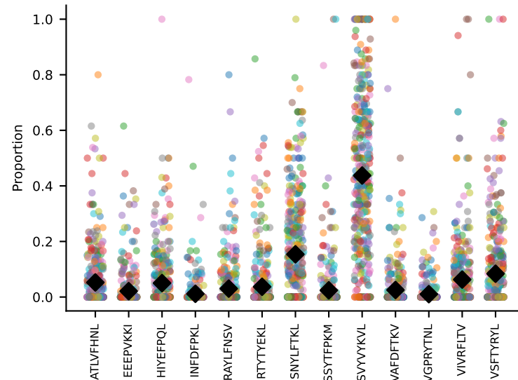
#18 AV8D-2-CATDGQGGRALIF-AJ15_BV29-CASSLGTSGNTLYF-BJ1-3 coh=0.508, n=5
