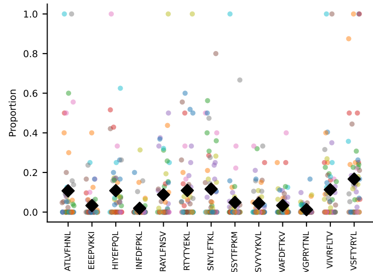
#58 AV7-4-CAASEDYNQGKLIF-AJ23_BV31-CAWSLGHYAEQFF-BJ2-1 coh=0.314, n=62
