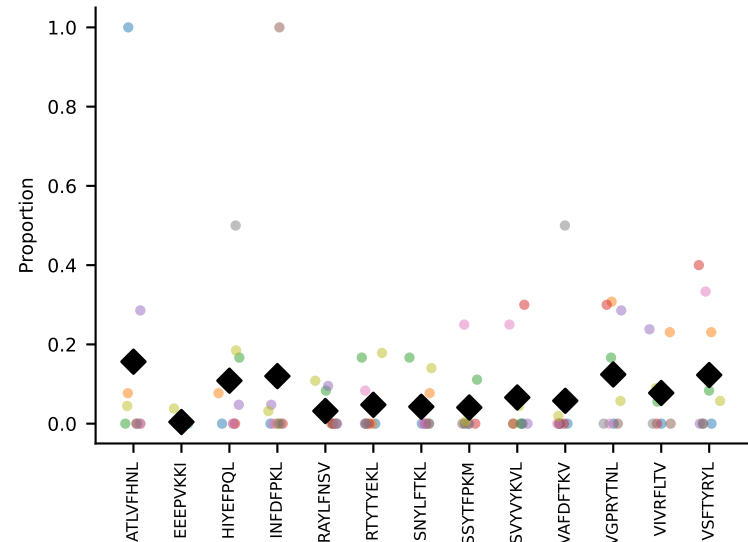
#101 AV8D-2-CATDPSSGQKLVF-AJ16_BV3-CASSLAWGASYEQYF-BJ2-7 coh=0.249, n=6
