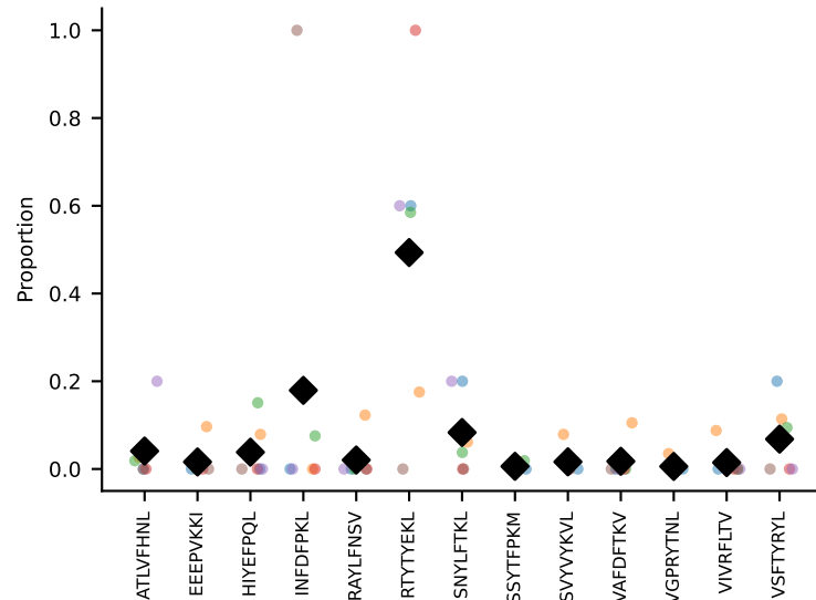
#19 AV14D-3/DV8-CAAGASSGSWQLIF-AJ22_BV31-CAWSPRQGAGTEVFF-BJ1-1 coh=0.497, n=6
