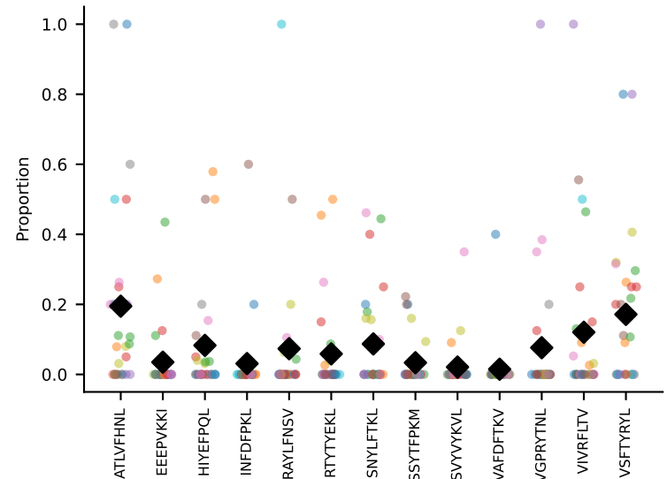
#104 AV17-CALESGSYGNEKITF-AJ48_BV1-CTCSGDRVSYEQYF-BJ2-7 coh=0.240, n=12
