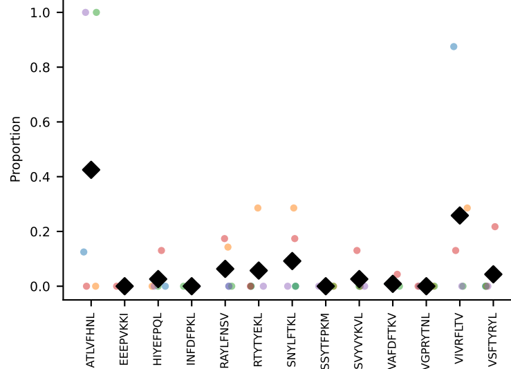
#82 AV13D-4-CAMANNYAQGLTf-AJ26_BV17-CASSSQNTLYF-BJ2-4 coh=0.270, n=5
