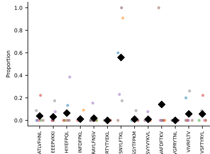
#20 AV13-2-CAPNNNAGAKLTF-AJ39_BV14-CASSDRYEYQYF-BJ2-7 coh=0.491, n=136
