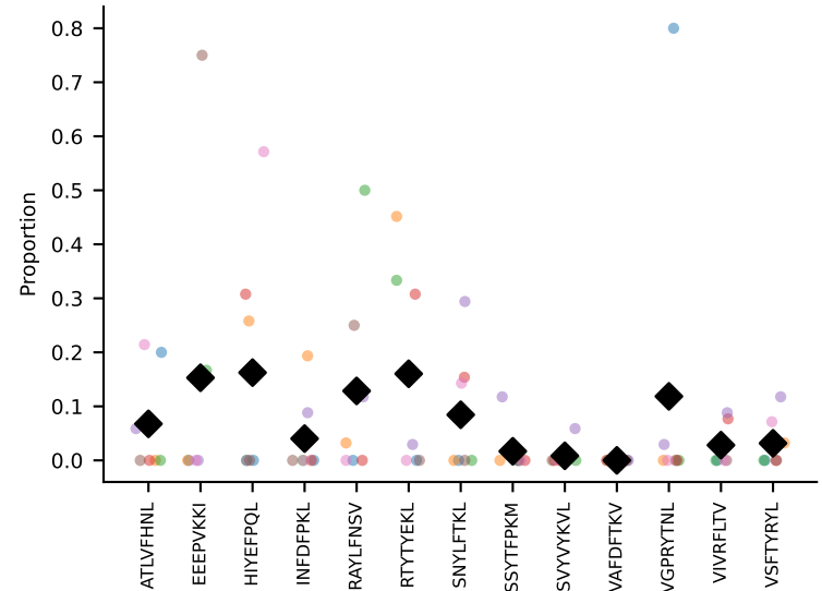
#108 AV14D-3/DV8-CAASETSGSWQLIF-AJ22_BV5-CASSPRLGGDTQYF-BJ1-2 coh=0.234, n=7
