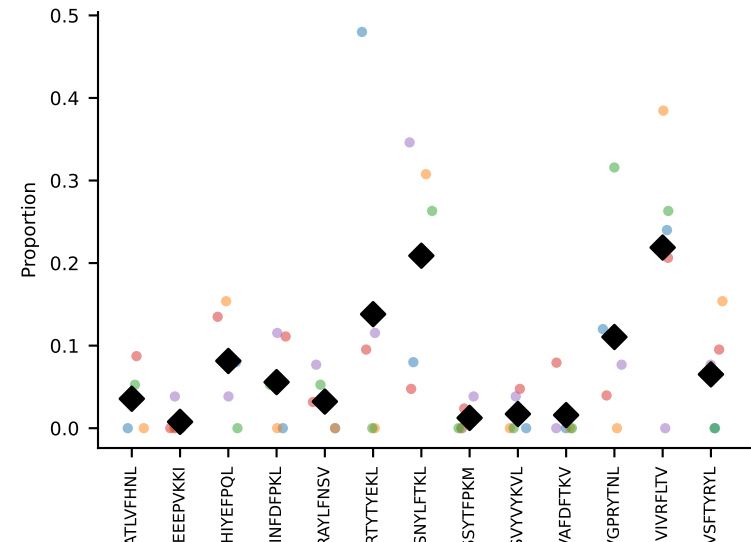
#12 AV10D-CAASRDYNQGLKIF-AJ23_BV3-CASSLGGSQNTLYF-BJ2-4 coh=0.547, n=5
