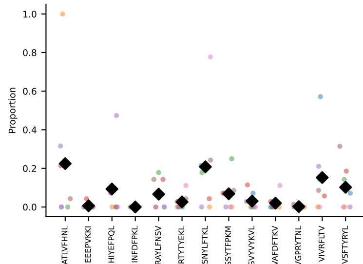
#46 AV10-CAASTDYNQGKLIF-AJ23_BV3-CASSLGTSYEQYF-BJ2-7 coh=0.345, n=9
