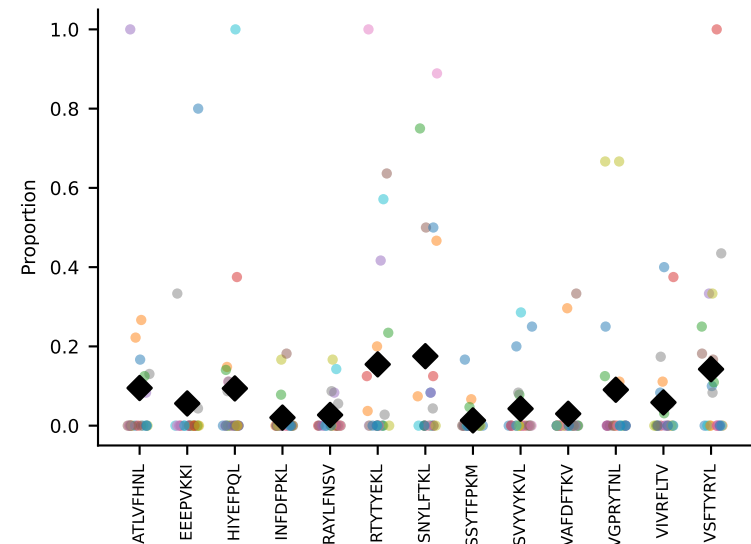
#115 AV4D-4-CAAEPASSGSWQLIF-AJ22_BV16-CASSLELGSDTQYF-BJ2-5 coh=0.225, n=8
