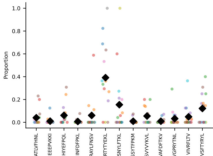
#21 AV14-2-CAASADTGNYKYVF-AJ40_BV13-3-CASSDNNQAPLF-BJ1-5 coh=0.473, n=7
