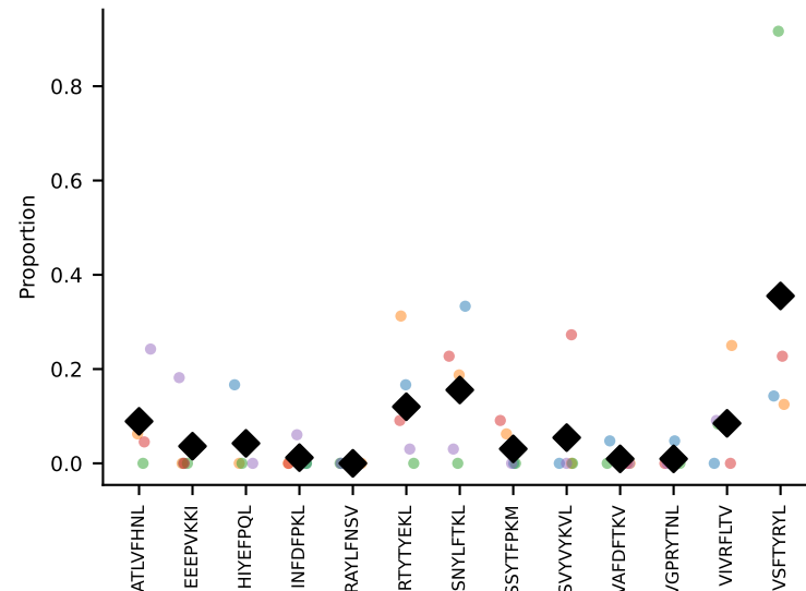
#22 AV16N-CAMREGNSNNRIFF-AJ31_BV13-1-CASRDINTEVFF-BJ1-1 coh=0.453, n=13
