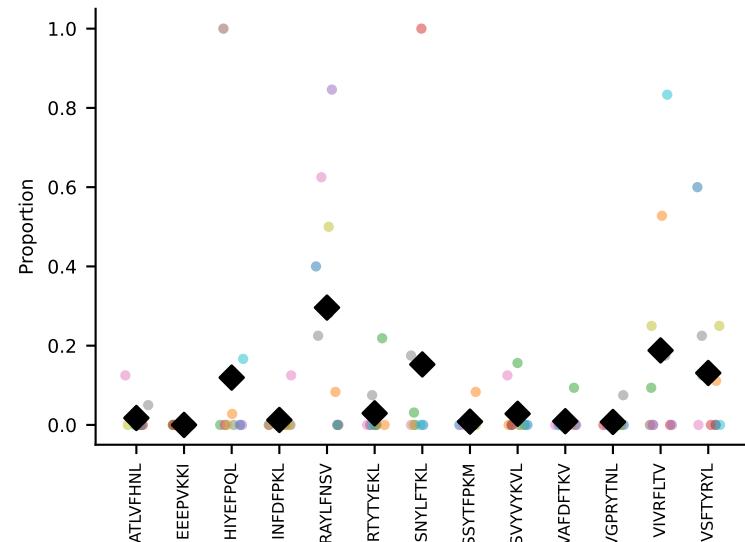
#45 AV9-2-CVFHDTNAYKVIF-AJ30_BV13-2-CASGDALFQDTQYF-BJ2-5 coh=0.345, n=12
