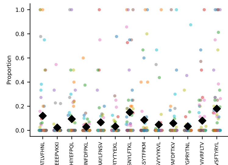
#129 AV6-6-CALGEEEWATGGNNKLTF-AJ56_BV1-CTCSTRGANERLFF-BJ1-4 coh=0.197, n=62
