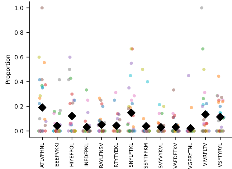
#54 AV12-2-CALSDRGSSSFSLKLVF-AJ50_BV1-CTCSGTNNQAPLF-BJ1-5 coh=0.319, n=6
