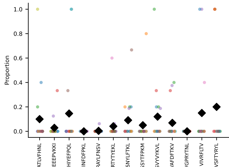
#144 AV2-CIVTDMNYNQGKLIF-AJ23_BV19-CASSPTGPNSDYTF-BJ1-2 coh=0.134, n=16
