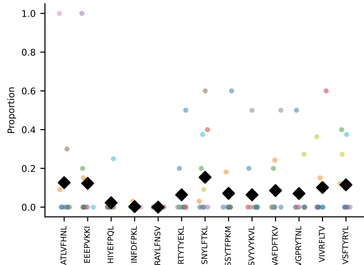
#140 AV14-2-CAATNSAGNKLTF-AJ17_BV26-CASSRTL SGN TLYF-BJ1-3 coh=0.156, n=11
