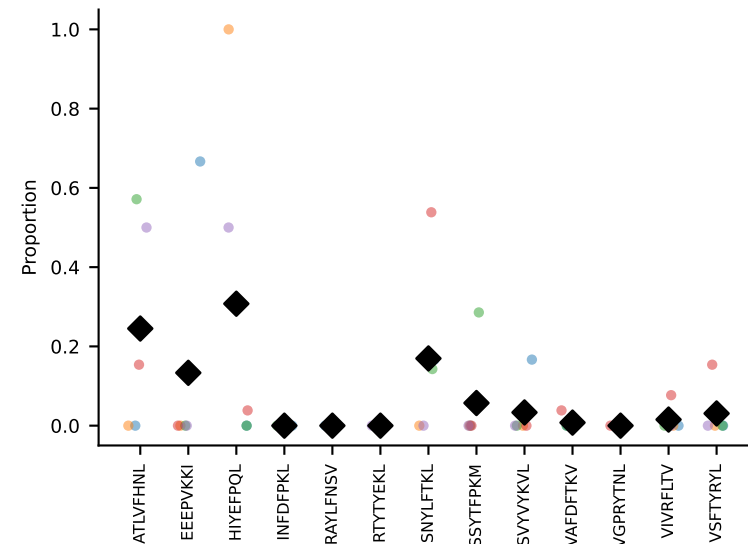
#113 AV16-CAMREDGYQNIFY-AJ49_BV16-CASSLGWGGREQYF-BJ2-7 coh=0.227, n=42
