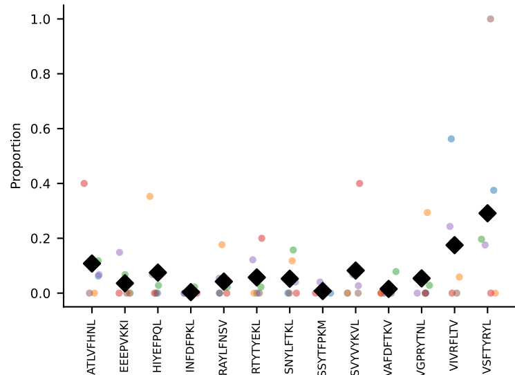
#44 AV7-5-CAVRNAGAKLTF-AJ39_BV1-CTCSATGGGNQAPLF-BJ1-5 coh=0.348, n=19
