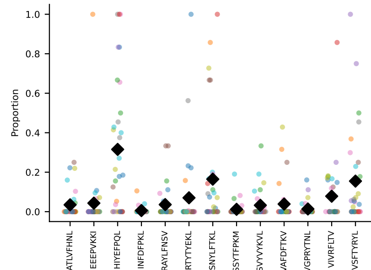
#47 AV7D-3-CAVSMSYAQLTF-AJ26_BV1-CTCSARTGGGYAEQFF-BJ2-1 coh=0.338, n=6
