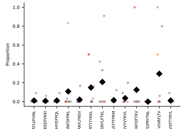
#132 AV6-6-CALGDRNYNOGKLIF-AJ23_BV3-CASSLGGVSNERLFF-BJ1-1 coh=0.190, n=5
