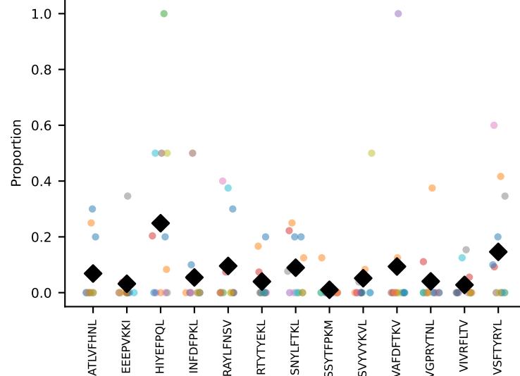
#79 AV14-2-CAASASSGSWQLIF-AJ22_BV31-CAWSLAGSGNTLYF-BJ1-3 coh=0.271, n=23
