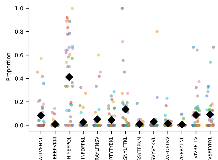
#24 AV21/DV12-CILRVAWNNNAPRF-AJ43_BV2-CASSQEQGYAEQFF-BJ2-7 coh=0.446, n=42
