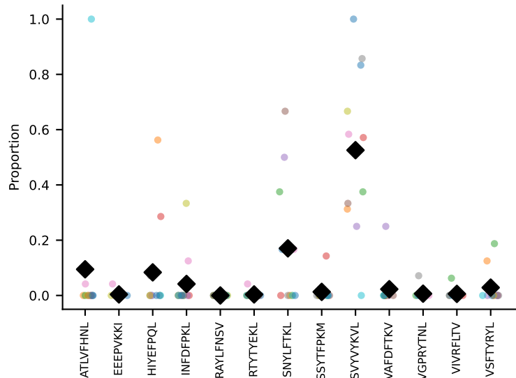
#17 AV1-CAVRPNNNNAPRF-AJ43_BV13-2-CASGARTYNYAEQFF-BJ2-1 coh=0.516, n=16
