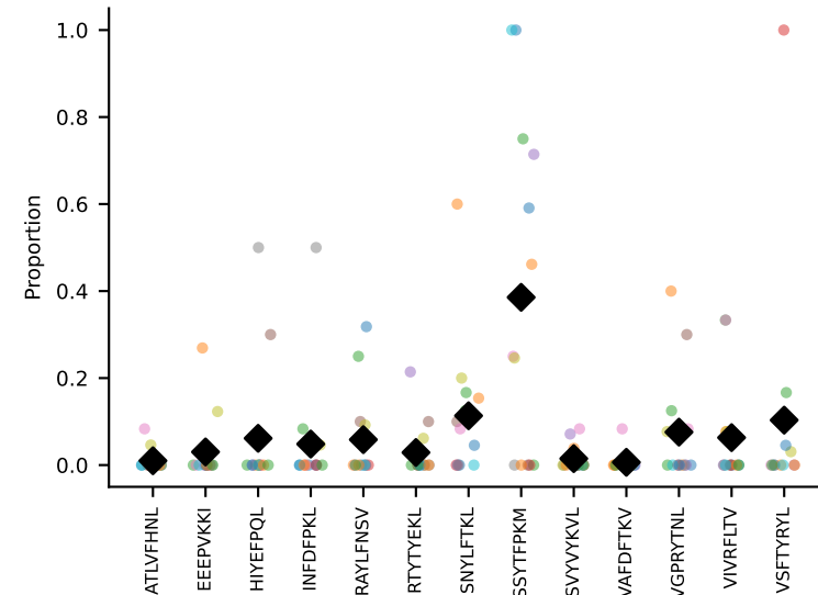
#43 AV13-1-CALERSNNRIFF-AJ31_BV2-CASSQDRRGDEQYF-BJ2-7 coh=0.349, n=31
