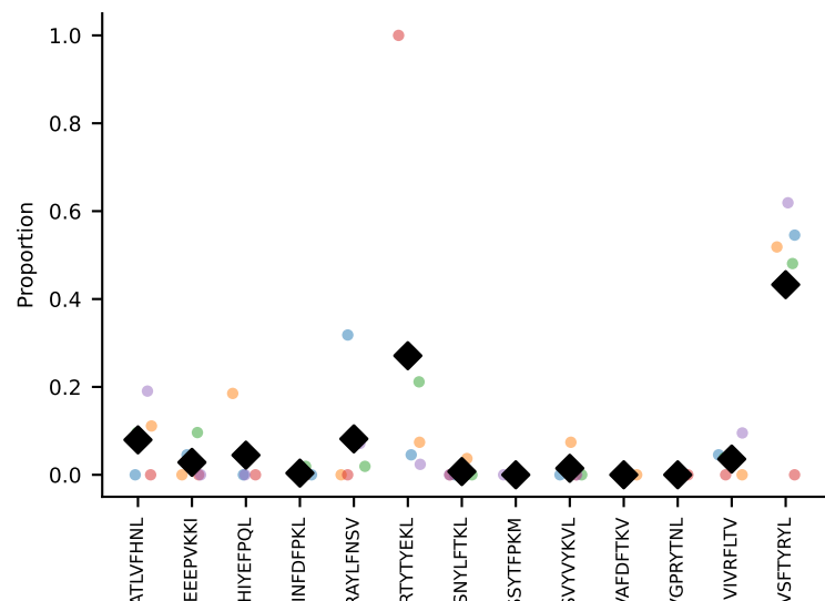
#11 AV3-3-CAVSMDNNA PRF-AJ43_BV1-CTCSAVGGDTQYF-BJ2-5 coh=0.582, n=5
