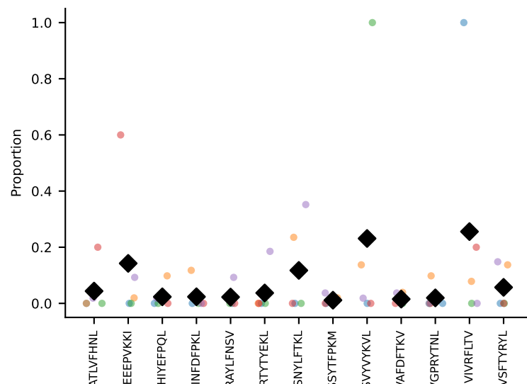
#131 AV13-2-CAIDPNTNKVVF-AJ34_BV31-CAWSLLGSQNTLYF-BJ2-4 coh=0.193, n=5
