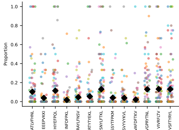
#103 AV16N-CAMREGNNAGAKLTF-AJ39_BV16-CASSSGQKNTEVFF-BJ1-1 coh=0.244, n=83
