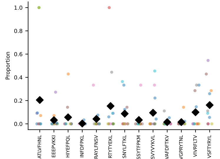
#105 AV7-4-CAASERGASSSFskLVF-AJ50_BV1-CTCSATNNQAPLF-BJ1-5 coh=0.238, n=11
