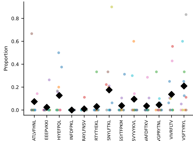
#106 AV5-4-CAASSNTNKVVF-AJ34_BV13-1-CASSATGDSYTF-BJ1-2 coh=0.236, n=5
