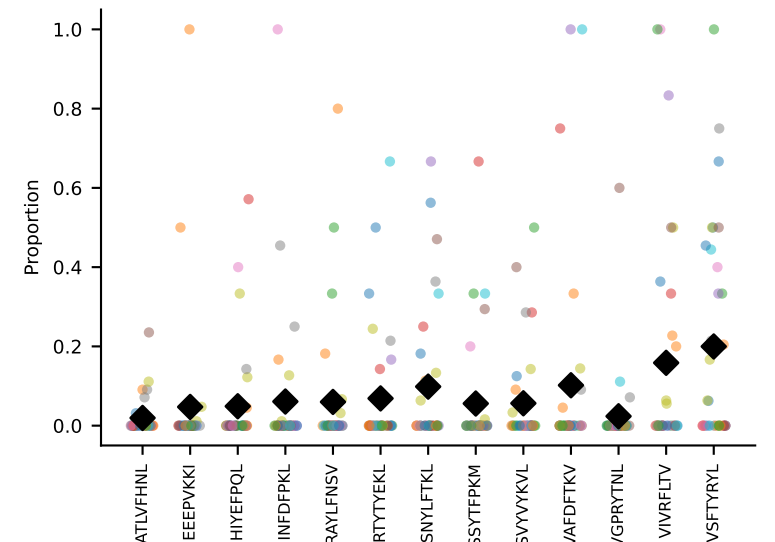
#127 AV12D-3-CALSGPGTGSNRLTF-AJ28_BV29-CASTANTEVFF-BJ1-1 coh=0.205, n=36
