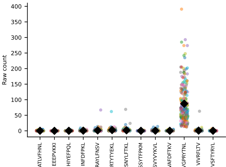
#81 AV9-4-CAVSMDYANKMIF-AJ47_BV3-CASSSGPNYEQYF-BJ2-7 coh=0.980, n=227
