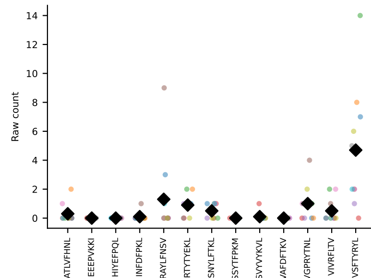
#311 AV16N-CAMREEAGNTGKLIF-AJ37_BV20-CGARDWGGYEQYF-BJ2-7 coh=0.550, n=25
