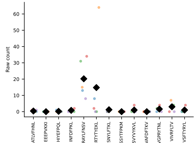
#281 AV16-CAMREANYGNEKITF-AJ48_BV1-CTCSADRVQNTLYF-BJ2-4 coh=0.685, n=5
