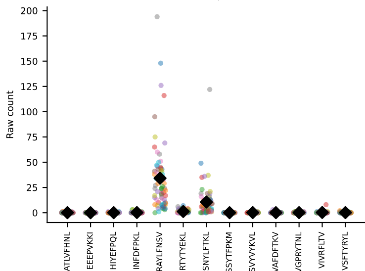
#204 AV9-2-CVLNTGYQNFYF-AJ49_BV13-1-CASSDPGREQYF-BJ2-7 coh=0.895, n=68
