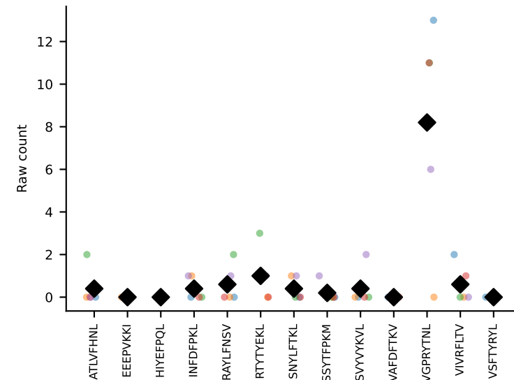
#308 AV12-2-CALSLSSGSWQLIF-AJ22_BV13-1-CASSDQGTEVFF-BJ1- coh=0.567, n=9
