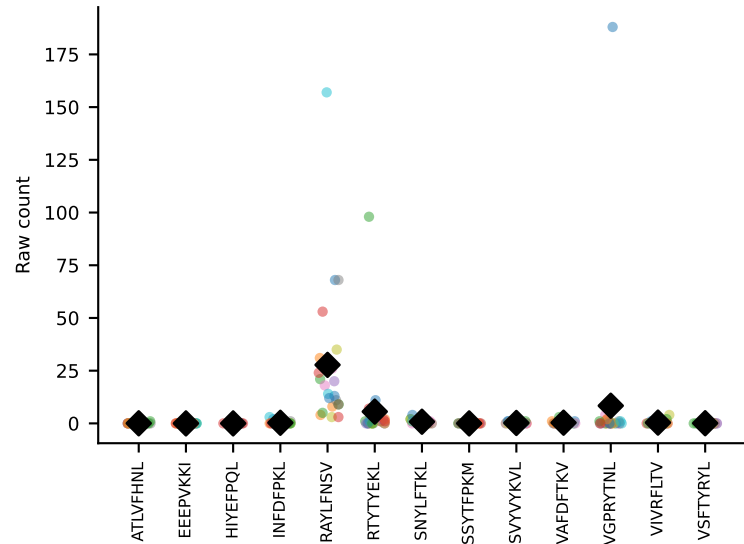
#247 AV7-2-CAASNMGYKLTF-AJ9_BV20-CGARLGGDQYF-BJ2-5 coh=0.799, n=7
