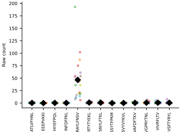
#80 AV16/DV11-CAMRADSNYQLIW-AJ33_BV3-CASSRGQISNERLFF-BJ1-1 coh=0.981, n=24
