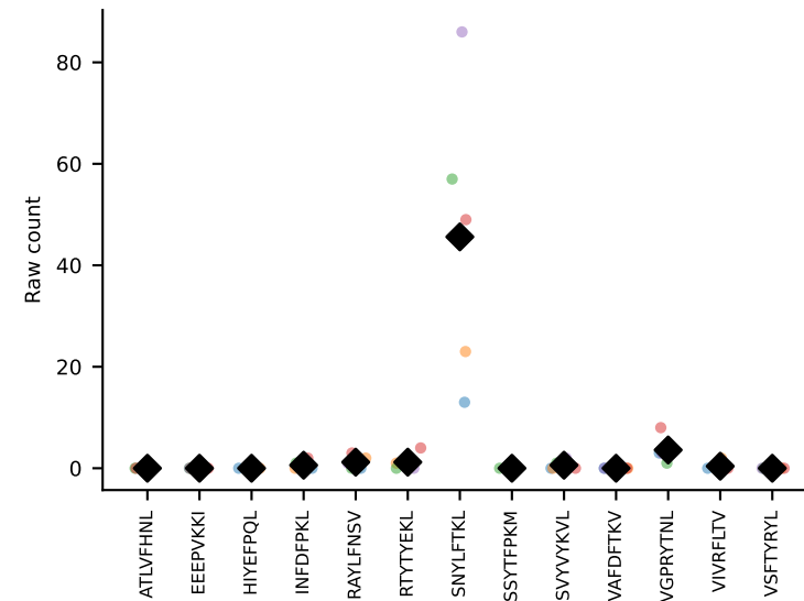
#67 AV10-CAASSGSWQLIF-AJ22_BV1-CTCSADGTGEREQYF-BJ2-7 coh=0.986, n=6
