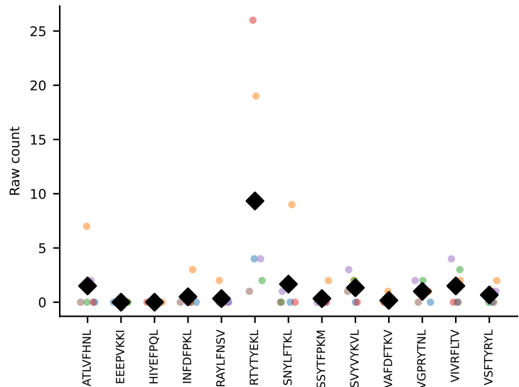
#283 AV14-2-CAASASSGSWQLIF-AJ22_BV31-CAWSLAGSGNTLYF-BJ1-3 coh=0.678, n=6
