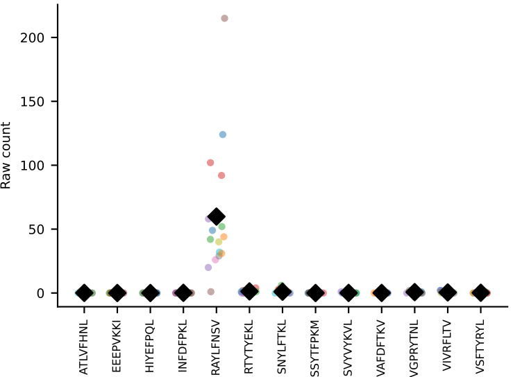
#156 AV4-4/DV10-CAAMDYANKMIF-AJ47_BV2-CASSQDRGYNNQAPLF-BJ1-5 coh=0.943, n=17
