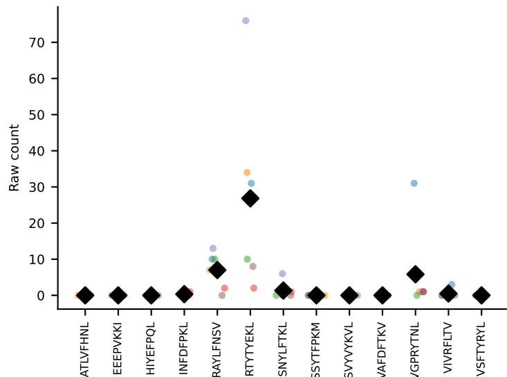
#249 AV6N-6-CALDTNAYKVIF-AJ30_BV4-CASSPDLNTLYF-BJ2-4 coh=0.792, n=6
