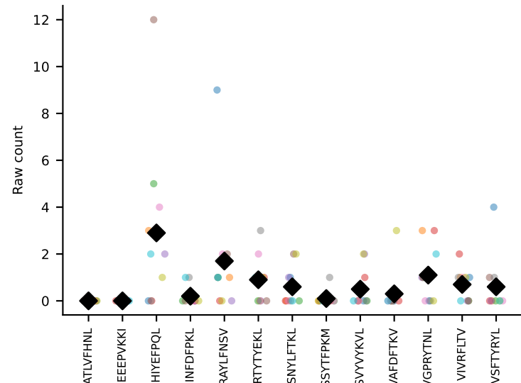
#334 AV16-CAMREGQGGSAKLIF-AJ57_BV1-CTCSADRFYEQYF-BJ2-7 coh=0.417, n=10
