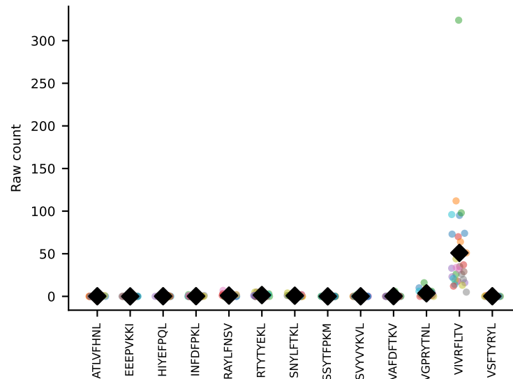
#103 AV9-4-CAVSMDYANKMIF-AJ47_BV3-CASSLGTGYEQYF-BJ2-7 coh=0.969, n=14
