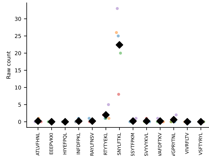
#71 AV10-CAASPNSNNRIFF-AJ31_BV13-3-CASSDRYEQYF-BJ2-7 coh=0.985, n=5
