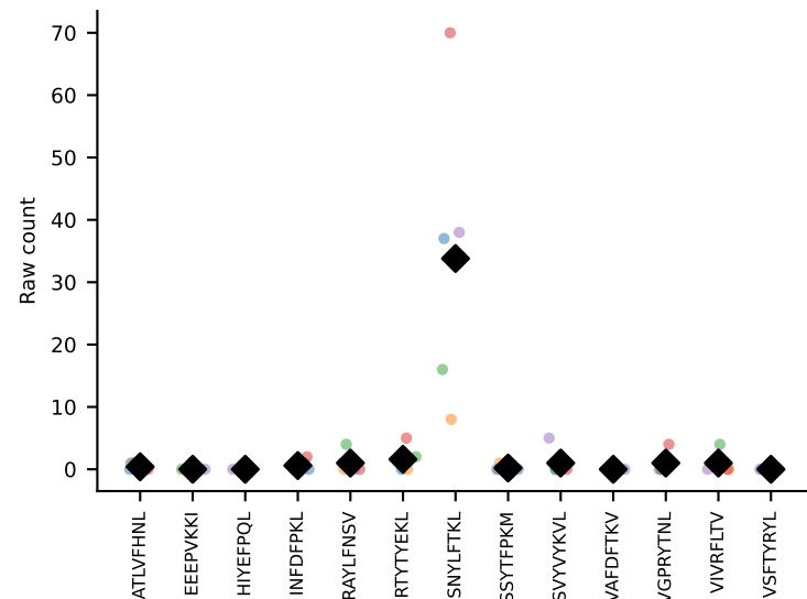
#106 AV12-1-CALSETGNTGKLIF-AJ37_BV13-2-CASGDAGGSYEYF-BJ2-7 coh=0.967, n=5
