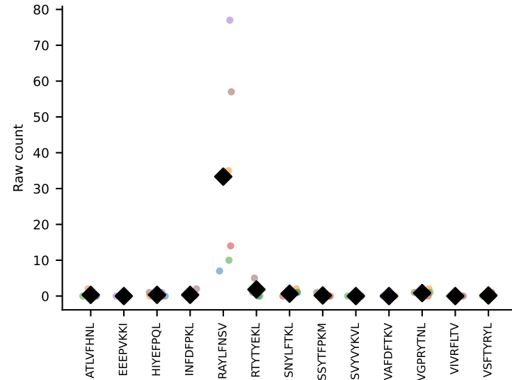
#65 AV6D-7-CALGDGSGGKLT-L-AJ44_BV13-3-CASSDVRTSQNTLYF-BJ2-4 coh=0.987, n=27
