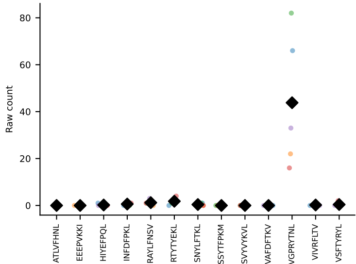
#74 AV6D-7-CALGDDSGYNKLTf-AJ11_BV3-CASSLGTVSYEQYF-BJ2-7 coh=0.985, n=5
