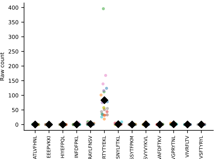
#82 AV13-1-CASPMDSNYQLIW-AJ33_BV31-CAWSLGQDTQYF-BJ2-5 coh=0.980, n=23
