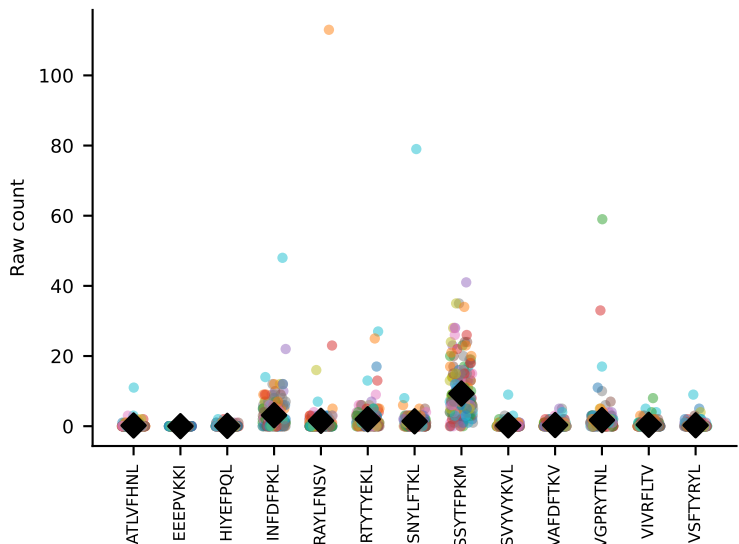
#285 AV14-2-CAATYSNNRLTL-AJ7_BV13-2-CASGGGWNTevFF-BJ1-1 coh=0.675, n=180
