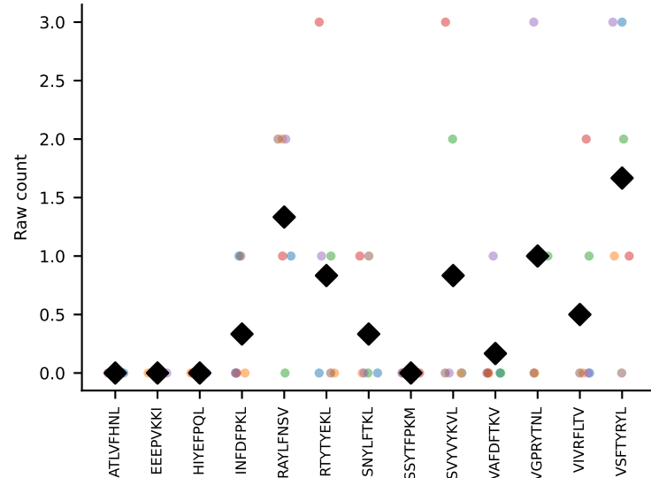
#329 AV3-3-CAVSASNNAGAKLTF-AJ39_BV5-CASSPDRGDERLFF-BJ1-4 coh=0.455, n=55
