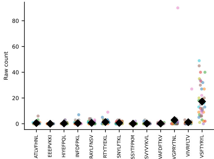
#245 AV13-2-CAIDDTNGKLTF-AJ27_BV12-1-CASSQGNTLYF-BJ2-4 coh=0.808, n=31
