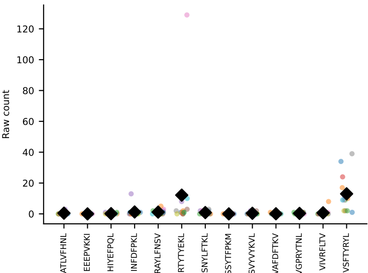
#286 AV13N-1-CAMELNSGTyQRF-AJ13_BV17-CASSPGQGFQDTQYF-BJ2-5 coh=0.675, n=13
