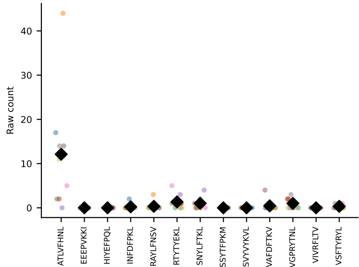
#279 AV8D-2-CATDSQGGRALIF-AJ15_BV3-CASSLGTGGEQYF-BJ2-7 coh=0.688, n=9
