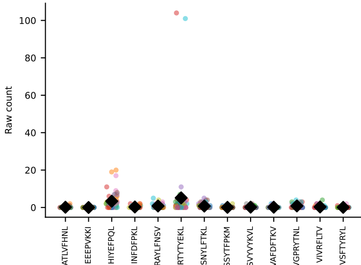
#333 AV9-2-CVLSANTGYQNFYF-AJ49_BV1-CTCSVDRISYEQYF-BJ2-7 coh=0.421, n=5
