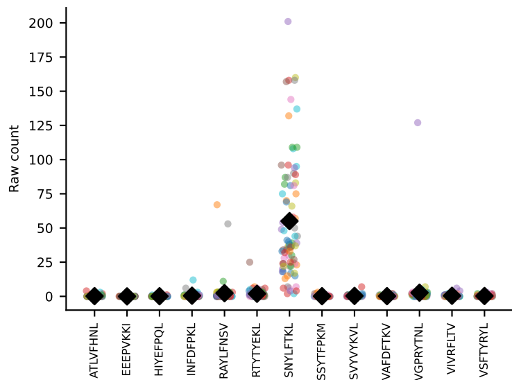
#200 AV8-1-CATEGYQNFYF-AJ49_BV12-1-CASSLGTGGYEQYF-BJ2-7 coh=0.905, n=45
