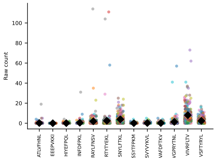
#296 AV6N-6-CALSDRGSGGSNAKLTF-AJ42_BV13-1-CASSDWGDYEQYF-BJ2-2 coh=0.618, n=9
