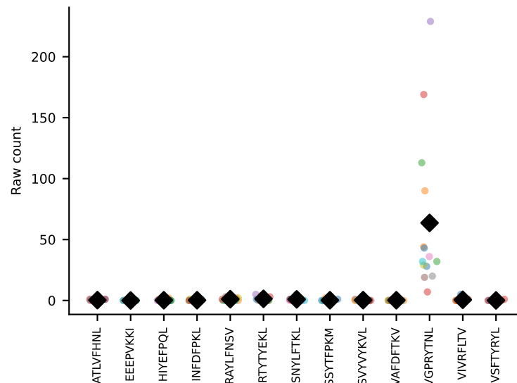
#107 AV9-4-CAVRWDYANKMIF-AJ47_BV3-CASSLSSYEYF-BJ2-7 coh=0.966, n=120
