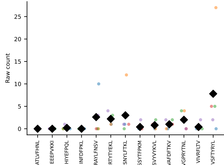
#330 AV13D-2-CAIDPNYNVLYF-AJ21_BV13-3-CASSEKGREQYF-BJ2-7 coh=0.442, n=40
