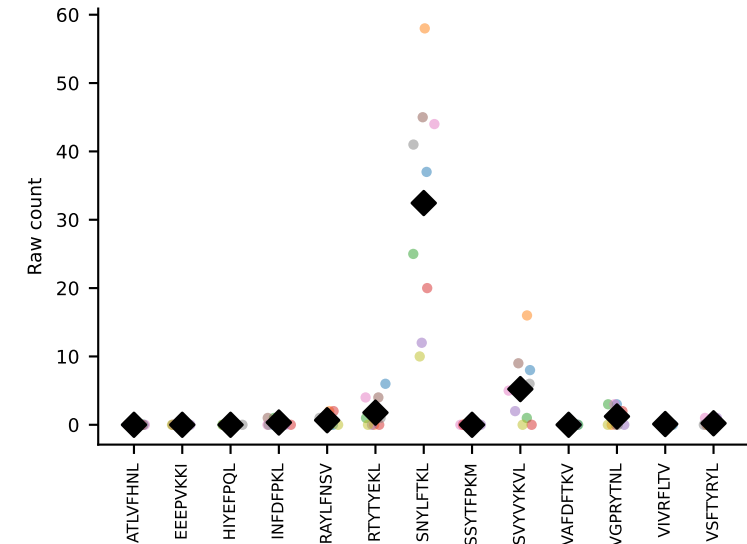
#79 AV16-CAMREGGAGNTGKLIF-AJ37_BV13-2-CASGELYEQYF-BJ2-7 coh=0.982, n=9
