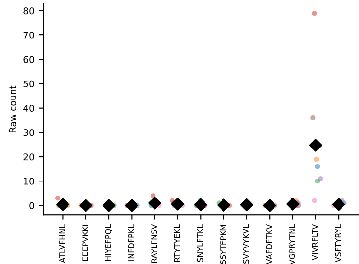
#73 AV5-1-CSASIGSGSWQLIF-AJ22_BV13-1-CASTGGVEQYF-BJ2-7 coh=0.985, n=7
