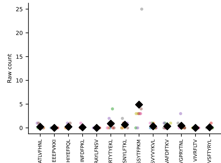
#312 AV16N-CAMRASSGSWQLIF-AJ22_BV1-CTCSASGTGDNSPLYF-BJ1- coh=0.537, n=9
