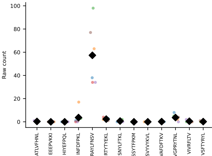
#77 AV9-2-CVLSSTSGGNYKPTF-AJ6_BV1-CTCSAVRVDTEVFF-BJ1-1 coh=0.982, n=6
