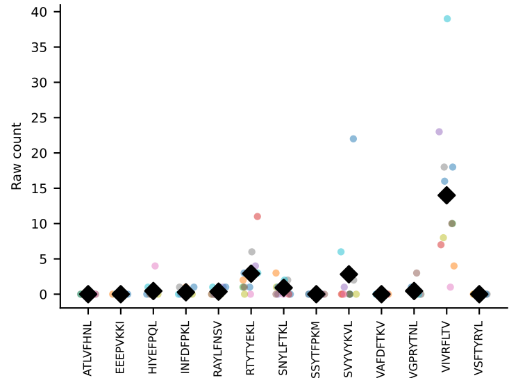
#278 AV10D-CAASWDTNAYKVIF-AJ30_BV13-2-CASGEQTEVFF-BJ1-1 coh=0.696, n=11
