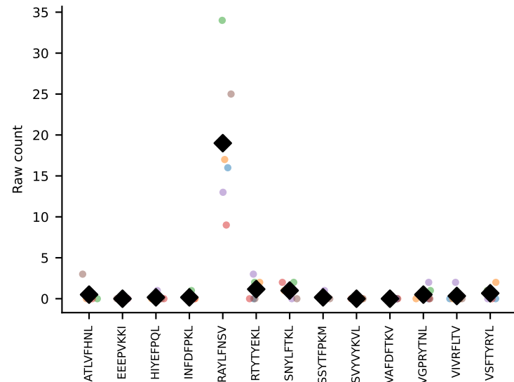
#102 AV6D-7-CALGDDSGYNKLTFF-AJ11_BV3-CASSLGQISYEYF-BJ2-7 coh=0.970, n=31
