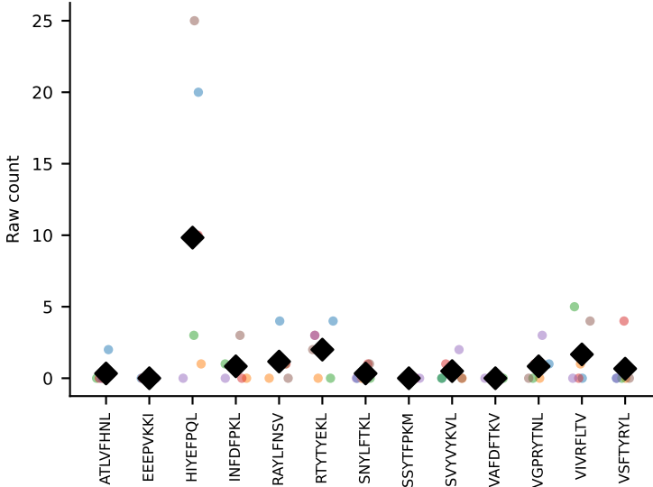
#317 AV14D-1-CAATGANTGKLTIF-AJ52_BV1-CTCSAAWGAEQYF-BJ2-7 coh=0.505, n=19
