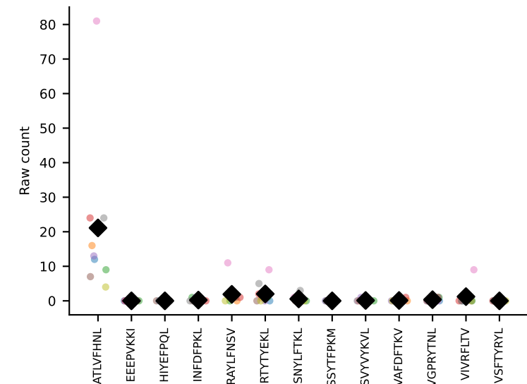
#83 AV7-3-CAVMGGRALIF-AJ15_BV13-1-CASSADWGDAEQFF-BJ2-1 coh=0.979, n=9
