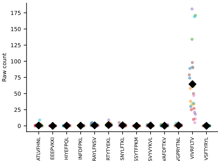
#69 AV5-4-CAARGDYANKMIF-AJ47_BV3-CASSLGVDTQYF-BJ2-5 coh=0.985, n=75
