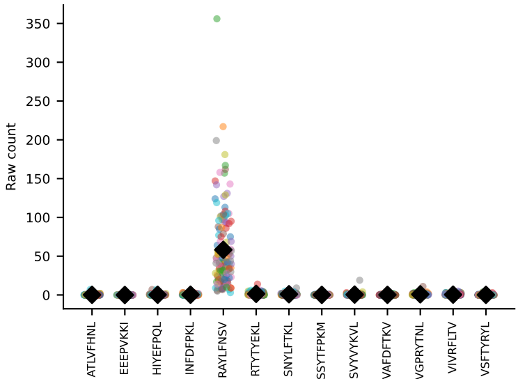
#76 AV16N-CAMREDSNYQLIW-AJ33_BV3-CASSLGQISNERLFF-BJ1-4 coh=0.982, n=138
