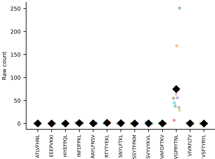
#93 AV9-4-CAVSVDYANKMIF-AJ47_BV3-CASSWGGGYEQYF-BJ2-7 coh=0.973, n=10
