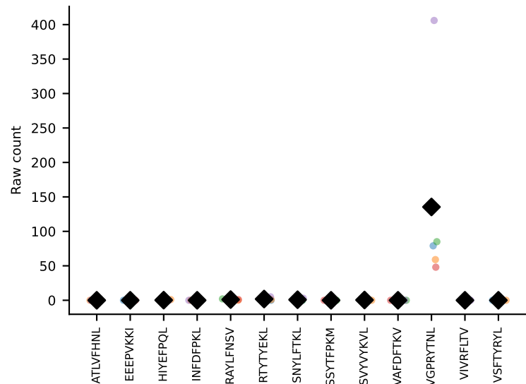
#8 AV9-2-CVLSLNYGSSGNKLIF-AJ32_BV3-CASSPGYYAEQFF-BJ2-1 coh=0.999, n=9
