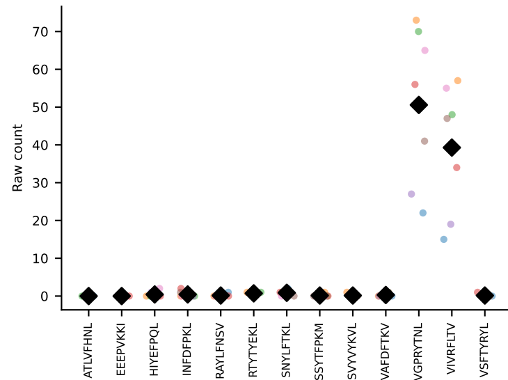
#66 AV5-4-CAASTDYANKMIF-AJ47_BV3-CASSSGTGYEQYF-BJ2-7 coh=0.986, n=74
