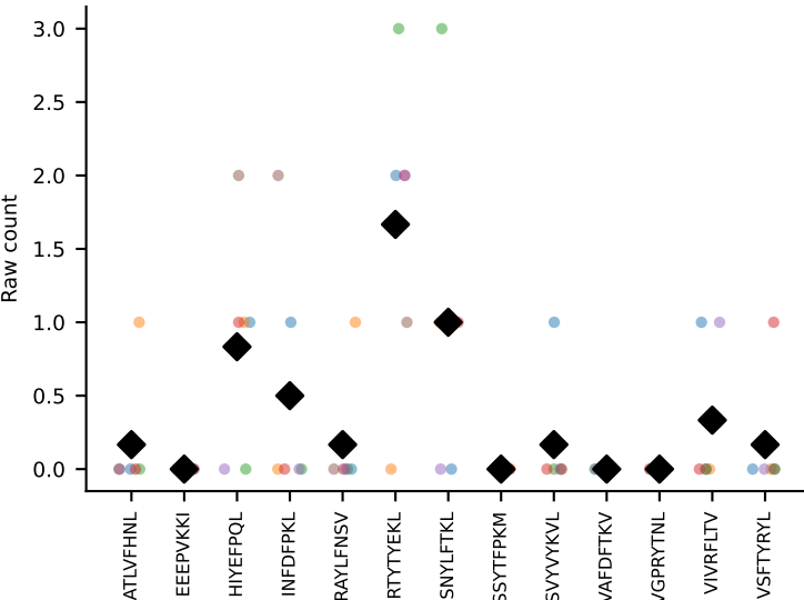
#321 AV10N-CAASRASGSWQLIF-AJ22_BV16-CASSLTGEGNTLYF-BJ1-3 coh=0.497, n=6
