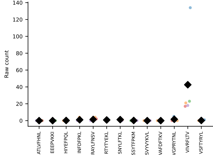
#75 AV6D-7-CALGDASGSWQLIF-AJ22_BV13-1-CASSDGANYAEQFF-BJ2-1 coh=0.984, n=5
