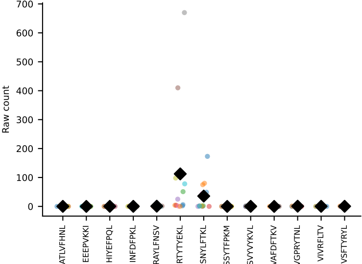
#322 AV16/DV11-CAMREEGGRALIF-AJ15_BV13-1-CASKDTYPEQYF-BJ2-7 coh=0.496, n=12
