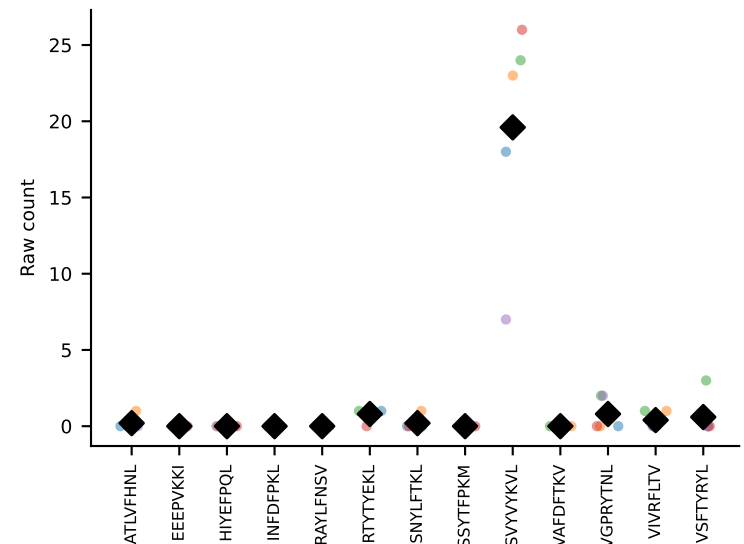
#84 AV9-2-CVLSLGNSNNRIFF-AJ31_BV13-2-CASGDAGGQDTQYF-BJ2-1 coh=0.979, n=5
