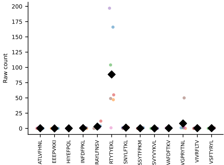
#277 AV7-3-CAVSGGNYKPTF-AJ6_BV31-CAWSYRGETLYF-BJ2-3 coh=0.711, n=7
