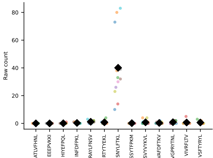
#78 AV16-CAMREGGAGNTGKLIF-AJ37_BV13-2-CASGDNYEQYF-BJ2-7 coh=0.982, n=13
