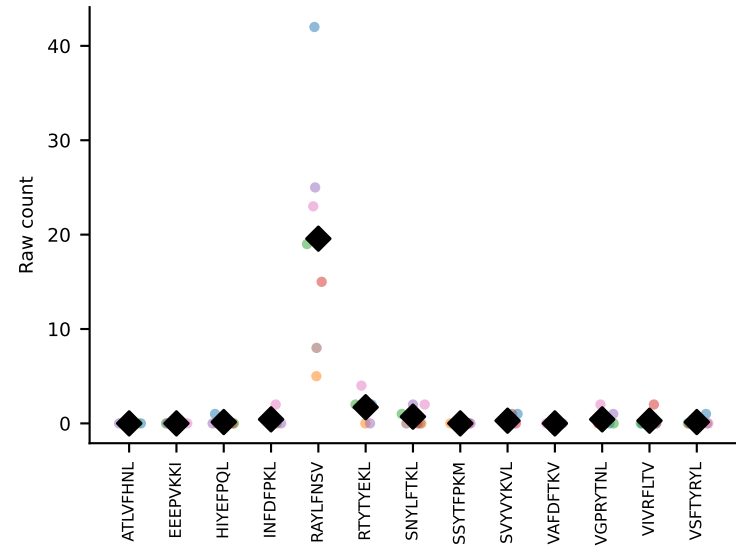
#89 AV10-CAASMDYANKMIF-AJ47_BV1-CTCSVTPNSDYTF-BJ1-2 coh=0.977, n=6
