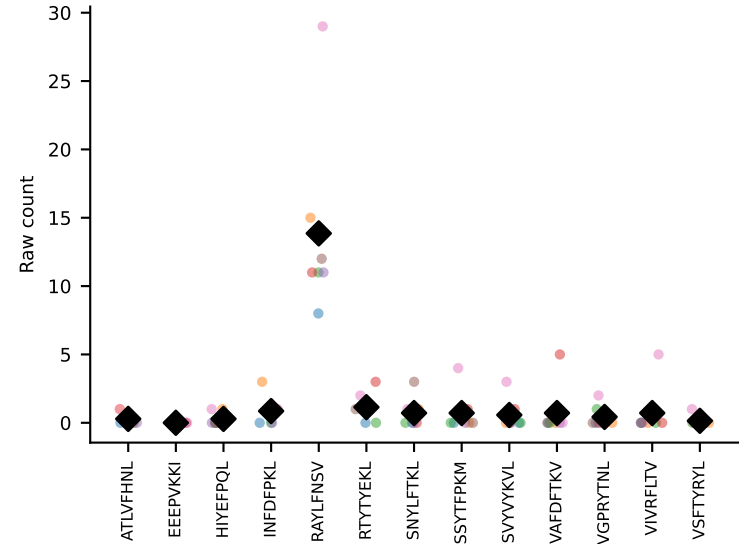
#154 AV16/DV11-CAMREGGGYKVVF-AJ12_BV13-2-CASGDIQAPLF-BJ1-5 coh=0.943, n=17 #155 AV12-3-CALSDLDYGNEKITF-AJ48_BV16-CASSGLGGLSYEQYF-BJ2-7 coh=0.943, n=13
