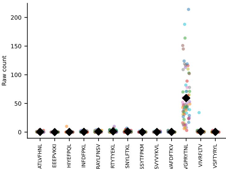
#70 AV16N-CAMREDSGYNKLT-AJ11_BV13-1-CASSDAGAEVFF-BJ1-1 coh=0.985, n=5
