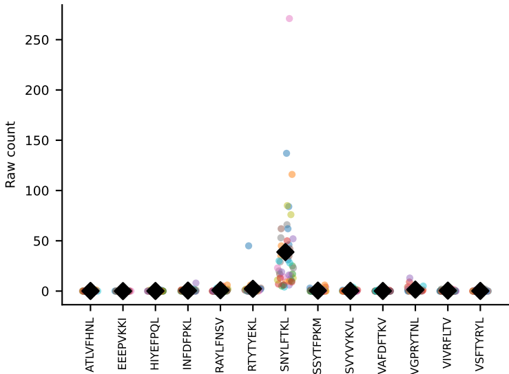
#150 AV13D-1-CAMEDSGTYQRF-AJ13_BV12-2-CASSLGQGAETLYF-BJ2-3 coh=0.944, n=6 #151 AV16/DV11-CAMRDSGGSNAKLTF-AJ42_BV1-CTCSADRVAETLYF-BJ2-3 coh=0.944, n=7
