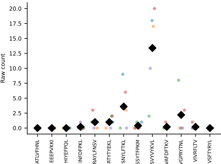
#284 AV16-CAMREANTGYQNfYF-AJ49_BV13-2-CASGTGGENTLYF-BJ2-2 coh=0.676, n=5
