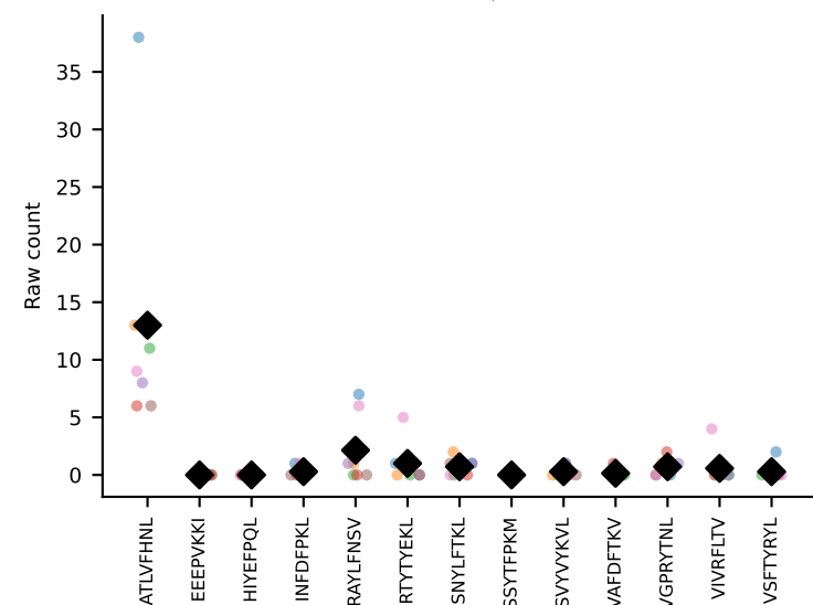
#202 AV13N-4-CAMEHGTGGYKVV F-AJ12_BV5-CASSQAQGEVFF-BJ1-1 coh=0.899, n=7
