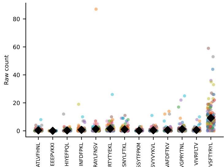
#287 AV6-5-CALSDHAGYQNfYF-AJ49_BV13-2-CASGARTGENYAEQFF-BJ2-1 coh=0.669, n=152
