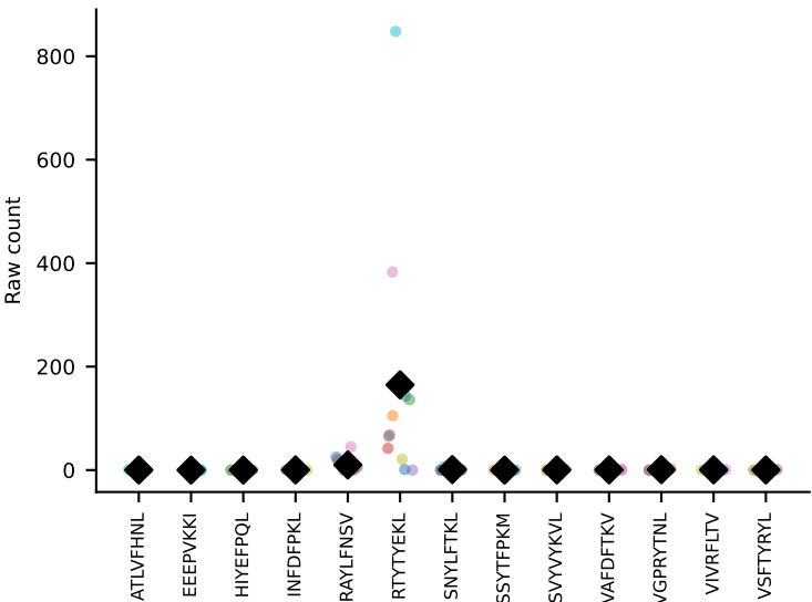
#282 AV16/DV11-CAMREPYQGGRALIF-AJ15_BV13-2-CASGDQGASGNTLYF-BJ1-1 coh=0.680, n=11
