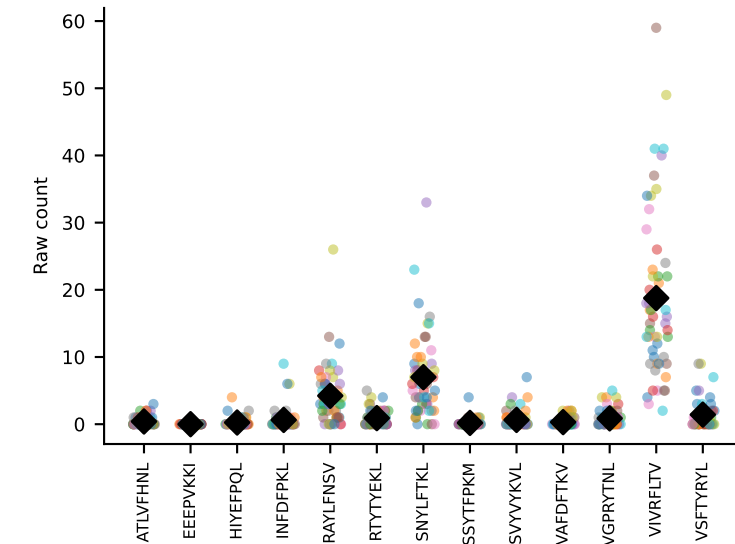
#215 AV6-6-CALGDQGTGSKLSF-AJ58_BV17-CASSRGQGYTGQLYF-BJ2-2 coh=0.876, n=52
