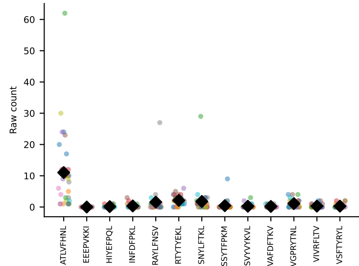
#280 AV16N-CAMREDTNTGKLTf-AJ27_BV16-CASSLDNYAEQFF-BJ2-1 coh=0.687, n=32
