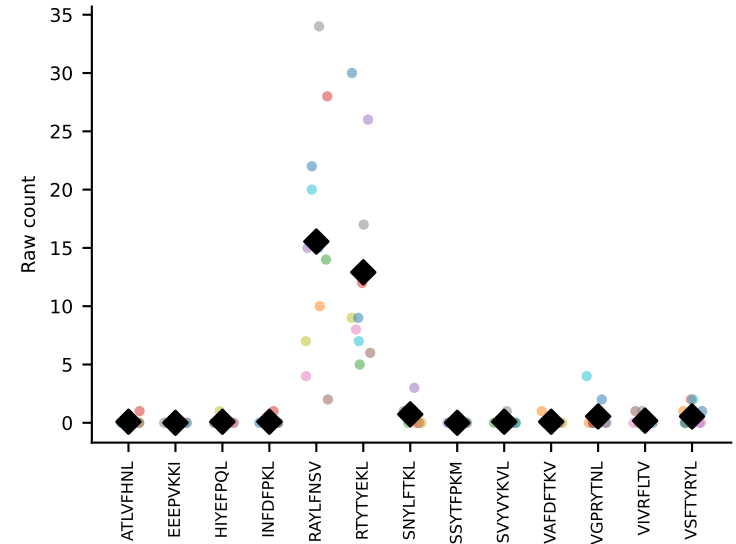
#216 AV7D-3-CAVTGNKYKVF-AJ40_BV13-2-CASGDQGASGNTLYF-BJ1 coh=0.875, n=16
