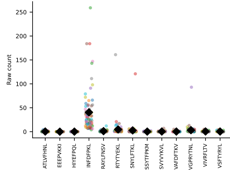
#211 AV10N-CAASLDSNYQLIW-AJ33_BV19-CASSSSGTTNQAPLF-BJ1-5 coh=0.884, n=6
