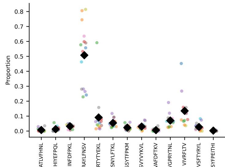
#213 AV5D-4-CAASDMGYKLTF-AJ9_BV13-2-CASGDALGGFSYEQYF-BJ2-7 coh=0.817, n=13
