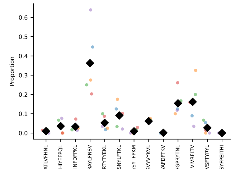
#215 AV16/DV11-CAMREGDTGYQNIFYF-AJ49_BV1-CTCSADRAQDTQYF-BJ2-5 coh=0.810, n=5
