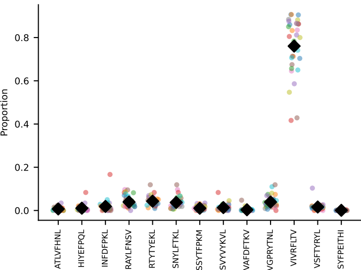
#101 AV16D/DV11-CAMREGSSGSWQLIF-AJ22_BV13-1-CASSDVGDEQYF-BJ2-7# coh=0.979, n=6
