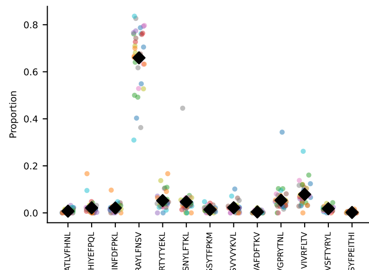
#153 AV13-1-CAMPDSSGSWQLIF-AJ22_BV4-CASSYSGEQYF-BJ2-7 coh=0.936, n=6
