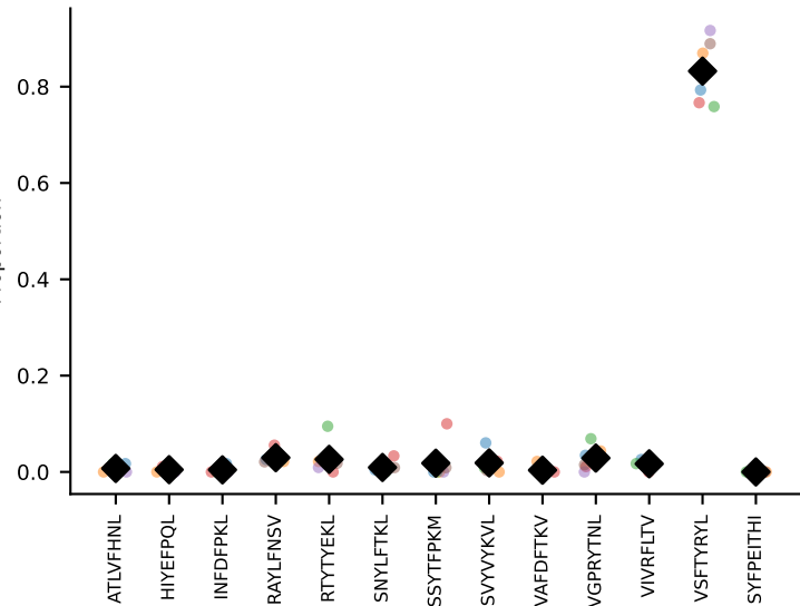
#55 AV16D/DV11-CAMREASSGSWLIF-AJ22_BV13-2-CASGDP TGQEYF-BJ2-7 coh=0.992, n=34
