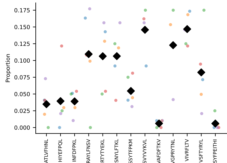
#209 AV8D-2-CATVGNRIFF-AJ31_BV1-CTCSAVRISNERLFF-BJ1-4 coh=0.821, n=15
