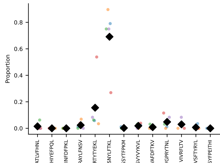
#216 AV6-4-CALVPDYANKMIF-AJ47_BV13-3-CASSDRGQVFF-BJ1-1 coh=0.798, n=5
