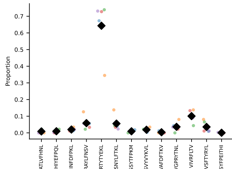
#150 AV10D-CAAVNNYAQGLTF-AJ26_BV13-1-CASSGTGNTEVFF-BJ1-1 coh=0.940, n=12
