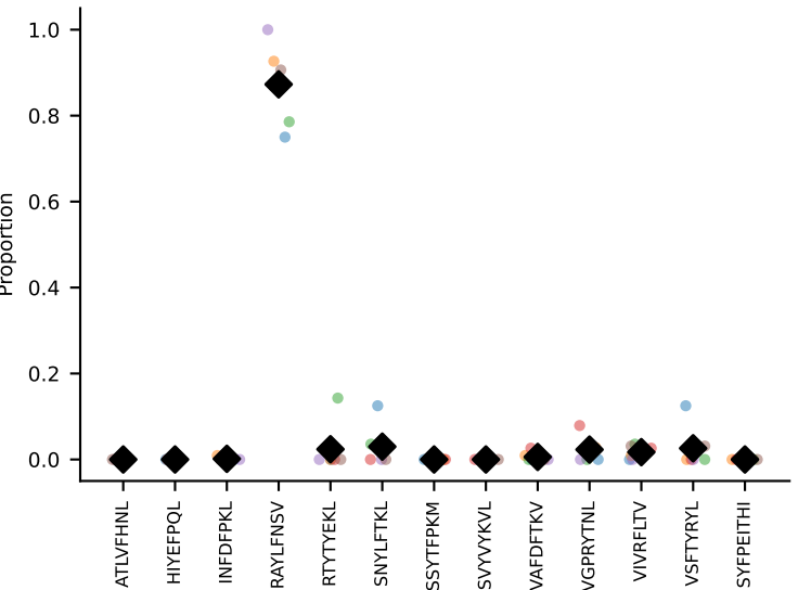
#92 AV5-1-CSASMDYANKMIF-AJ47_BV3-CASSYGTNNQAPLF-BJ1-5 coh=0.982, n=38
