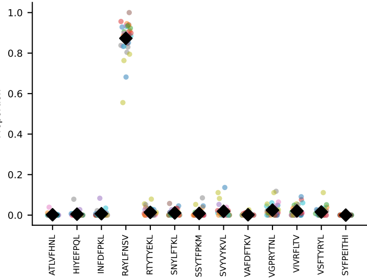
#59 AV19-CAAGVTGYQNIFYF-AJ49_BV29-CASSLRTGREYF-BJ2-7 coh=0.991, n=16
