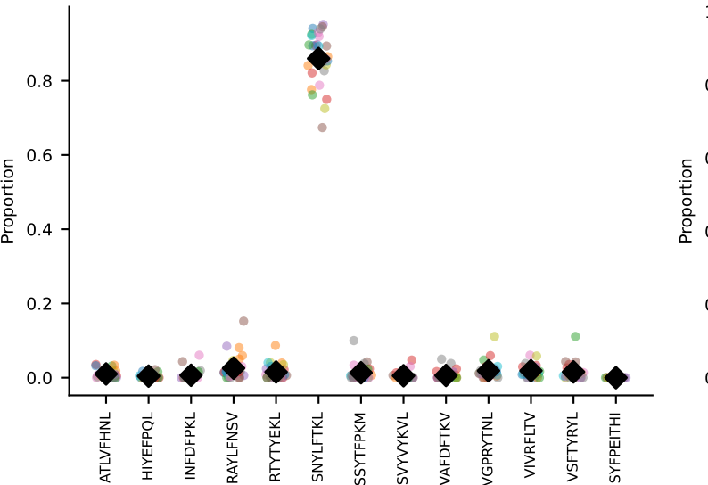
#53 AV9-3-CAVSSDYANKMIF-AJ47_BV3-CASSSGTGGYEYF-BJ2-7 coh=0.992, n=11
