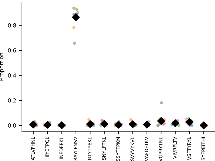
#68 AV12-2-CALRASNTDKVVF-AJ34*p03_BV1-CTCSADWDEQYF-BJ2-1 coh=0.989, n=5
