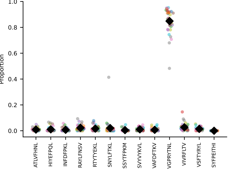
#96 AV12-2-CALSDLRTGGADRLTF-AJ45_BV13-1-CASSDVGAEQFF-BJ2-2 coh=0.981, n=7
