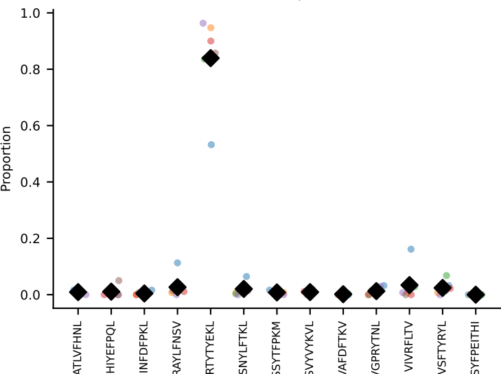
#105 AV16/DV11-CAMRESTGANTGKLTf-AJ52_BV13-3-CASSPGTVYAEQFF-BJ2-1# coh=0.977, n=6
