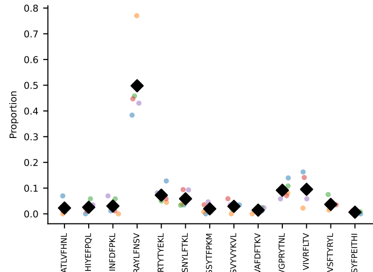
#149 AV1-CAVRDSYAQGLTF-AJ26_BV13-1-CASSDDRVTNTLYF-BJ1-3 coh=0.941, n=33
