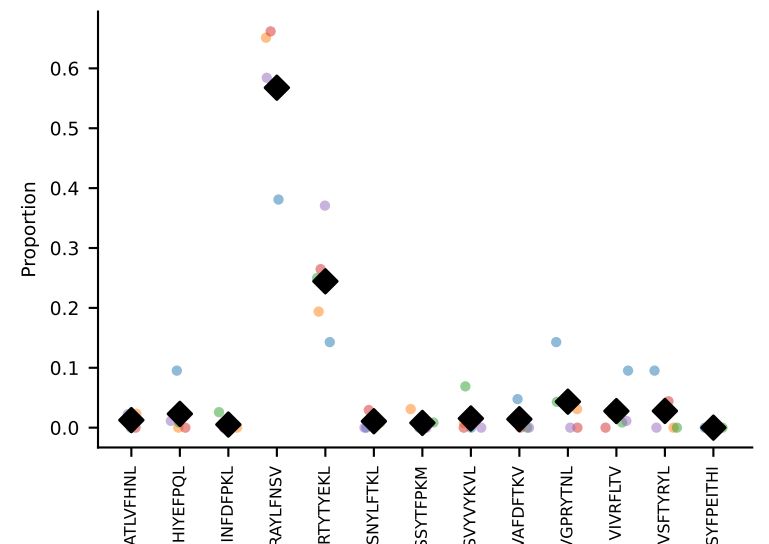
#151 AV6-6-CALGDTSGGSNYKLTF-AJ53_BV1-CTCSAVRANTGQLYF-BJ2-2 coh=0.938, n=6
