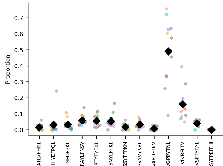
#212 AV16D/DV11-CAMRESSNTDKVVF-AJ34*p03_BV13-1-CASSDAPGREQYF-BJ2-7 coh=0.819, n=7
