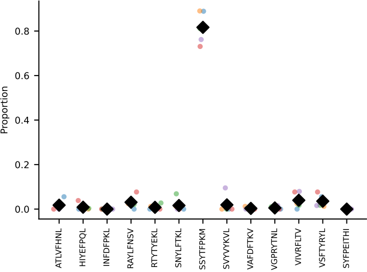
#69 AV6-6-CALGDHTGYQNfYF-AJ49_BV13-3-CASSENRVNTEVFF-BJ1-1 coh=0.989, n=5
