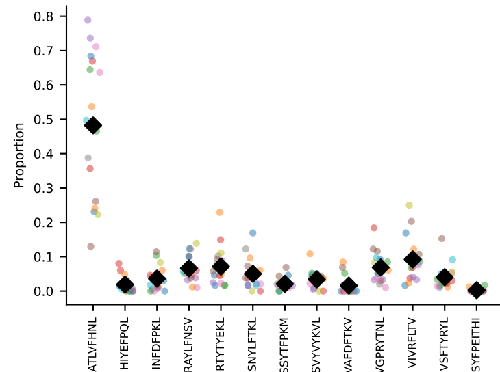
#210 AV14D-1-CAASKDTGNYKYVF-AJ40_BV13-3-CASSDSNTEVFF-BJ1-1 coh=0.820, n=5
