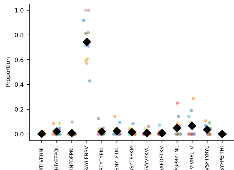
#154 AV7D-4-CAASTGYQNIFYF-AJ49_BV13-3-CASSRDRVNSPLYF-BJ1-6 coh=0.935, n=7
