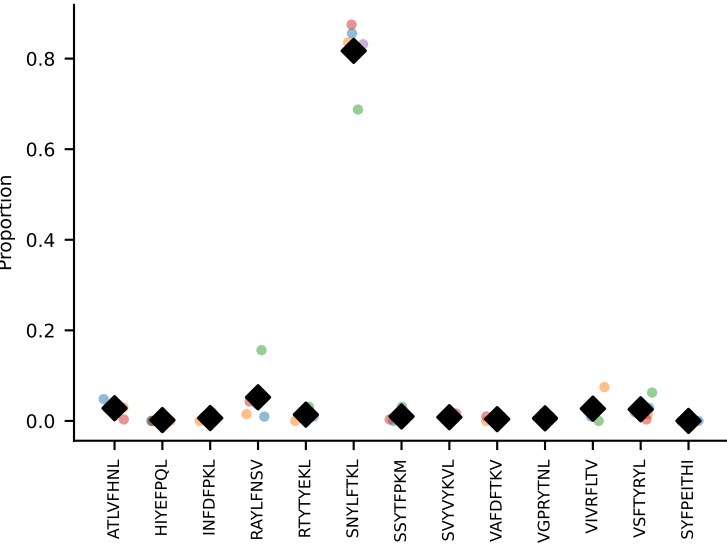
#72 AV16D/DV11-CAMREAGYKVVf-AJ12_BV13-2-CASGDAGGKAIEVFF-BJ1-1 coh=0.988, n=10
