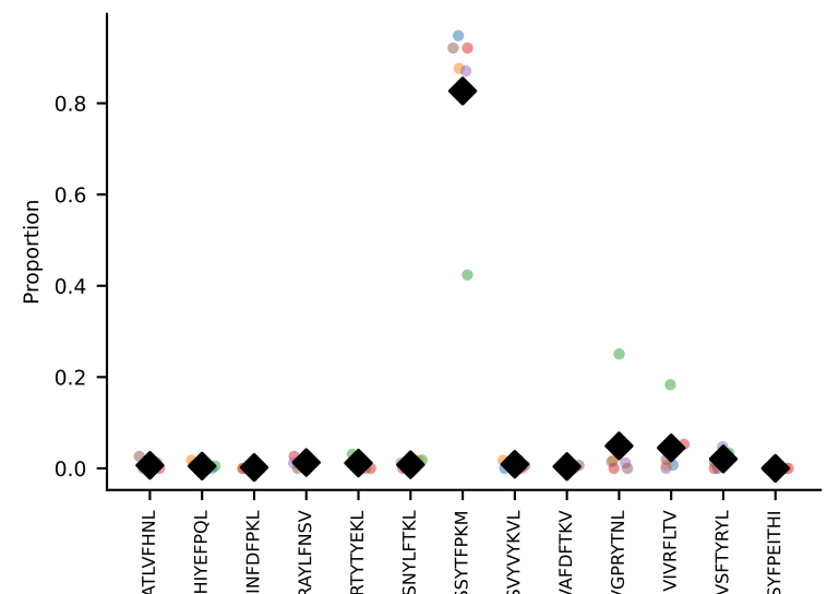
#156 AV3-3-CAVSAGQGGRALIF-AJ15_BV13-1-CASSDTGGYEYF-BJ2-1 coh=0.933, n=24
