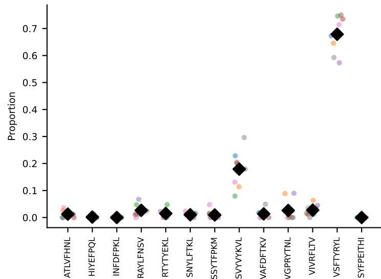
#104 AV14D-2-CAASPDGTGNYKYVF-AJ40_BV13-3-CASSDNGNNQAPLF-BJ2-5 coh=0.977, n=9
