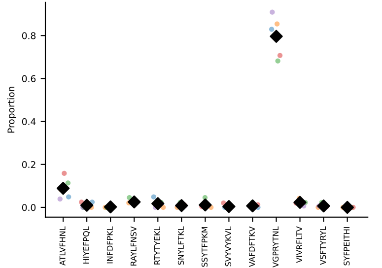
#60 AV7D-5-CAVSRFNYAQGLTF-AJ26_BV5-CASSQDAYSGNTLYF-BJ1-3 coh=0.991, n=5
