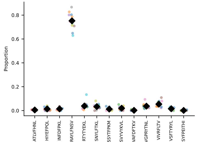
#56 AV8-2-CATDATRMDYANKMIF-AJ47_BV3-CASSLARDYEYF-BJ2-7 coh=0.991, n=5
