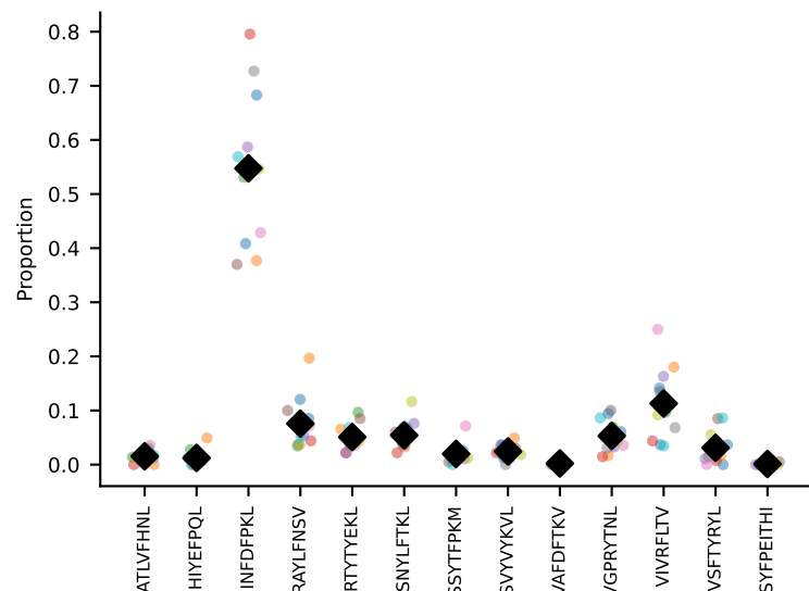
#151 AV6-6-CALGDTSGGSNYKLTF-AJ53_BV1-CTCSAVRANTGQLYF-BJ2-2 coh=0.938, n=6
