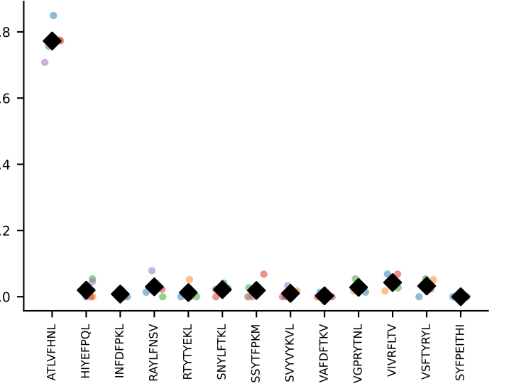
#58 AV16/DV11-CAMRHDTNAYKVIF-AJ30_BV5-CASSQDWGGAQDTQYF-BJ2-5 coh=0.991, n=5
