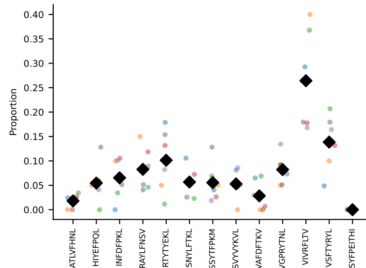
#211 AV9-3-CAVSENNNAGAKLTF-AJ39_BV1-CTCSAAWGDTQYF-BJ2-7 coh=0.819, n=20
