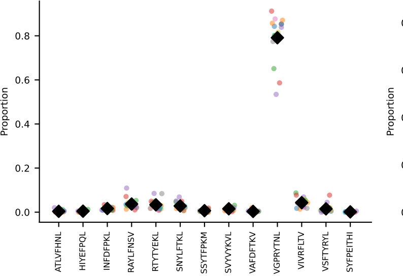
#57 AV6-5-CALSDLYANKMIF-AJ47_BV3-CASSFGTGGYEYF-BJ2-7 coh=0.991, n=15
