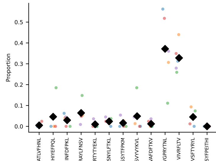
#214 AV19-CAAANTGYQNIFYF-AJ49_BV17-CASSRDPWGGSAAETLYF-BJ2-7 coh=0.817, n=34
