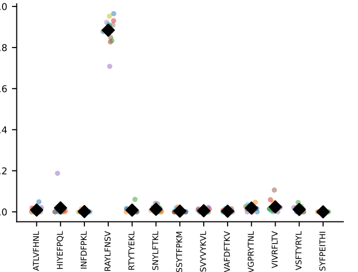
#54 AV13D-1-CAMVPNYNVLYF-AJ21*p03_BV13-1-CASSDLGGSSYEYF-BJ2-7 coh=0.992, n=7
