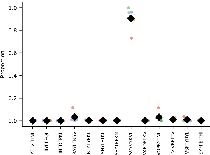
#65 AV9D-4-CALSANMGYKLTf-AJ9_BV13-1-CASEGTGGIYEQYF-BJ2-7 coh=0.990, n=8
