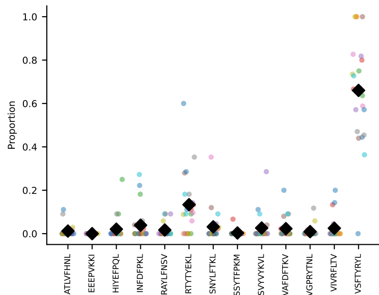
#16 AV12D-2-CALNQGGSAKLIF-AJ57_BV1-CTCSADWGNIAEQFF-BJ2-7 coh=0.818, n=21
