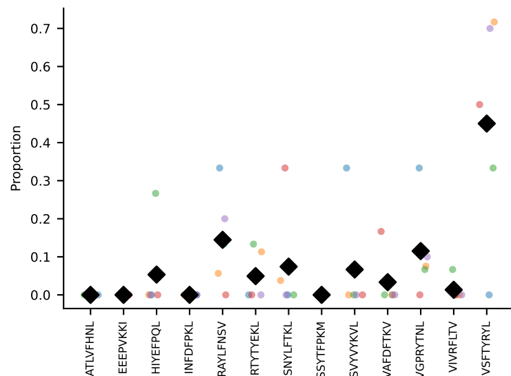
#191 AV6-7/DV9-CALSDHAGYQNFYF-AJ49_BV13-2-CASGARTGENYAEQFF-BJ2-1#192 AV19-CAAGNTGYQNFYF-AJ49_BV17-CASRDRGGERLFF-BJ1-4 coh=0.521, n=5
