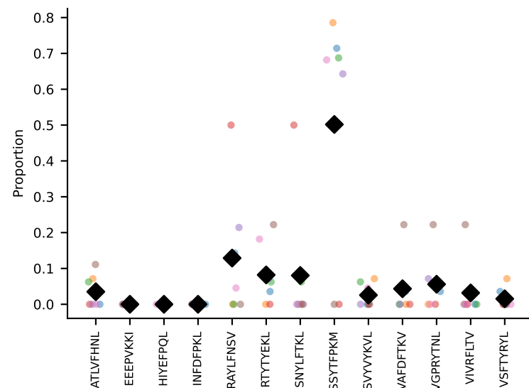
#192 AV19-CAAGNTGYQNFYF-AJ49_BV17-CASRDRGGERLFF-BJ1-4 coh=0.501, n=7
