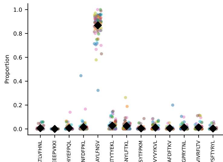
#47 AV16N-CAMREDSNYQLIW-AJ33_BV3-CASSLGQISNERLFF-BJ1-4 coh=0.977, n=76
