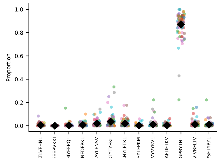
#48 AV5-4-CAASTDYANKMIF-AJ47_BV3-CASSSGTGYEQYF-BJ2-7 coh=0.975, n=88
