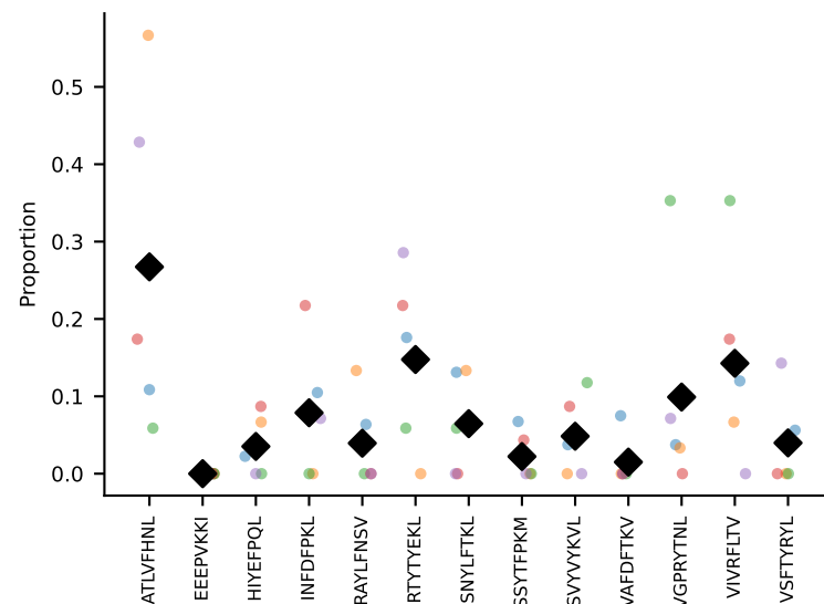
#190 AV6-6-CALGEAGGSNAKLTF-AJ42_BV14-CASSPGLSYNSPLYF-BJ1-6#191 AV6-7/DV9-CALSDHAGYQNFYF-AJ49_BV13-2-CASGARTGENYAEQFF-BJ2-1#192 AV19-CAAGNTGYQNFYF-AJ49_BV17-CASRDRGGERLFF-BJ1-4 coh=0.525, n=5
