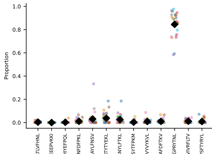
#46 AV9-4-CAVSGDYANKMIF-AJ47_BV3-CASSLGTGYEQYF-BJ2-7 coh=0.979, n=27
