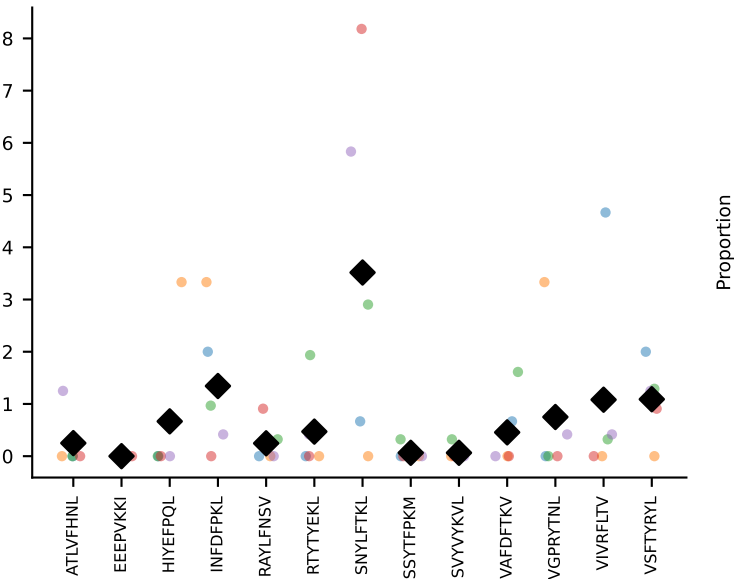
#207 AV7D-4-CAASDMGYKLTf-AJ9_BV2-CASSQDLGQGyAEQFF-BJ2-1 coh=0.368, n=5
