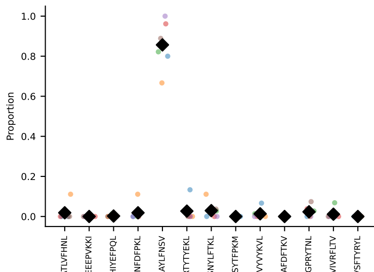
#45 AV16-CAMREDSNYQLIW-AJ33_BV3-CASSSGQISNERLFF-BJ1-4 coh=0.980, n=6
