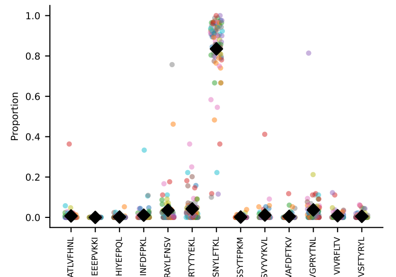
#132 AV13D-2-CAIDNNAGAKLTF-AJ39_BV13-3-CASRDRIYEQYF-BJ2-7 coh=0.897, n=26
