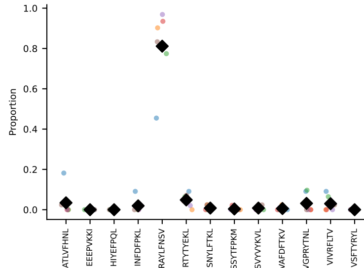
#80 AV10-CAASMTNSAGNKLTF-AJ17_BV26-CASRDWQGDTQYF-BJ2-5 coh=0.954, n=28
