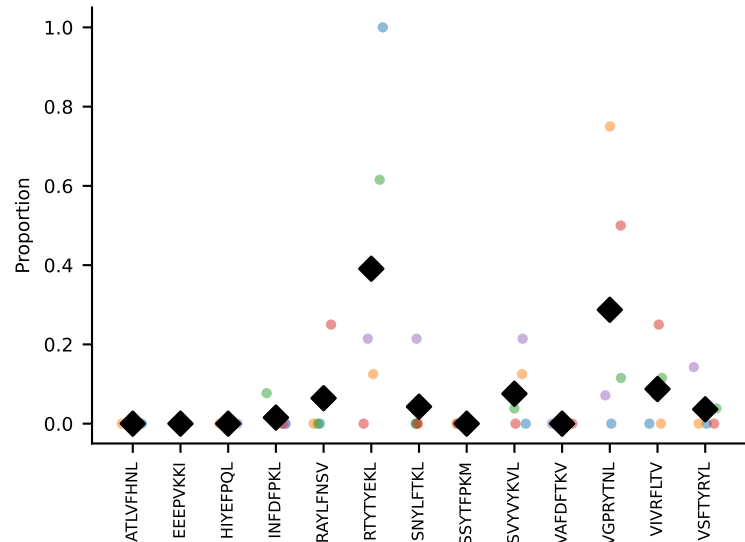
#235 AV4-4/DV10-CAAEETGGNNKLTf-AJ56_BV2-CASSQRPNTGQLYF-BJ2-2 coh=0.375, n=17
