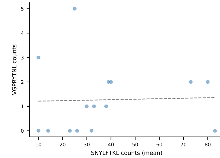
VGPRYTNL r=0.033 , p=9.07e-01
