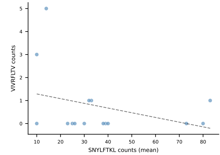
VIVRFLTV r=-0.336 , p=2.21e-01
