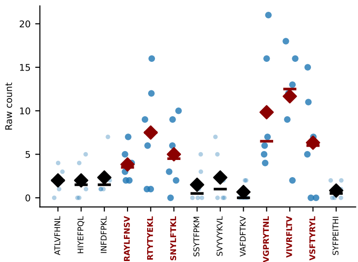
#216 AV13D-4-CAMTDGYONYF-AJ49_BV5-CASSQDSNTEVFF-BJ1-1 MULTI-SPECIFIC | Above BG: RAYLFNSV+RTYTYEKL+4more n=6 [HTxB:6] thresh=0.0
