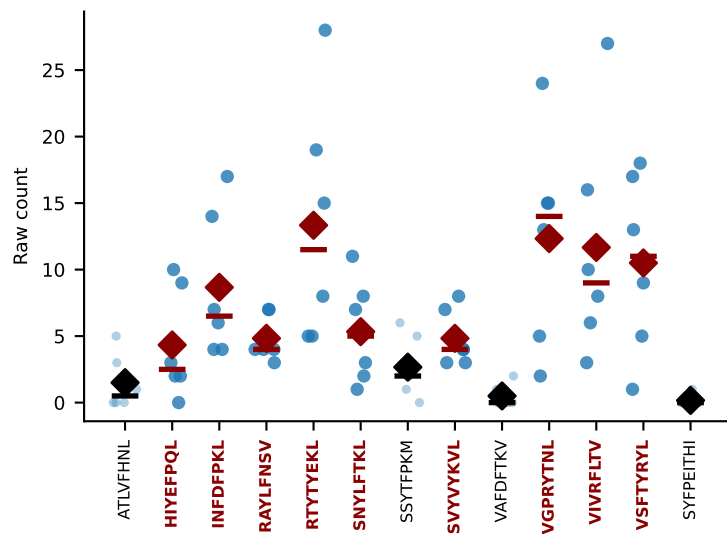
#207 AV16/DV11-CAMREEQQGTGSKLSF-AJ58_BV31-CAWRRQGGAYAEQFF-BJ2-1 MULTI-SPECIFIC | Above BG: HIYEPQL+INFDFPKL+7more n=6 [HTxB:6] thresh=0.0
