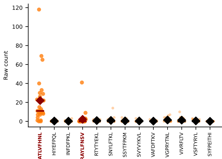
#102 AV8-2-CATDIOGGRALIF-AJ15_BV3-CASSWGGADSDYTF-BJ1-2 DUAL | Above BG: ATLVFHNL+RAYLFNSV n=27 [HTxC:27] thresh=0.0
