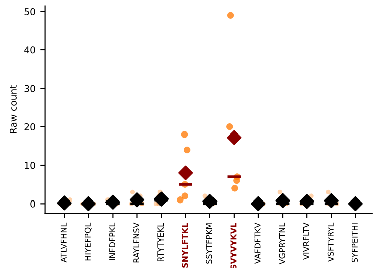
#97 AV16/DV11-CAMREGNTGYQNIFY-AJ49_BV13-2-CASGQGAGNTLYF-BJ1-3 DUAL | Above BG: SNYLF TKL+SVVYKVL n=5 [HTxC:5] thresh=0.0
