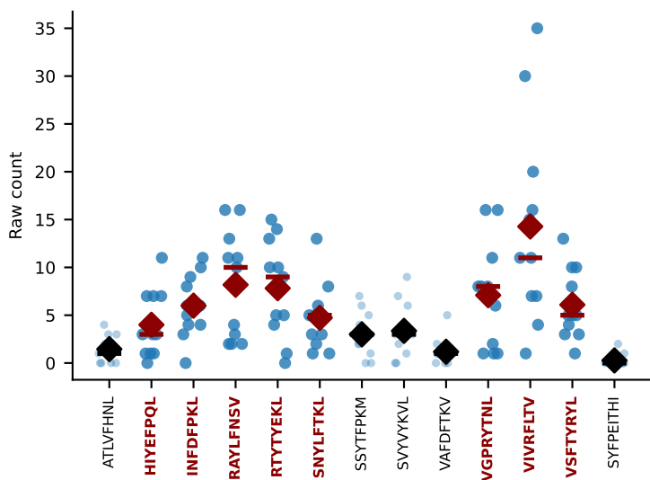
#210 AV13-1-CAANTGANTGKLTf-AJ52_BV17-CASSPGQGHTGQLYF-BJ2-2 MULTI-SPECIFIC | Above BG: HIYEPQL+INFDFPKL+6more n=11 [HTxB:11] thresh=0.0
