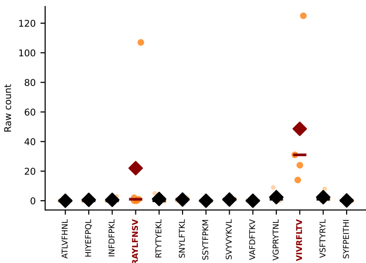
#104 AV8-1-CATEPDTGYQNIFY-AJ49_BV3-CASSLAWGLNYAEQFF-BJ2-1 DUAL | Above BG: RAYLFNSV+VIVRFLTV n=5 [HTxC:5] thresh=0.0
