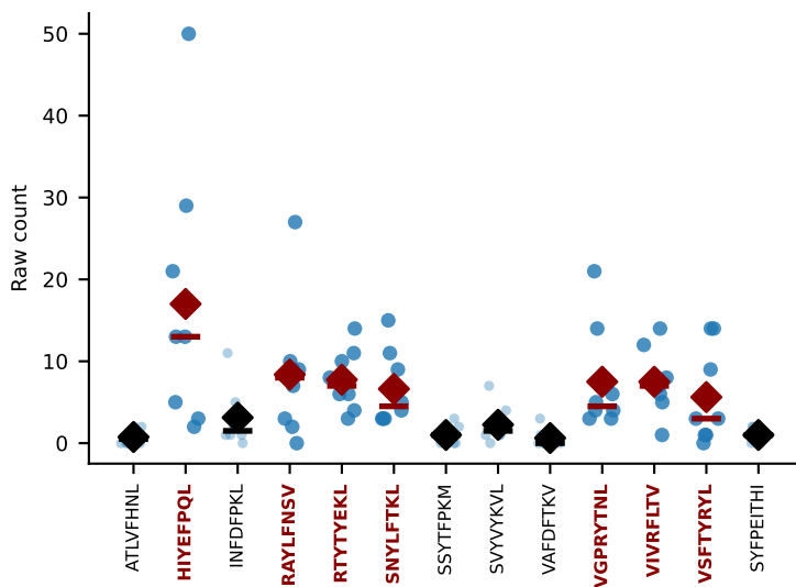
#214 AV16D/DV11-CAMRVSNTRYQNYF-AJ49_BV1-CTCSEDVRVYAEQFF-BJ2-1 MULTI-SPECIFIC | Above BG: HIYEPQL+RAYLFNSV+5more n=8 [HTxB:8] thresh=0.0
