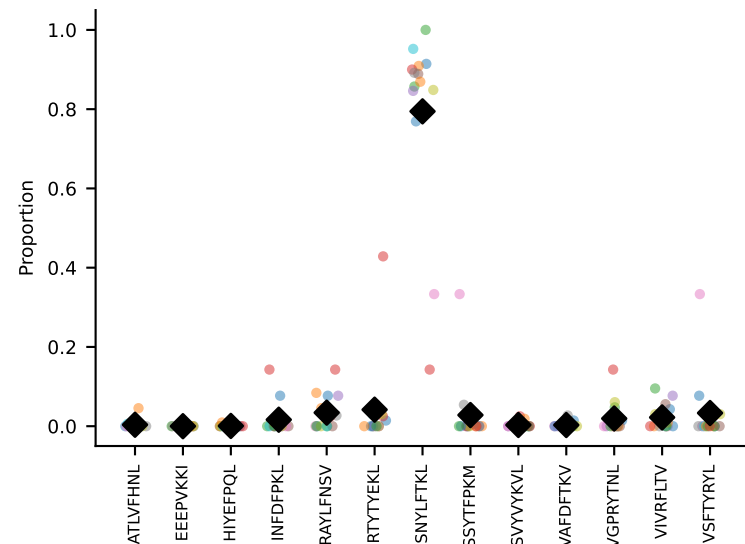
#21 AV19-CAAGITGYQNFYF-AJ49_BV17-CASSRLGSSYEQYF-BJ2-7 coh=0.839, n=14
