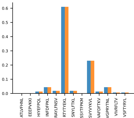
AV16/DV11-CAMREGDSGYNKLTF-AJ11_BV13-2-CASGTGGANTLYF-BJ2-1 PROP n:5→5
