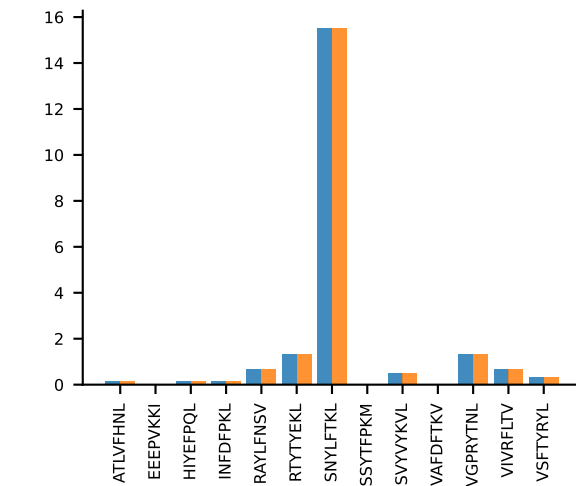
AV16/DV11-CAMREGDSGYNKLTF-AJ11_BV13-2-CASGTGGANTLYF-BJ2-1 MEAN n:5→5
