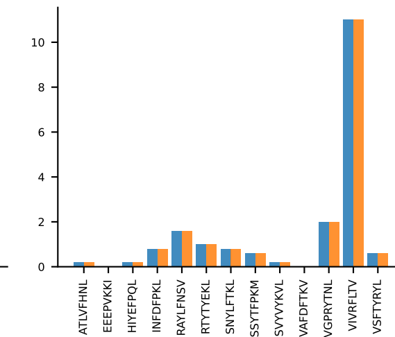
AV7-2-CAASRGDYANKMIF-AJ47_BV13-3-CASSARVEQYF-BJ2-7 MEAN n:5→5
