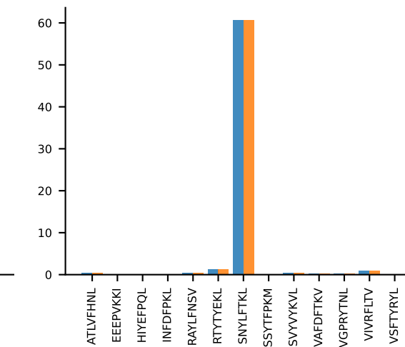
AV11-CVVGANNYAQGLTF-AJ26_BV13-2-CASGDVGGNSPLYF-BJ1-16 MEAN n:5→5
