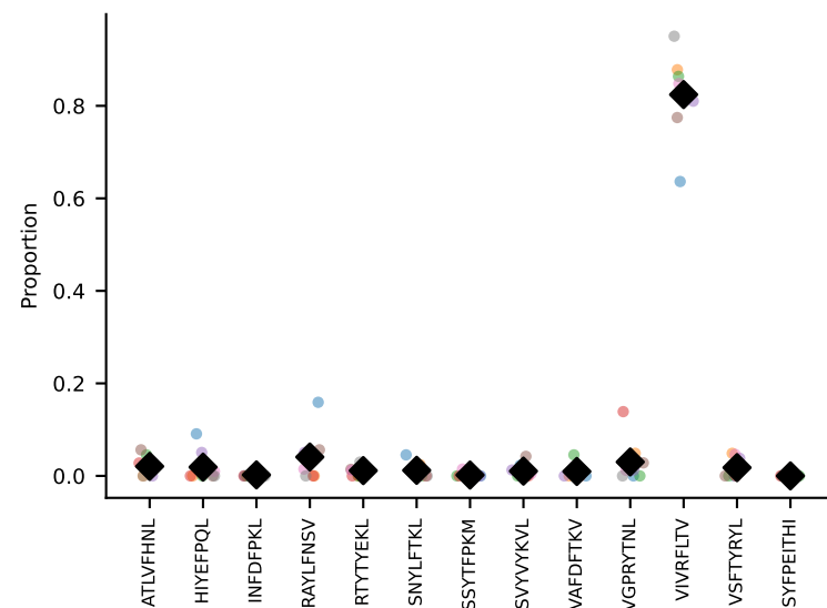
#57 AV16/DV11-CAGTGGADRLTF-AJ45_BV3-CASSPDNANTEVFF-BJ1-1 coh=0.982, n=7
