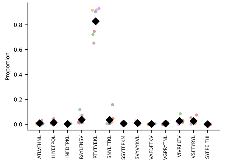
#56 AV16D/DV11-CAMREDTGNYKYVF-AJ40_BV13-2-CASGALTEVFF-BJ1-1 coh=0.982, n=5
