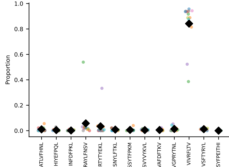
#91 AV16/DV11-CAMREANYGNEKITF-AJ48_BV1-CTCSADRVHSDYTF-BJ1-1#92 AV16D/DV11-CAMREGSSGSWQLIF-AJ22_BV1-CTCSADRVAETLYF-BJ1-1 coh=0.897, n=10
