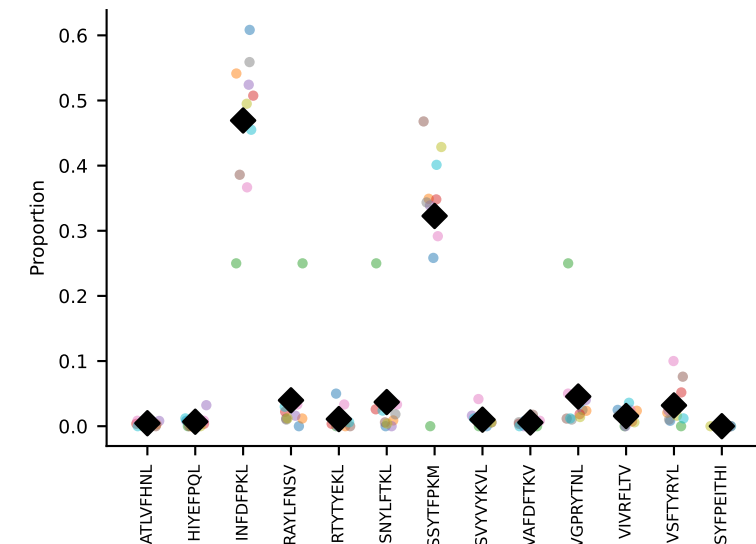
#93 AV13-1-CAMTGNTRKLIF-AJ37*p02_BV13-1-CASSPGTGFAEQFF-BJ2-1#94 AV8D-2-CATEANSPTYQRF-AJ13_BV3-CASSPPGGGDTQYF-BJ2-5 coh=0.867, n=10
