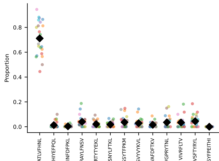
#71 AV19-CAAGGTGYQNIFYF-AJ49_BV1-CTCSAGNPSAETLYF-BJ2-3 coh=0.959, n=24
