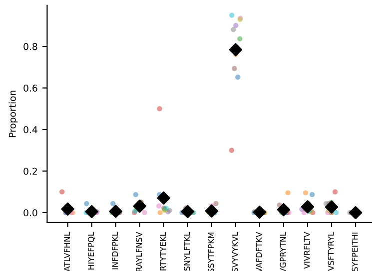
#94 AV8D-2-CATEANSPTYQRF-AJ13_BV3-CASSPPGGGDTQYF-BJ2-5#95 AV13-1-CAMEPGGNNKLTF-AJ56_BV13-3-CASSDRYEQYF-BJ2-7 coh=0.860, n=14
