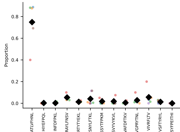
#80 AV13-1-CAMPSSGSWQLIF-AJ22_BV4-CASSYSGEQYF-BJ2-7 coh=0.936, n=6
