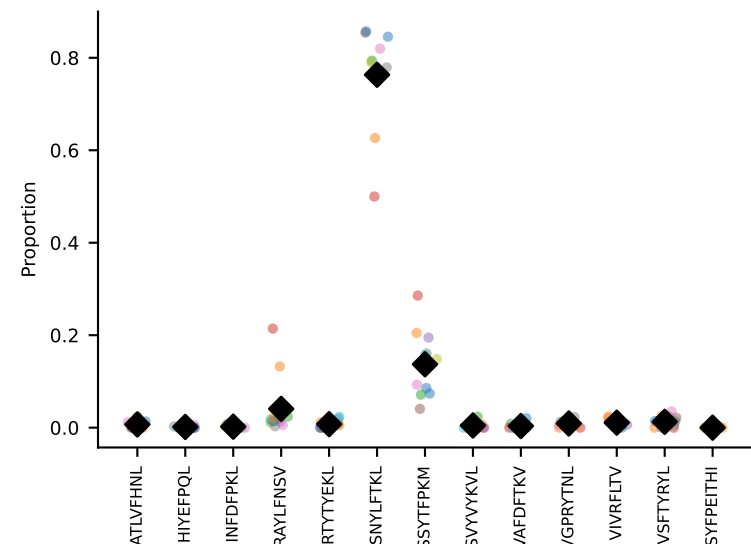
#68 AV16/DV11-CAMREDTGYNFYF-AJ49_BV13-2-CASGGVGYAEQFF-BJ1-1 coh=0.963, n=5
