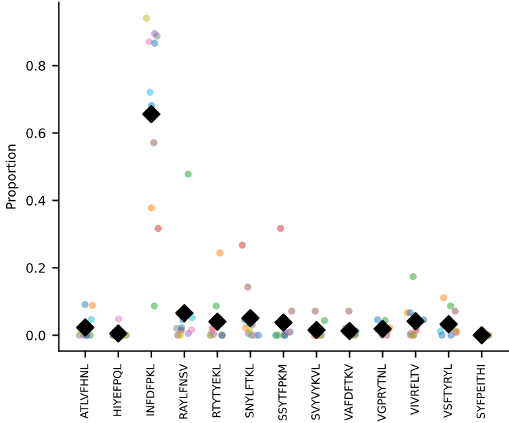
#98 AV7D-2-CAANDWAGNTRKLIF-AJ37*p02_BV13-2-CASGDPDGYAEQFF-BJ2-7 coh=0.759, n=11
