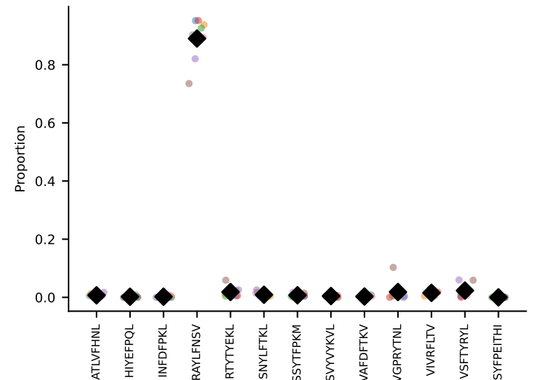
#20 AV16/DV11-CAMREGSTGYQNFYF-AJ49_BV13-2-CASGEQVYEQYF-BJ2-7 coh=0.995, n=10
