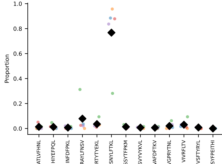
#95 AV13-1-CAMEPGGNNKLTF-AJ56_BV13-3-CASSDRYEQYF-BJ2-7#96 AV14D-1-CAASKDTGNYKYVF-AJ40_BV13-3-CASSDSNTEVFF-BJ1-1 coh=0.860, n=5
