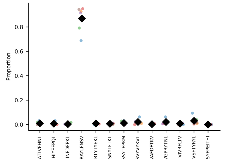
#24 AV7-5-CAMSSPPSNTDKVVF-AJ34*p03_BV1-CTCSAVRVSGNTLYF-BJ2-7 coh=0.994, n=6
