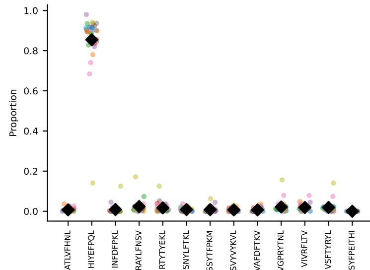
#77 AV6-4-CALVEGGRALIF-AJ15_BV14-CASRDRTQYF-BJ2-5 coh=0.945, n=5
