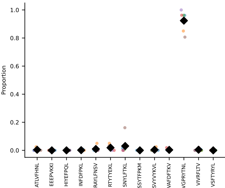
#3 AV10-CAASTDYANKMIF-AJ47_BV3-CASSLAHSYEQYF-BJ2-7 coh=0.992, n=6
