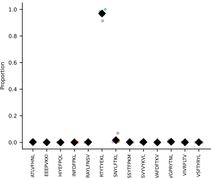
#1 AV16-CAMRKEGADRLTF-AJ45_BV13-1-CASSDNYEQYF-BJ2-7 coh=0.999, n=6
