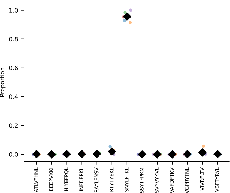
#2 AV16/DV11-CAMREGTNAYKVIF-AJ30_BV13-2-CASGDAWGQAGNTLYF-BJ1-3 coh=0.999, n=5
