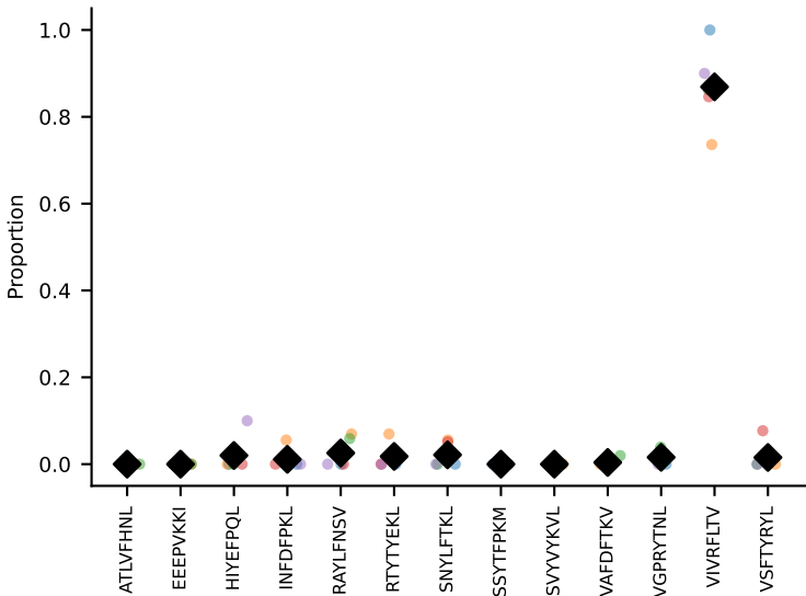
#29 AV14-2-CAASGGYNQGKLIF-AJ23_BV3-CASSLGFQDTQYF-BJ2-5 coh=0.985, n=73
