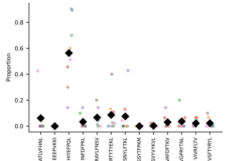
#144 AV13D-1-CAMERSNNRIFF-AJ31_BV2-CASSQDRRGDTQYF-BJ2-5 coh=0.678, n=8
