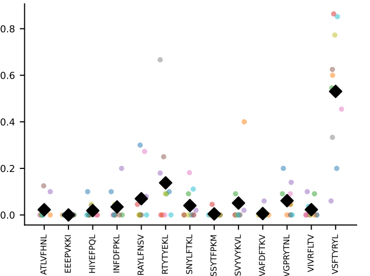
#150 AV13N-4-CAMEPSSSFSLVLF-AJ50_BV31-CAWSLGGAEQFF-BJ2-1 coh=0.607, n=5
