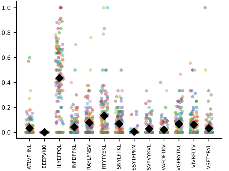
#156 AV16N-CAMREEAGNTGKLIF-AJ37_BV20-CGARDWGGYEYF-BJ2- coh=0.559, n=32
