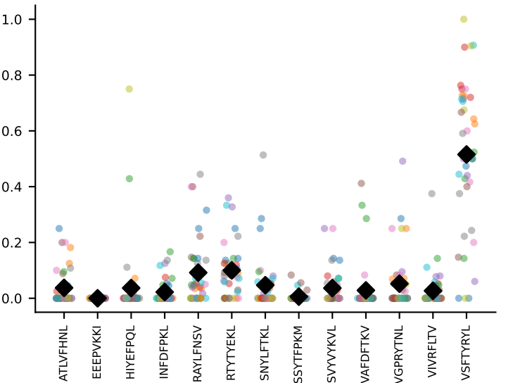
#151 AV14-2-CAASASSGSWQLIF-AJ22_BV31-CAWSLAGSGNTLYF-BJ1-3 coh=0.594, n=8
