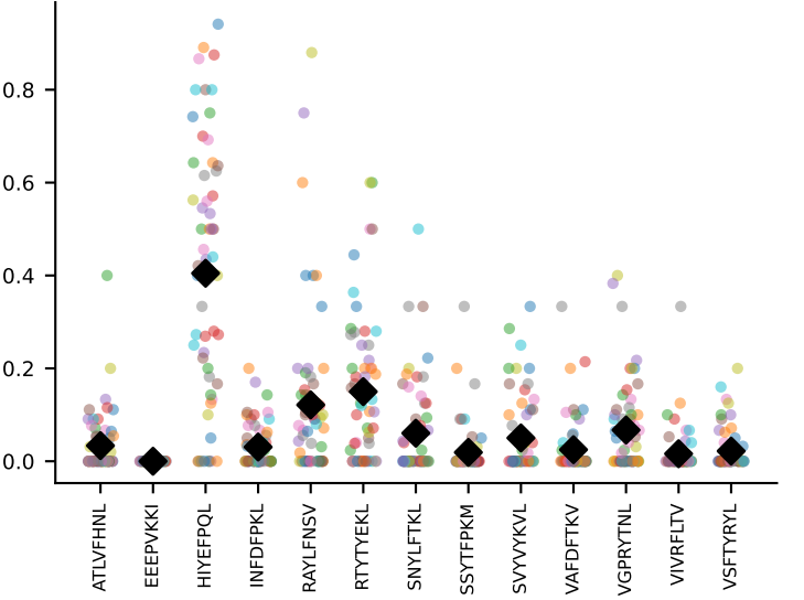
#155 AV13N-1-CAMERSNNRIFF-AJ31_BV2-CASSQDRRGGEQYF-BJ2-7 coh=0.564, n=58
