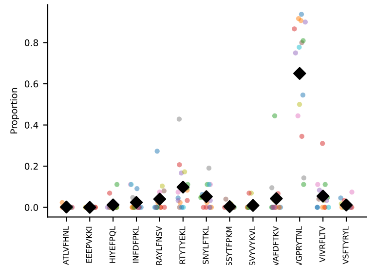
#140 AV12D-2-CALNQGGSAKLIF-AJ57_BV1-CTCSADWGNAYAEQFF-BJ2-5 coh=0.745, n=49
