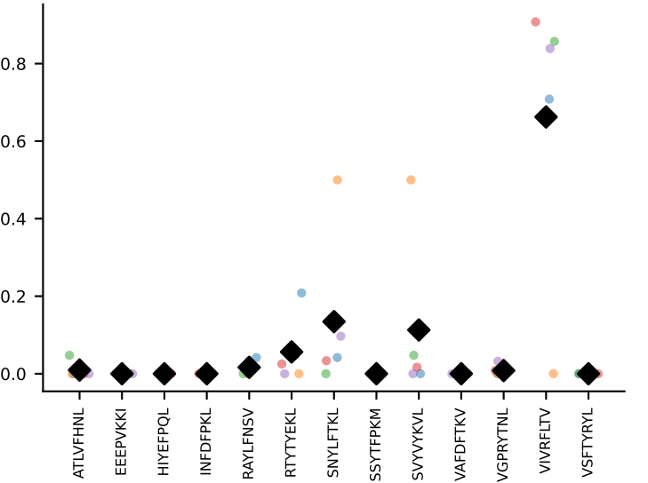
#154 AV8D-2-CATDDQGGRALIF-AJ15_BV19-CASSSGVNERLFF-BJ1-4 coh=0.572, n=9
