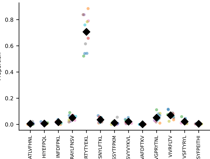
#8 AV15-1/DV6-1-CALWELASSNTDKVVF-AJ34*p03_BV3-CASSFGTGGYYEQYF-BJ2-5 coh=0.955, n=10
