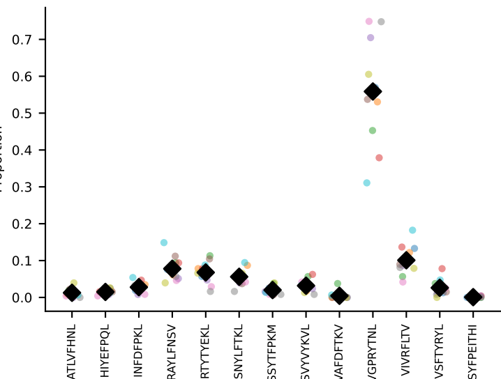
#12 AV6D-7-CALRYGGSGNKLIFF-AJ32_BV3-CASSLGTGDTQYF-BJ2-5 coh=0.921, n=10
