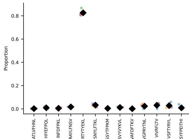
#7 AV7D-5-CAVSSSGGNYKPTF-AJ6_BV3-CASSQDRTGTSAETLYF-BJ2-3 coh=0.997, n=10
