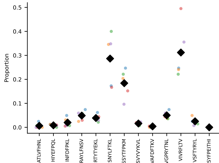
#70 AV16/DV11-CAMREGDTNAYKVIF-AJ30_BV13-2-CASGEINSPLYF-BJ1-6#71 AV16D/DV11-CAMRNYAQLTF-AJ26_BV13-2-CASGGGGGEQYF-BJ2-7#72 AV16D/DV11-CAMREGNTGNYKYVF-AJ40_BV13-2-CASGDLYEQYF-BJ2-1 coh=0.878, n=6
