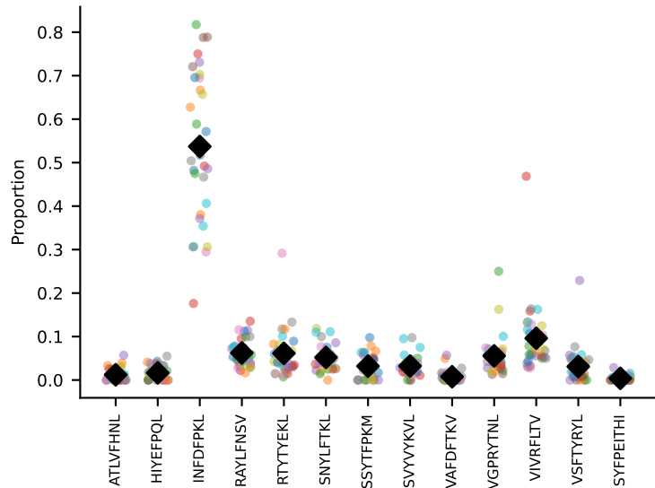
#65 AV16/DV11-CAMREGYQNFYF-AJ49_BV13-1-CASSGRNTEVFF-BJ1-1 coh=0.890, n=7
