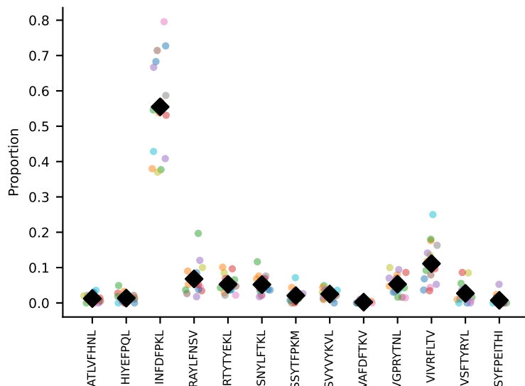
#46 AV5-1-CSASTGGFASALTF-AJ35_BV2-CASSQDGAGANSQYTF-BJ1-2 coh=0.941, n=6
