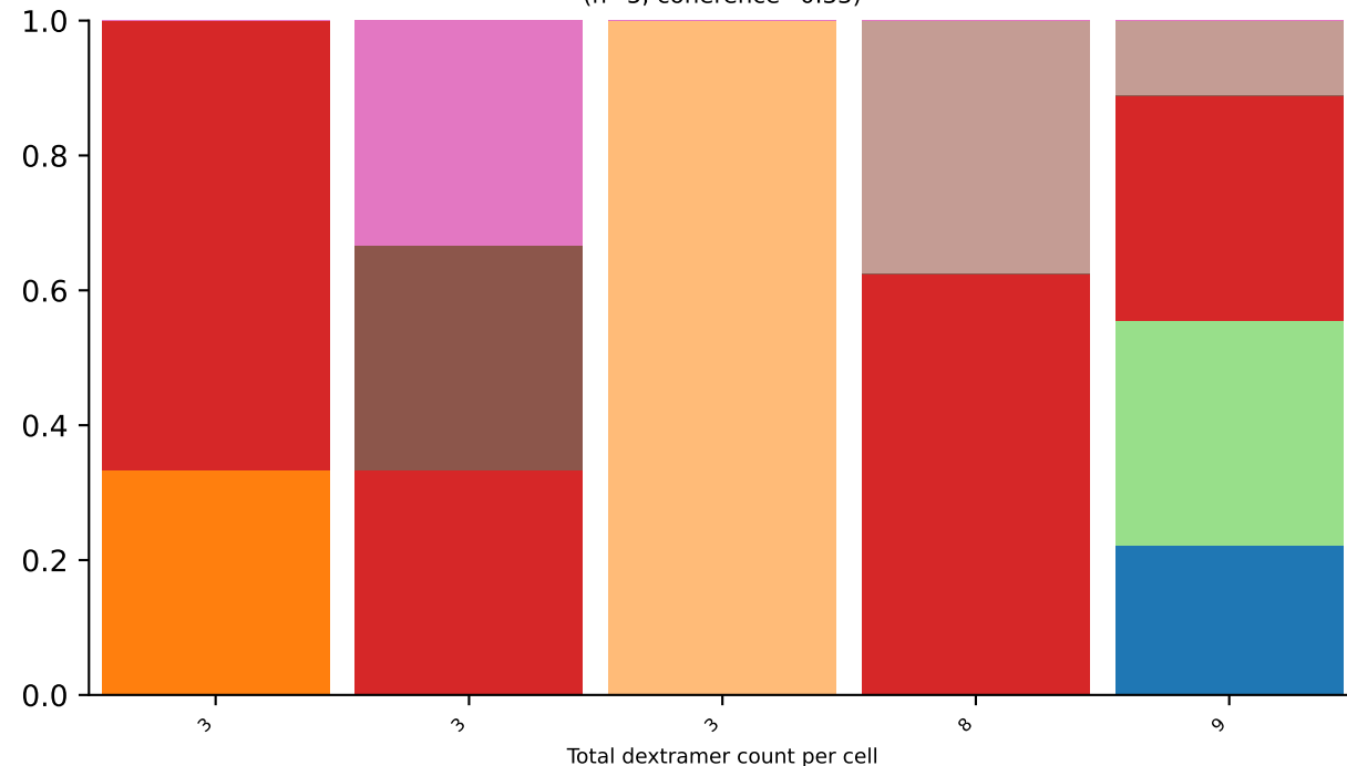
Dual AV14-2-CAASASSGSWQLIF-AJ22/AV15-2/DV6-2-CALSERSSGSWQLIF-AJ22_BV31-CAWSLAGSGNTLYF-BJ1-3 (n=5, coherence=0.33)
