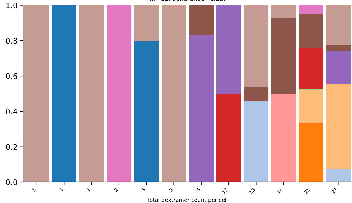
Dual AV12D-2-CALSDRGNMGYKLTf-AJ9/AV8D-2-CATDTGGLSGKLTf-AJ2_BV13-1-CASSPGQYAEQFF-BJ2-1 (n=12, coherence=0.18)
