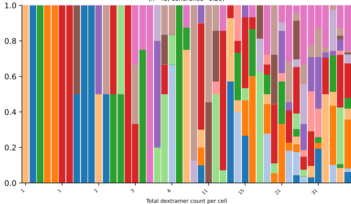
Single(s) AV8 / BV13 CATDTGGLSGKLTf / CASSPGQYAEQFF 1 clonotype(s) (n=45, coherence=0.20)
