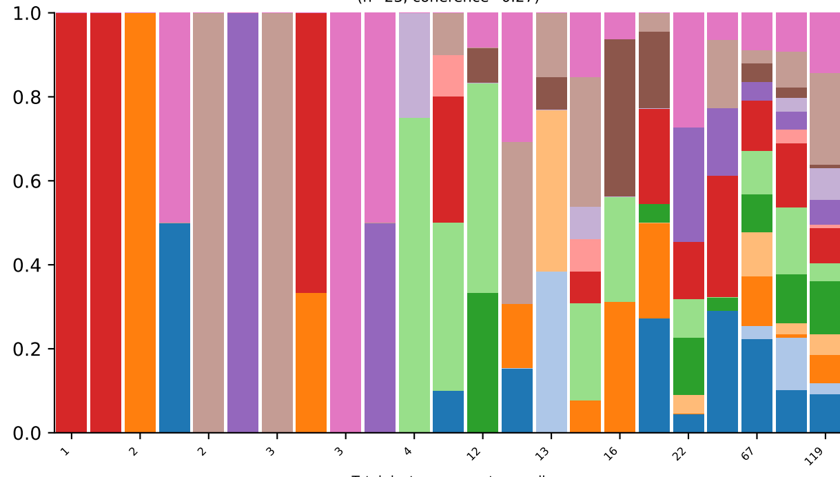
Single(s) AV14 / BV31 CAASASSGSWQLIF / CAWSLAGSGNTLYF 1 clonotype(s) (n=23, coherence=0.27)
