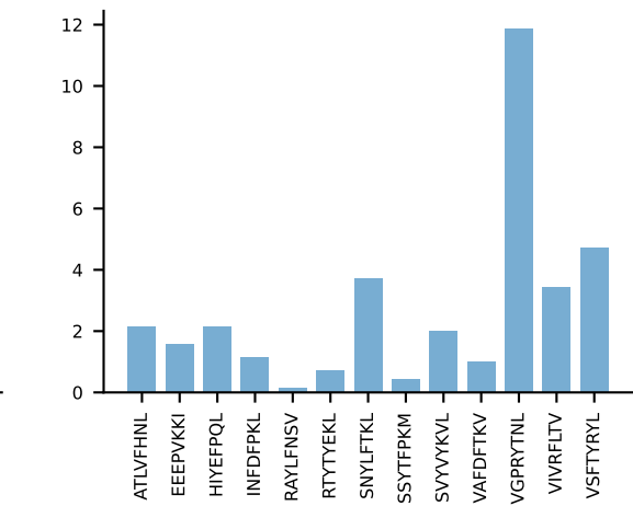
AV13D-2-CAIGGGSALGRLHF-AJ18_BV12-2-CASSPGQAAEQFF-BJ1-2 MEAN n:7→0 LOST
