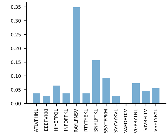
AV3D-3-CAVHYAQGLTF-AJ26_BV1-CTCSADRNSDYTF-BJ1-2 PROP n:7→0 LOST
