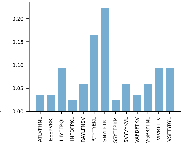
AV13D-2-CAIGGGSALGRLHF-AJ18_BV12-2-CASSPGQAAEQFF-BJ1-2 PROP n:7→0 LOST
