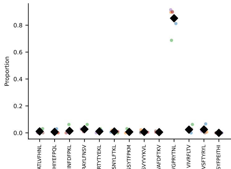
#30 AV16D/DV11-CAMREGGNNRIFF-AJ31_BV13-2-CASGGVYEYF-BJ2-7 coh=0.994, n=5
