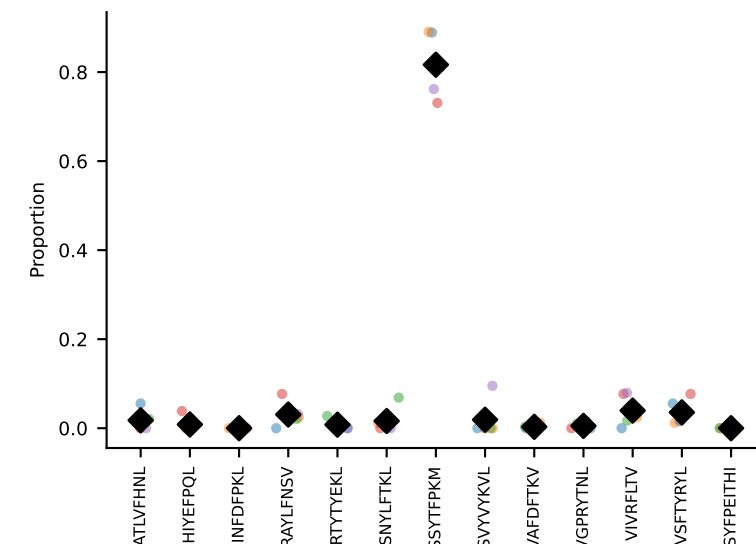
#45 AV6-6-CALGDHTGYQNFYF-AJ49_BV13-3-CASSEN RVNTEVFF-BJ1-1 coh=0.989, n=5
