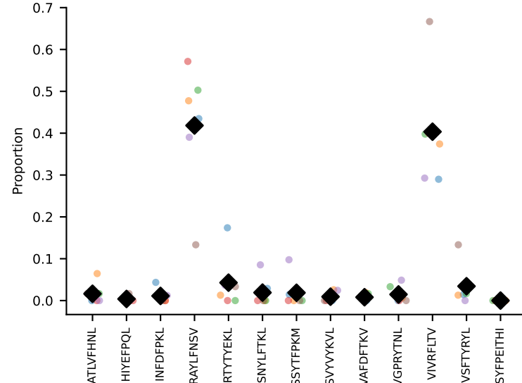
#106 AV13-1-CAMEPGGNNKLTf-AJ56_BV13-3-CASSDRYEYF-BJ2-7 coh=0.860, n=5
