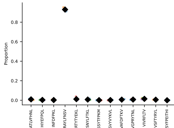
#6 AV16/DV11-CAMREDTNAYKVIF-AJ30_BV13-2-CASGDPGNQAPLF-BJ1-5 coh=0.999, n=7
