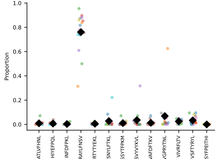
#103 AV16D/DV11-CAMREGSSGSWLIF-AJ22_BV1-CTCSADRVAEITLYF-BJ2-7 coh=0.880, n=7
