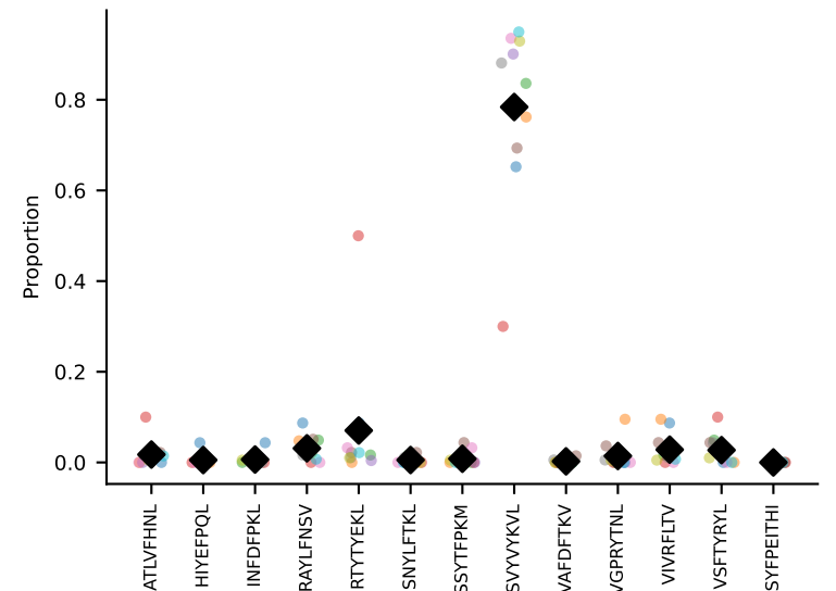
#104 AV13-1-CAMTGNTKRLIF-AJ37*p02_BV13-1-CASSPGTGFAEQFF-BJ2-7 coh=0.867, n=10
