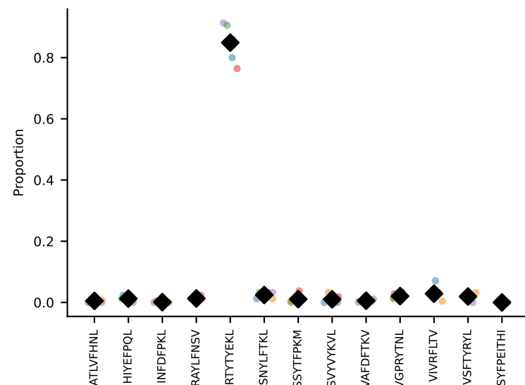
#21 AV16/DV11-CAMREDNAGAKLTF-AJ39_BV1-CTCSAARVDTQYF-BJ2-5 coh=0.996, n=8
