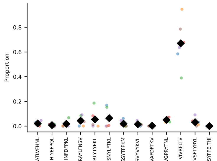
#91 AV6D-7-CALSEVSGGNYKPTF-AJ6_BV14-CASSLGANSDYTF-BJ1-2 coh=0.931, n=14
