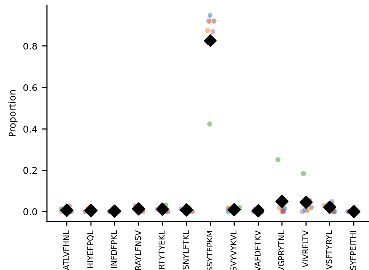
#90 AV7D-5-CAVAYQGGRALIF-AJ15_BV13-1-CASSDVGTISNERLFF-BJ1-4 coh=0.931, n=12
