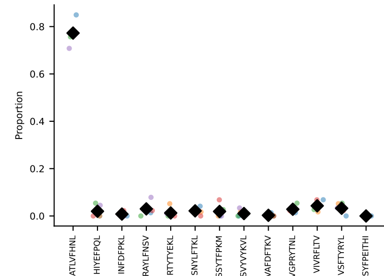
#41 AV16D/DV11-CAMREGGSAGNKLTF-AJ17*p02_BV1-CTCSADRVGNTLYF-BJ1-2 coh=0.990, n=9
