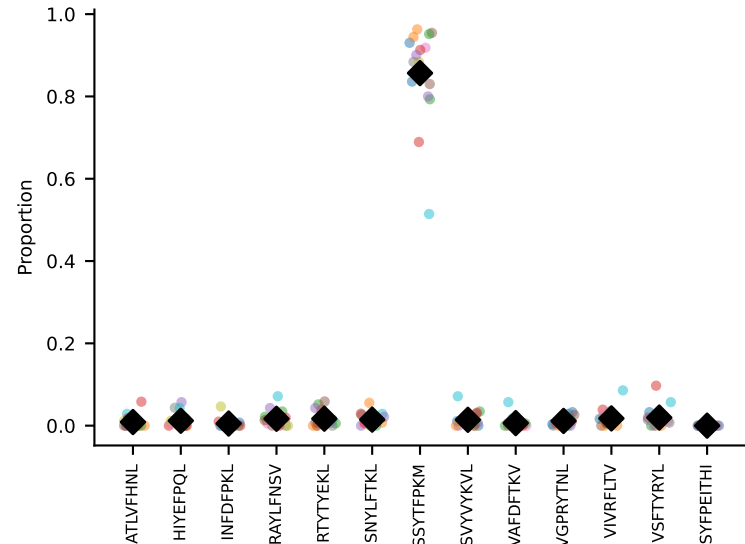
#42 AV16/DV11-CAMRSNTGYQNFYF-AJ49_BV13-2-CASGDRGRNTLYF-BJ2-1 coh=0.990, n=11
