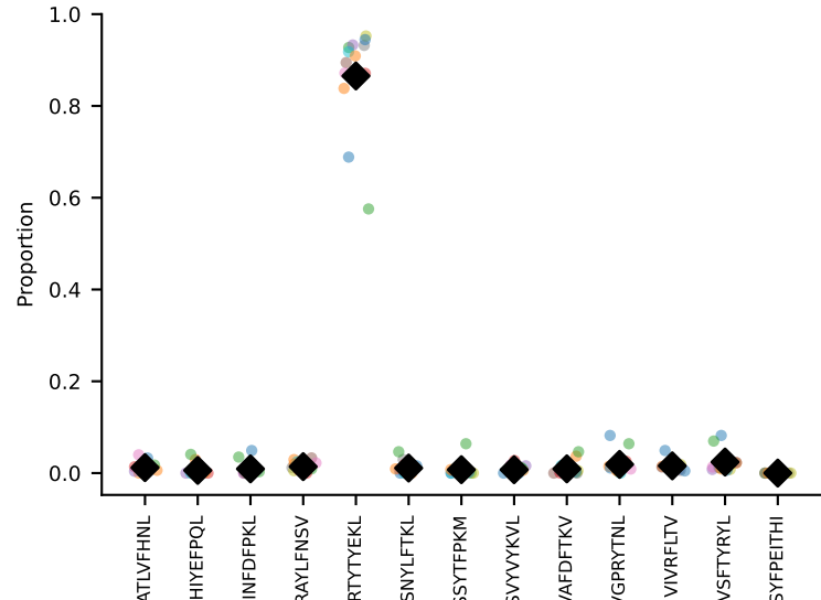
#35 AV13D-1-CAMVPNYNVLYF-AJ21*p03_BV13-1-CASSDLGGSSYEYF-BJ2-7 coh=0.992, n=7
