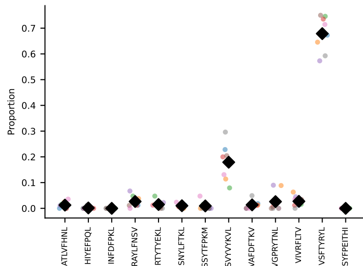
#67 AV16/DV11-CAMRESTGANTGKLTf-AJ52_BV13-3-CASSPGTVYAEQFF-BJ2-5 coh=0.977, n=6
