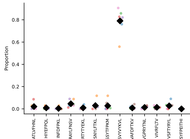
#66 AV14D-2-CAASPDGTGNYKYVF-AJ40_BV13-3-CASSDNGNNQAPLF-BJ2-5 coh=0.977, n=9
