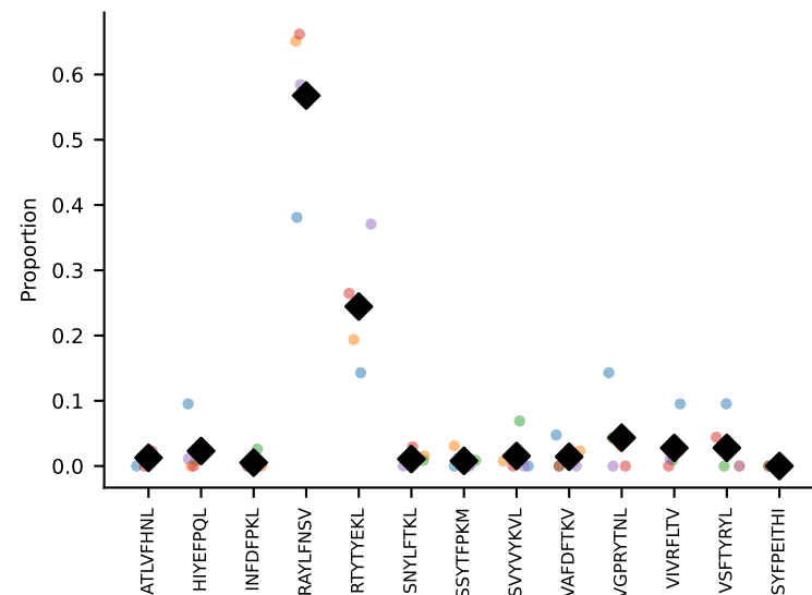
#89 AV3-3-CAVSAGQGGRALIF-AJ15_BV13-1-CASSDTGGYEYF-BJ2-7 coh=0.933, n=24
