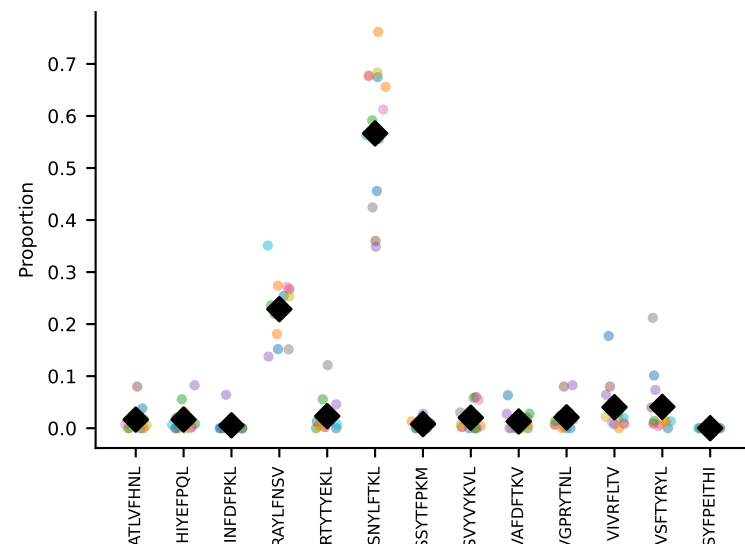
#81 AV16D/DV11-CAMREGGAYKVIF-AJ30_BV13-2-CASGDAYERLFF-BJ1-4 coh=0.948, n=13
