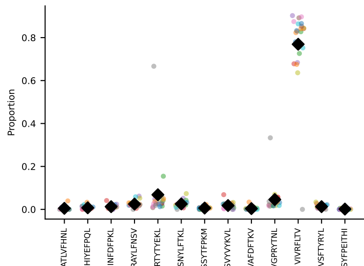
#72 AV6-6-CALGTFSNTDKVVF-AJ34*p03_BV13-1-CASSDVRDSGNTLYF-BJ1-3 coh=0.910, n=22
