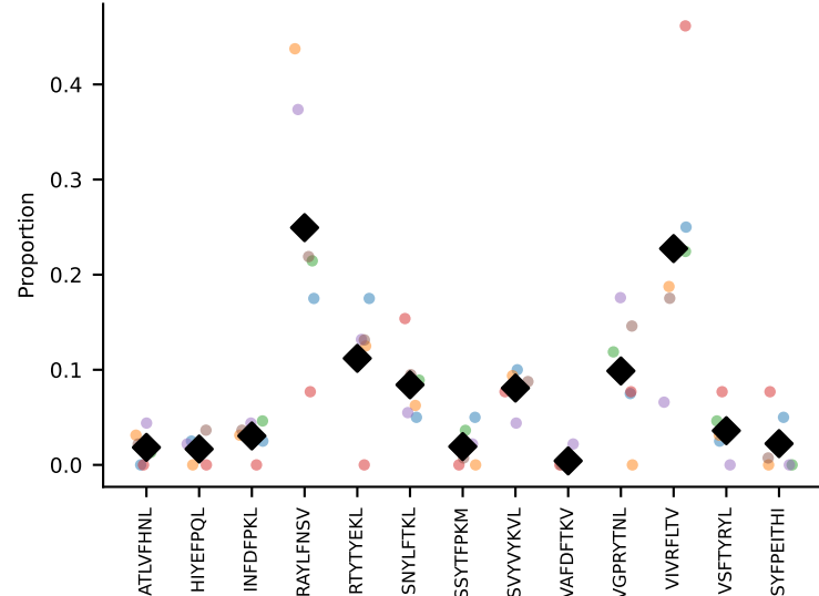
#115 AV12-2-CALSDTGANTGKLTf-AJ52_BV1-CTCSADPSYEQYf-BJ2-7-#116 AV16/DV11-CAMREGLGGNNKLTf-AJ56_BV1-CTCSAAGTGNTevff-BJ1-3 coh=0.781, n=7
