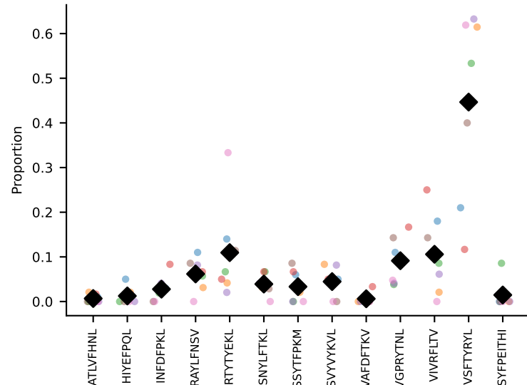
#119 AV13-1-CAMNQGSsAKLIF-AJ57_BV1-CTCSALNYAEQFF-BJ2-1-#120 AV16D/DV11-CAMRDTNAYKVIf-AJ30_BV13-2-CASGDVGGGQNTLYf-BJ1-3 coh=0.768, n=5
