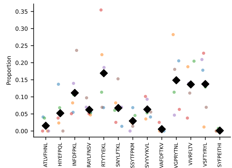
#132 AV16D/DV11-CAMRVSNTRYQNFYF-AJ49_BV1-CTCSEDVYAEQFF-BJ1-1 coh=0.716, n=8
