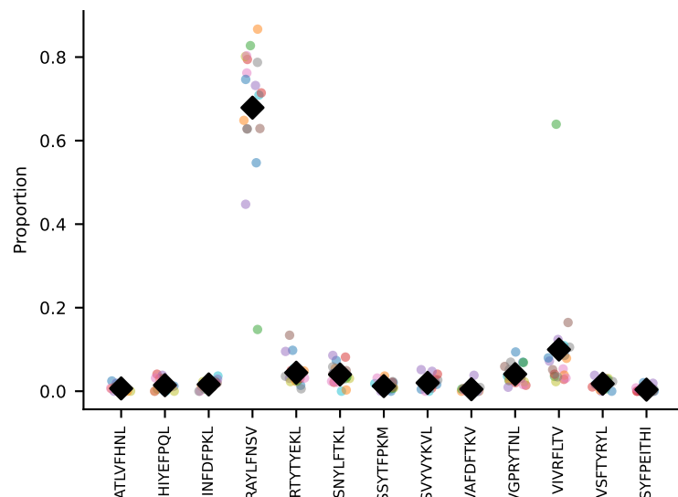
#71 AV8-1-CATDASSGSWQLIF-AJ22_BV4-CASTAANTEVFF-BJ1-1 coh=0.912, n=18
