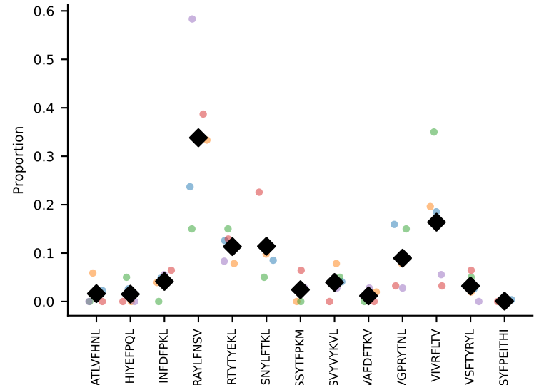
#120 AV16D/DV11-CAMRDTNAYKVIf-AJ30_BV13-2-CASGDVGGGQNTLYf-BJ1-3 coh=0.767, n=9
