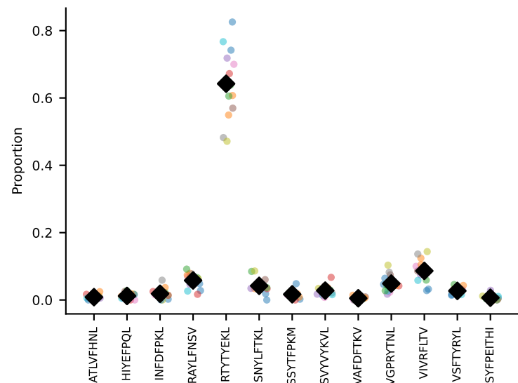
#32 AV10-CAASMDNYNVLVIF-AJ21*p03_BV31-CAWSLSSDYTF-BJ1-2 coh=0.979, n=7
