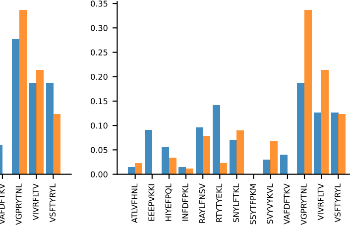
AV13-2-CAIDPNYNVLYf-AJ21_BV13-1-CASRDSNGNTLYf-BJ1-3 PROP n:8→7
