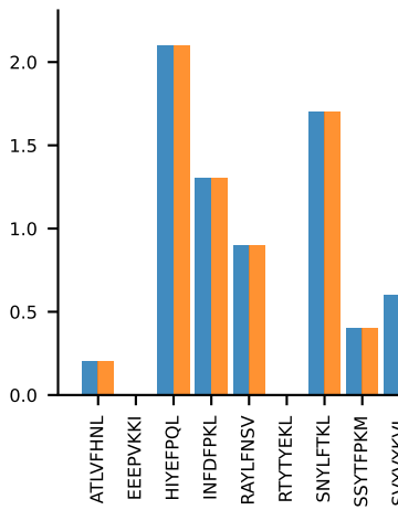
AV7-4-CAAVITGNTGKLIF-AJ37_BV13-1-CASSGGNYAEQFF-BJ2-1 MEAN n:9→6
