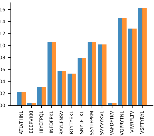
AV13-1-CALGTNSAGNKLTf-AJ17_BV2-CASSQDRVYEQYf-BJ2-7 PROP n:9→9
