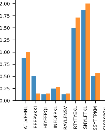
AV13-2-CAIDPNYNVLYf-AJ21_BV13-1-CASRDSNGNTLYf-BJ1-3 MEAN n:8→7
