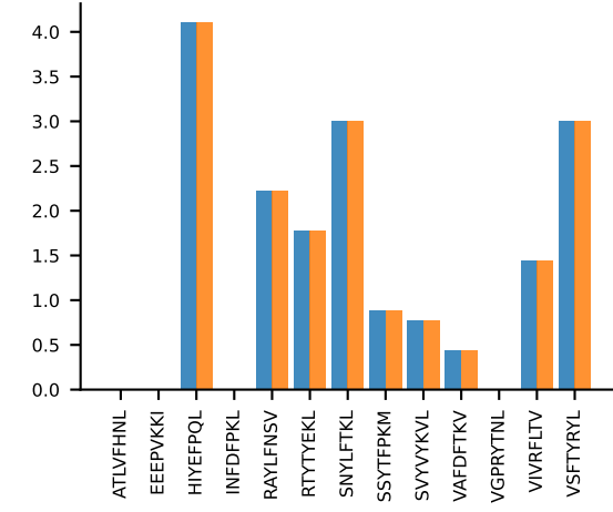
AV9D-3-CAVSMQGGRALIF-AJ15_BV13-3-CASRDRDEQYf-BJ2-7 MEAN n:9→7
