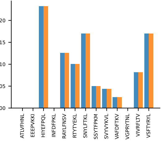
AV9D-3-CAVSMQGGRALIF-AJ15_BV13-3-CASRDRDEQYf-BJ2-7 PROP n:9→7
