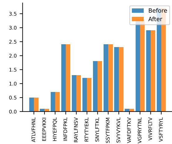
AV13-1-CALGTNSAGNKLTf-AJ17_BV2-CASSQDRVYEQYf-BJ2-7 MEAN n:9→9
