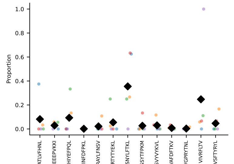
#24 AV12-1-CALSETGNTGKLIF-AJ37_BV13-2-CASGDAGTNTTEVFF-BJ1-1 coh=0.427, n=5
