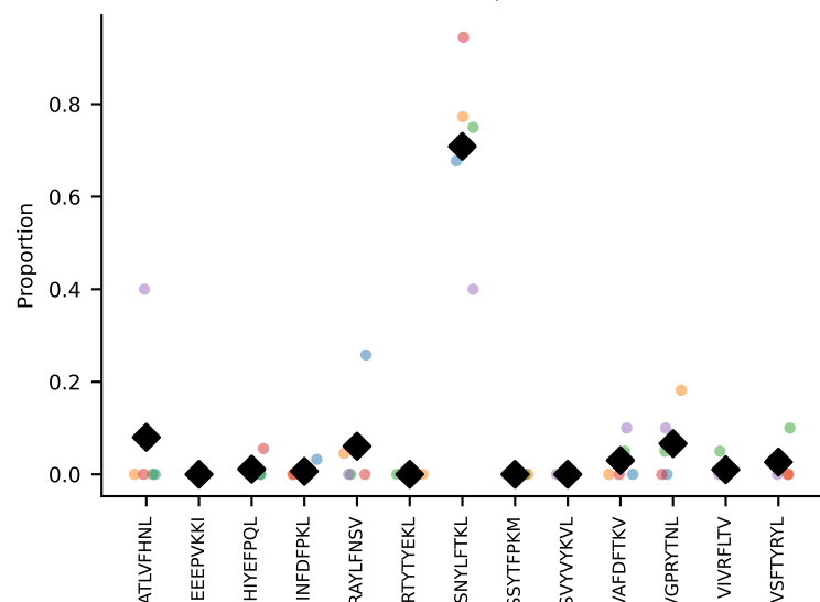
#404 AV7-2-CAAINNTNTGKLTFF-AJ27_BV13-2-CASGDAGGGNERLFF-BJ1-4 coh=0.844, n=5
