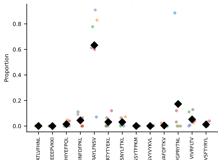
#363 AV3-3-CAVSSNNRIFF-AJ31_BV1-CTCSAVRVGNTLYF-BJ1-3 coh=0.689, n=6
