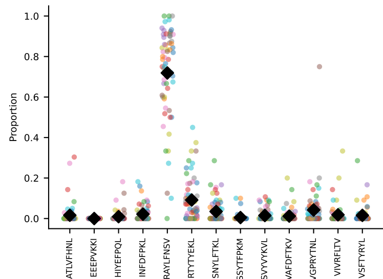
#403 AV14-1-CAASADTGNYKYVF-AJ40_BV13-3-CASSGTGTQNTLYF-BJ2-1 coh=0.847, n=10
