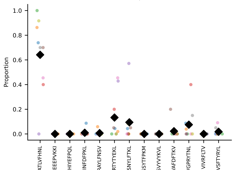
#364 AV8D-2-CATDSQGGRALIF-AJ15_BV3-CASSLGTGGEQYF-BJ2-7 coh=0.688, n=9
