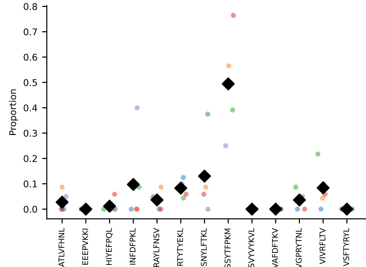
#360 AV7-3-CAVSGGNYKPTF-AJ6_BV31-CAWSYRGETLYF-BJ2-3 coh=0.711, n=7
