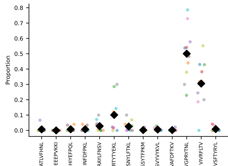
#334 AV13-2-CAIDNNAGAKLTFF-AJ39_BV13-3-CASSDRDTLYF-BJ2-4 coh=0.841, n=28
