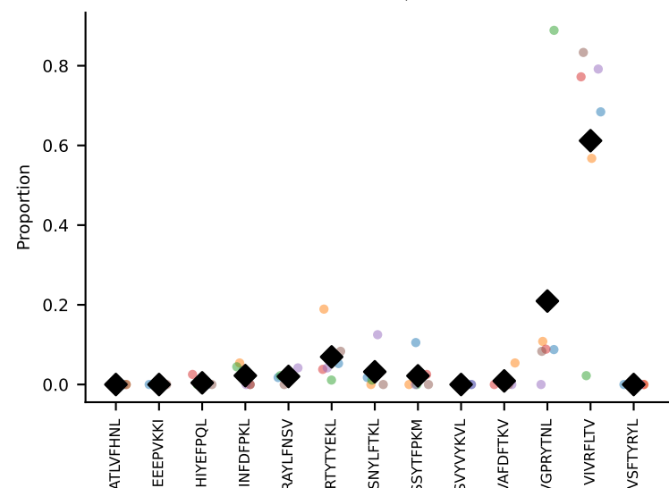
#362 AV16/DV11-CAMRENTGGLSGKLTF-AJ2_BV13-1-CASSDEQYNNQAPLF-BJ1-5 coh=0.691, n=6
