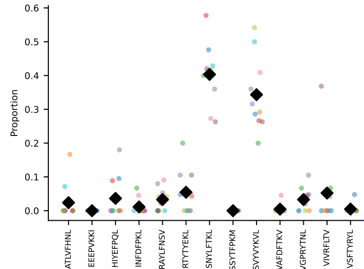
#326 AV5-4-CAARTSSSFSLKLVF-AJ50_BV1-CTCSAVRLAETLYF-BJ2-3 coh=0.860, n=6
