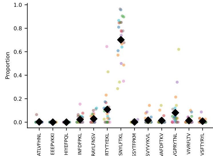
#196 AV7D-5-CAVSMTNSAGNKLTFF-AJ17_BV3-CASSLSTGNSDYTF-BJ1-2 coh=0.850, n=27
