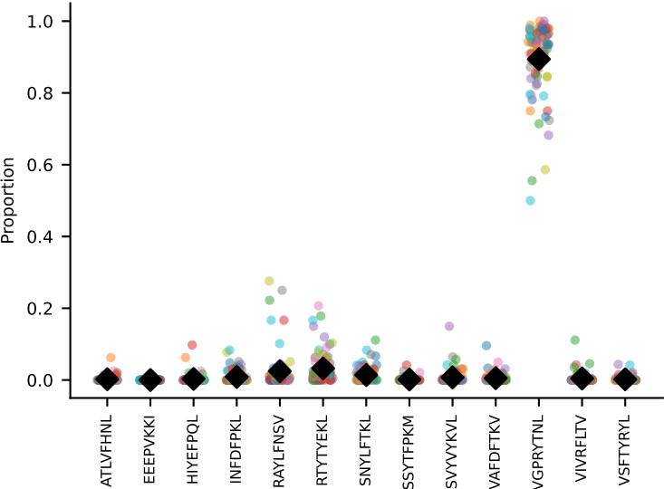
#80 AV17-CALGNNAGAKLTf-AJ39_BV13-1-CASSILGGSYEYF-BJ2-7 coh=0.985, n=15
