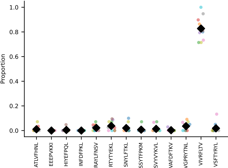
#82 AV6D-7-CALGDDSGYNKLTf-AJ11_BV3-CASSLGTVSYEYF-BJ2-7 coh=0.985, n=5
