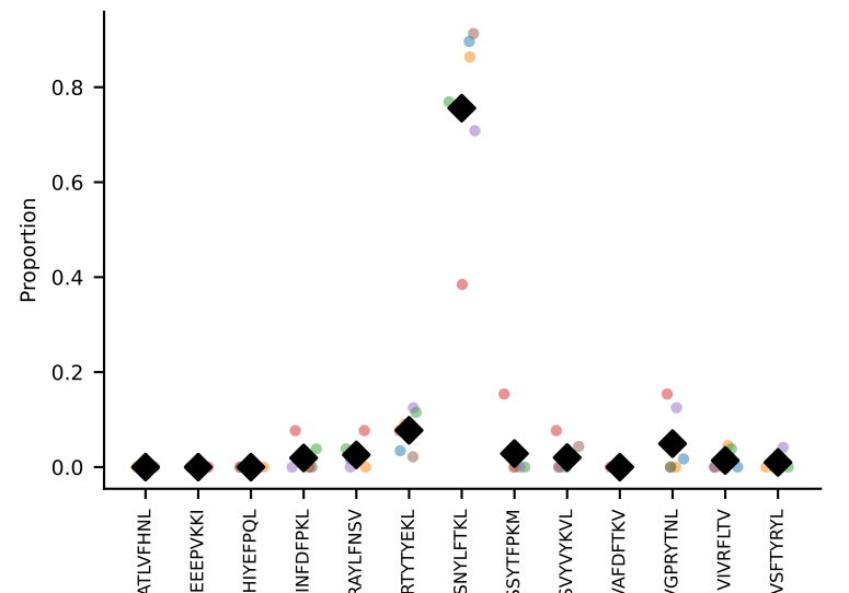
#395 AV16N-CAMREGSSGSQWLIF-AJ22_BV13-2-CASGVQGSATLYF-BJ1-5 coh=0.940, n=5
