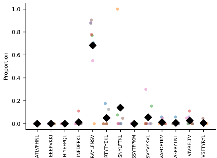
#421 AV10D-CAASWDTNAYKVIF-AJ30_BV13-2-CASGEQTEVFF-BJ1-1 coh=0.696, n=11
