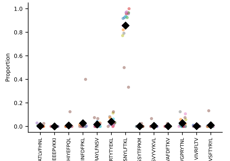
#284 AV16N-CAMRDDSGYNKLTFF-AJ11_BV13-2-CASGDAGTGVDSDYTF-BJ1-5 coh=0.941, n=6
