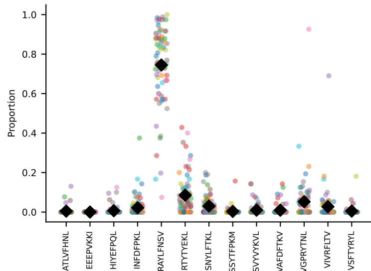
#191 AV7D-3-CAVTGNKYKYF-AJ40_BV13-2-CASGDQGASGNTLYF-BJ1-3 coh=0.875, n=16
