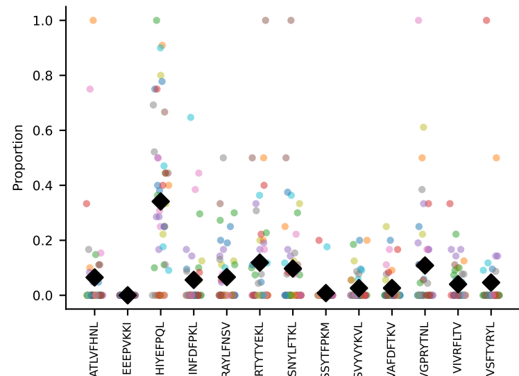
#454 AV3-3-CAVRNNAAGAKLTF-AJ39_BV19-CASSRLGLYEQYF-BJ2-7 coh=0.388, n=6
