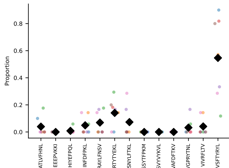
#223 AV6-5-CALSDHAGYQNFYF-AJ49_BV13-2-CASGARTGENYAEQFF-BJ2-1 coh=0.689, n=194
