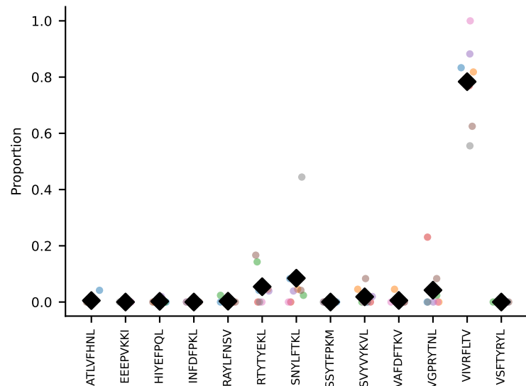
#295 AV13D-2-CAIDTNAYKVF-AJ30_BV3-CASSLDWSSYEQYF-BJ2-7 coh=0.927, n=20
