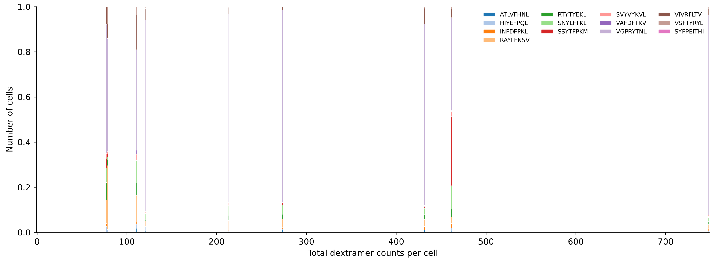
BALBc_HIL Combined | #112 AV6D-7-CALRYGGSGNKLIF-AJ32_BV3-CASSLGTDGTQYF-BJ2-5 (n=9) Total pMHC histogram — stacked by mean peptide proportion per bin [112/228]
