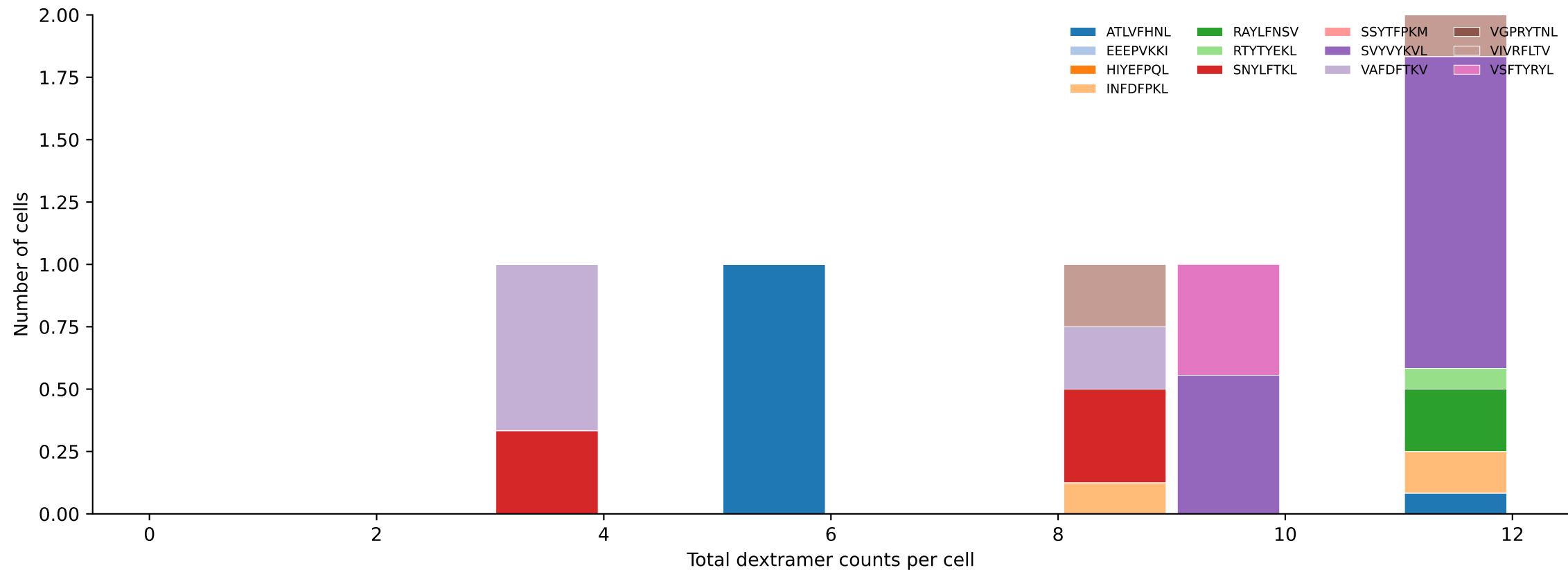
D7ABC_LL Combined | #314 AV14D-1-CAASAGGSAKLIF-AJ57_BV12-2-CASSLGQGAGAEQFF-BJ2-1 (n=6) Total pMHC histogram — stacked by mean peptide proportion per bin [314/392]
