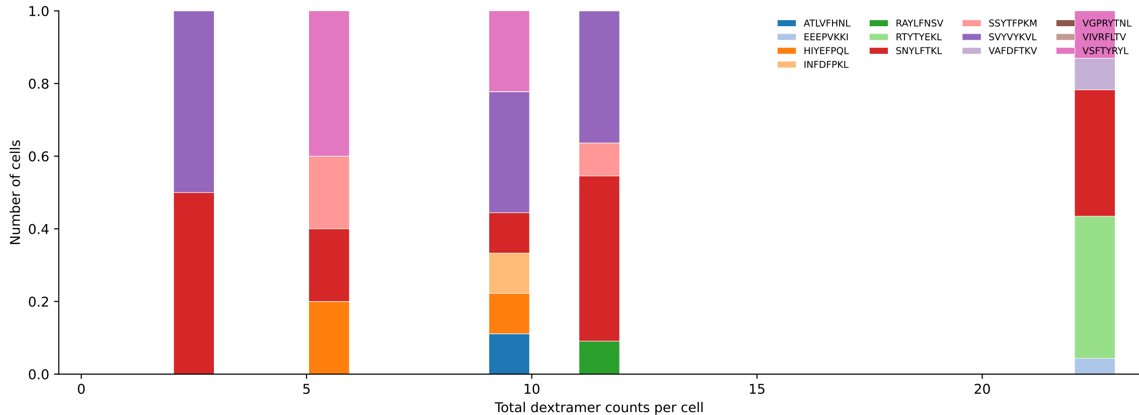
D7ABC_LL Combined | #226 AV19-CAAGAAGNTGKLIF-AJ37_BV26-CASSLSKVNQDTQYF-BJ2-5 (n=5) Total pMHC histogram — stacked by mean peptide proportion per bin [226/392]
