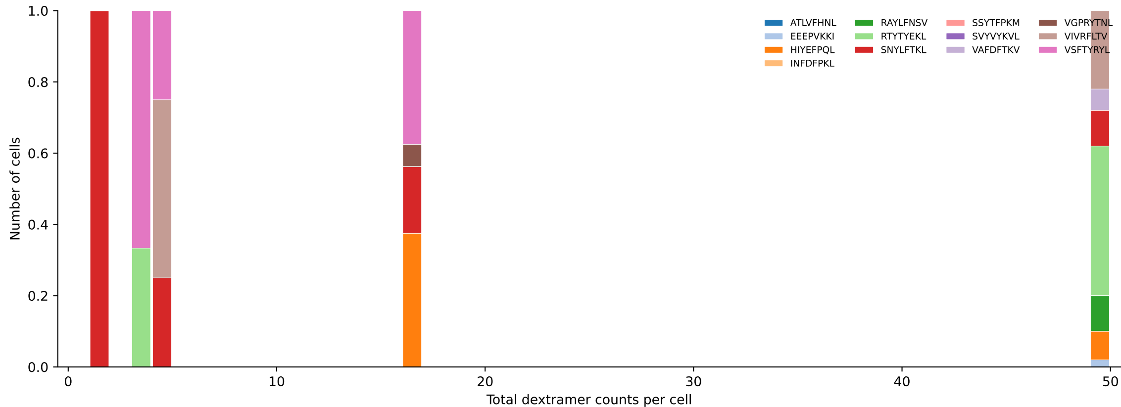
D7ABC_LL Combined | #268 AV9D-3-CAVSMQGGSAKLIF-AJ57_BV13-3-CASRDRGRDTQYF-BJ2-5 (n=5) Total pMHC histogram — stacked by mean peptide proportion per bin [268/392]
