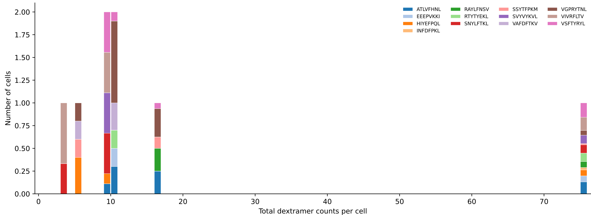
D7ABC_LL Combined | #310 AV3D-3-CAVSERSNYNVLYF-AJ21_BV5-CASSQGQGYAEQFF-BJ2-1 (n=8) Total pMHC histogram — stacked by mean peptide proportion per bin [310/392]
