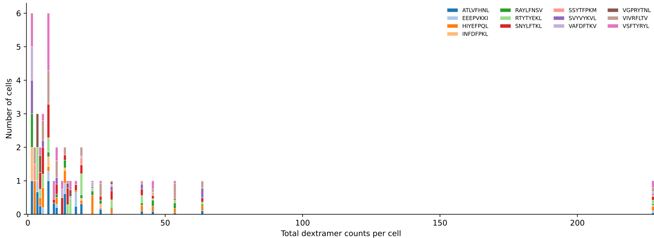
D7ABC_LL Combined | #95 AV14-2-CAAGASSGSWQLIF-AJ22_BV31-CAWSLAGSGNTLYF-BJ1-3 (n=41) Total pMHC histogram — stacked by mean peptide proportion per bin [95/392]
