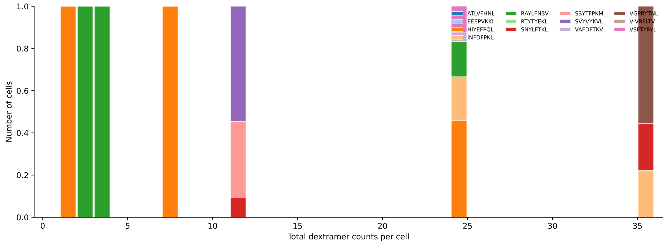
D7ABC_LL Combined | #328 AV14-2-CAASGNYNVLYF-AJ21_BV3-CASSLDWGGSEYQYF-BJ2-7 (n=7) Total pMHC histogram — stacked by mean peptide proportion per bin [328/392]
