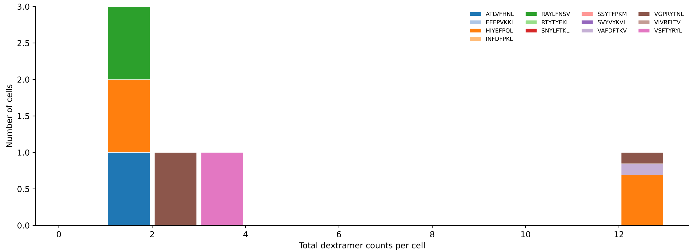
D7ABC_LL Combined | #389 AV16-CAMREGGGASSSFSLVF-AJ50_BV16-CASSSGQYEQYF-BJ2-7 (n=6) Total pMHC histogram — stacked by mean peptide proportion per bin [389/392]
