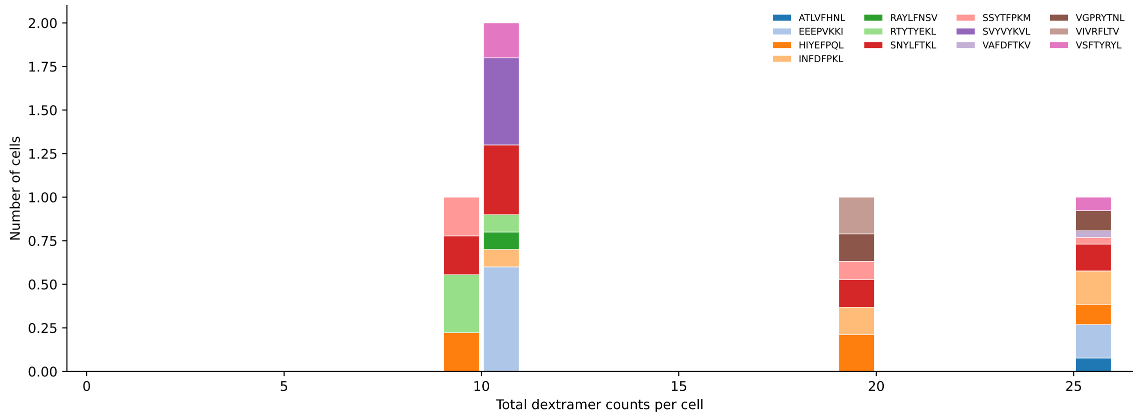
D7ABC_LL Combined | #66 AV16/DV11-CAMREVDTNAYKVIF-AJ30_BV13-1-CASSDGLNSDYTF-BJ1-2 (n=5) Total pMHC histogram — stacked by mean peptide proportion per bin [66/392]
