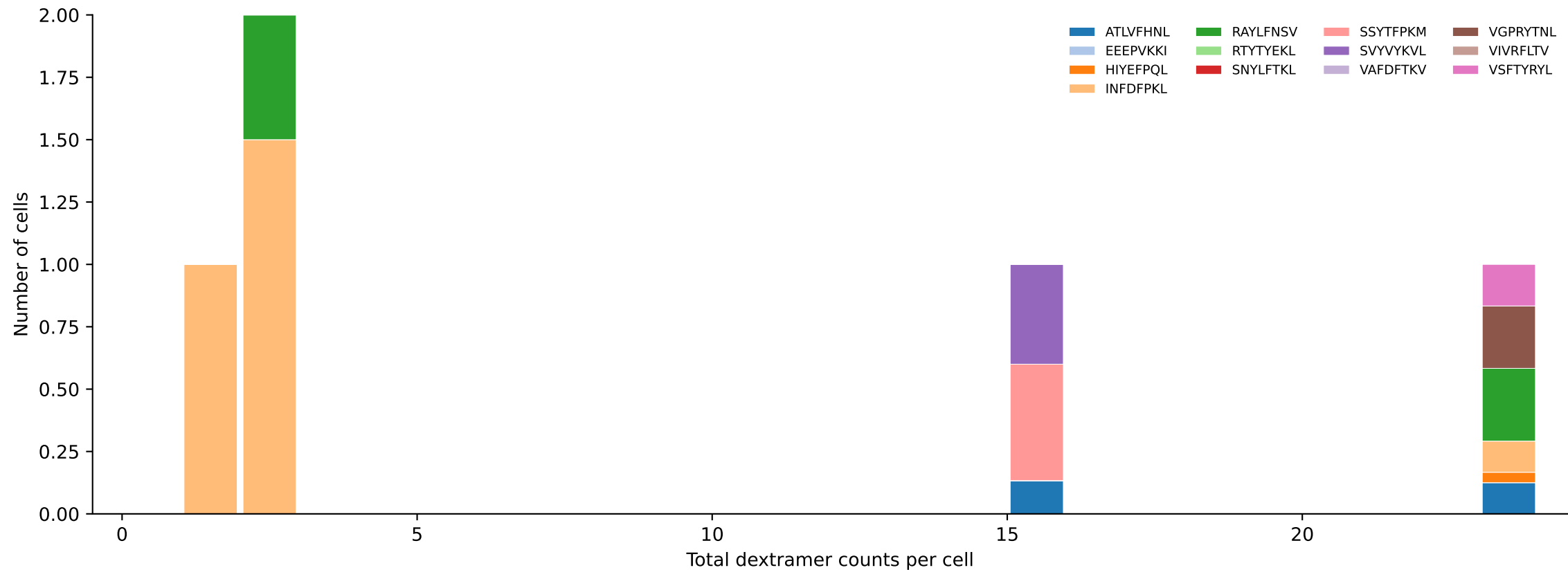
D7ABC_LL Combined | #255 AV19-CAAGVGDNSKLIW-AJ38_BV14-CASRYRDTQYF-BJ2-5 (n=5) Total pMHC histogram — stacked by mean peptide proportion per bin [255/392]
