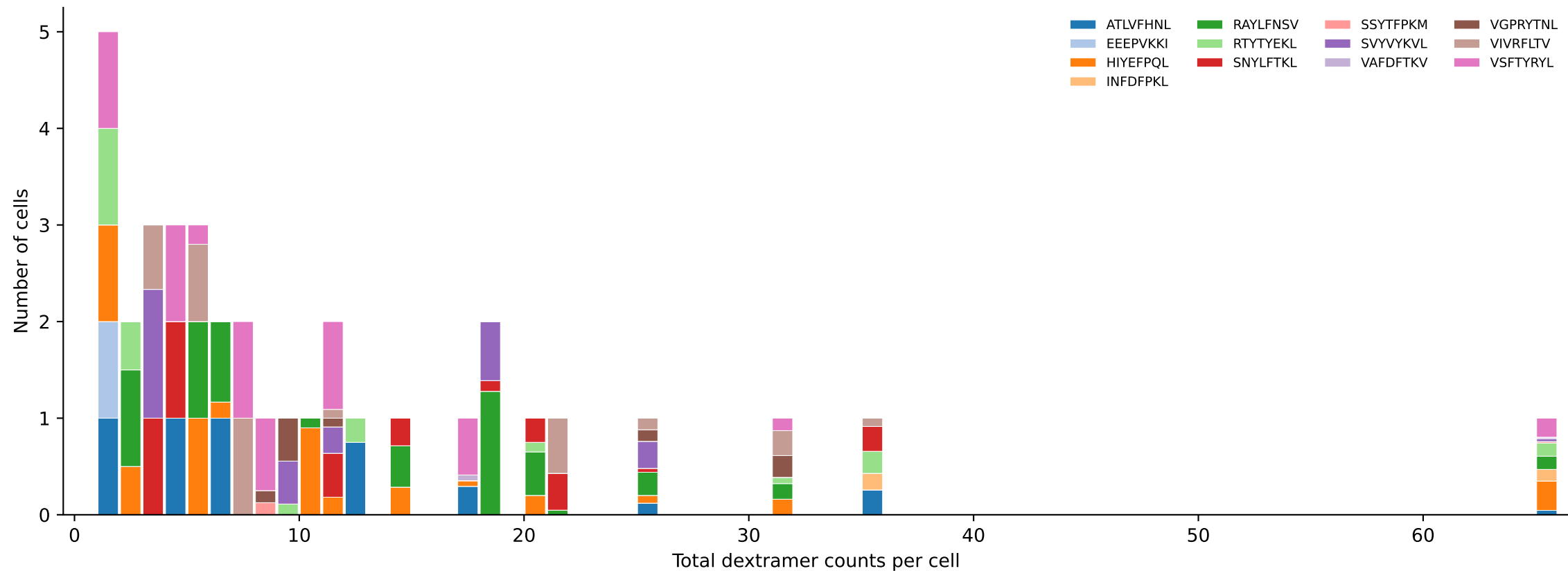
D7ABC_LL Combined | #353 AV9-2-CVLSVTGSGGKLT-AJ44_BV14-CASSFANTGQLYF-BJ2-2 (n=36) Total pMHC histogram — stacked by mean peptide proportion per bin [353/392]
