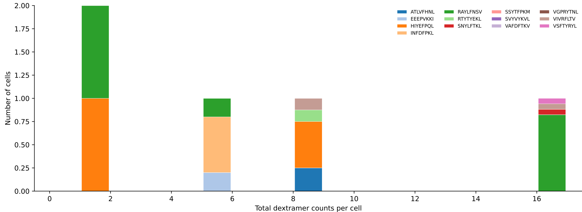
D7ABC_LL Combined | #101 AV14-2-CAADSNYQLIW-AJ33_BV13-1-CASSEVGGQDTQYF-BJ2-5 (n=5) Total pMHC histogram — stacked by mean peptide proportion per bin [101/392]
