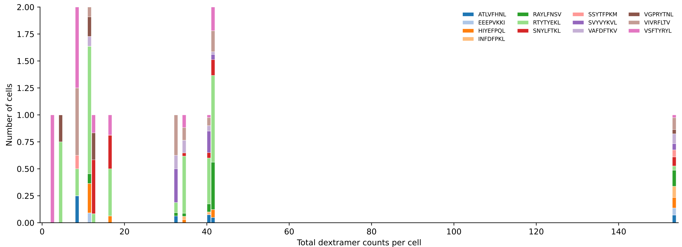
D7ABC_LL Combined | #39 AV6-6-CALGESGGSNAKLTF-AJ42_BV13-3-CASSDAQTYNSPLYF-BJ1-6 (n=14) Total pMHC histogram — stacked by mean peptide proportion per bin [39/392]
