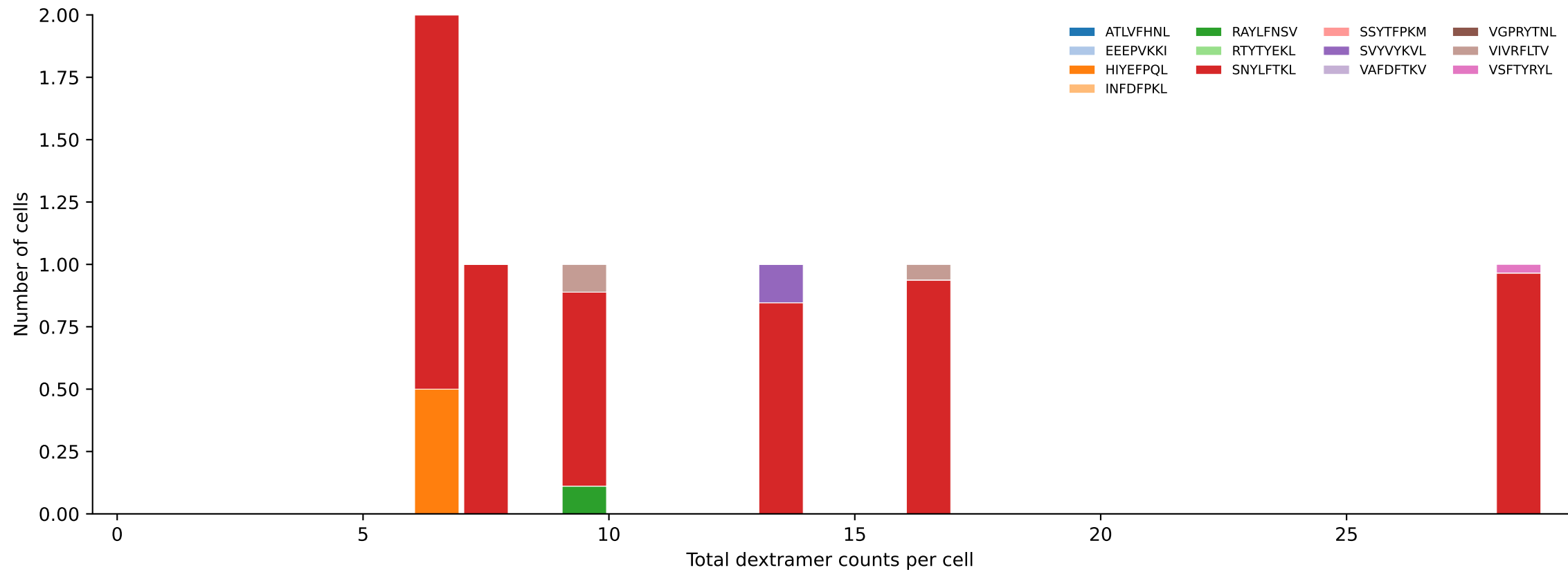
D7ABC_LL Combined | #3 AV13D-1-CAMETSNYNVLYF-AJ21_BV13-3-CASSDRDEQFF-BJ2-1 (n=7) Total pMHC histogram — stacked by mean peptide proportion per bin [3/392]
