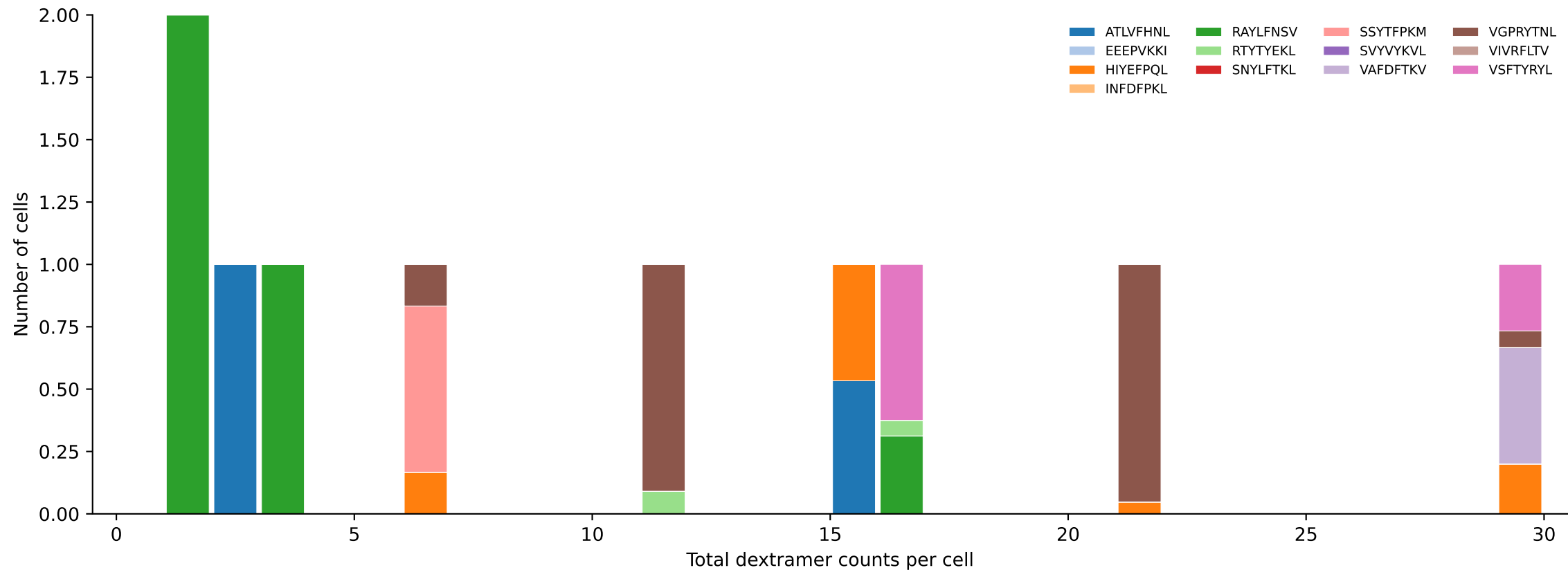
D7ABC_LL Combined | #354 AV8D-2-CATDGQGGRALIF-AJ15_BV3-CASSPQGHSDYTF-BJ1-2 (n=10) Total pMHC histogram — stacked by mean peptide proportion per bin [354/392]
