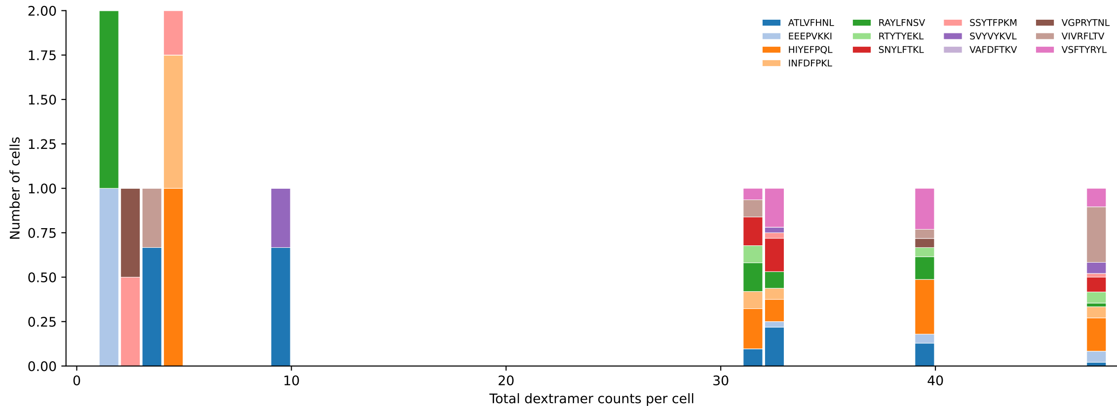
D7ABC_LL Combined | #124 AV14-2-CAASGTGYQNFYF-AJ49_BV2-CASSQAWGNQDTQYF-BJ2-5 (n=11) Total pMHC histogram — stacked by mean peptide proportion per bin [124/392]
