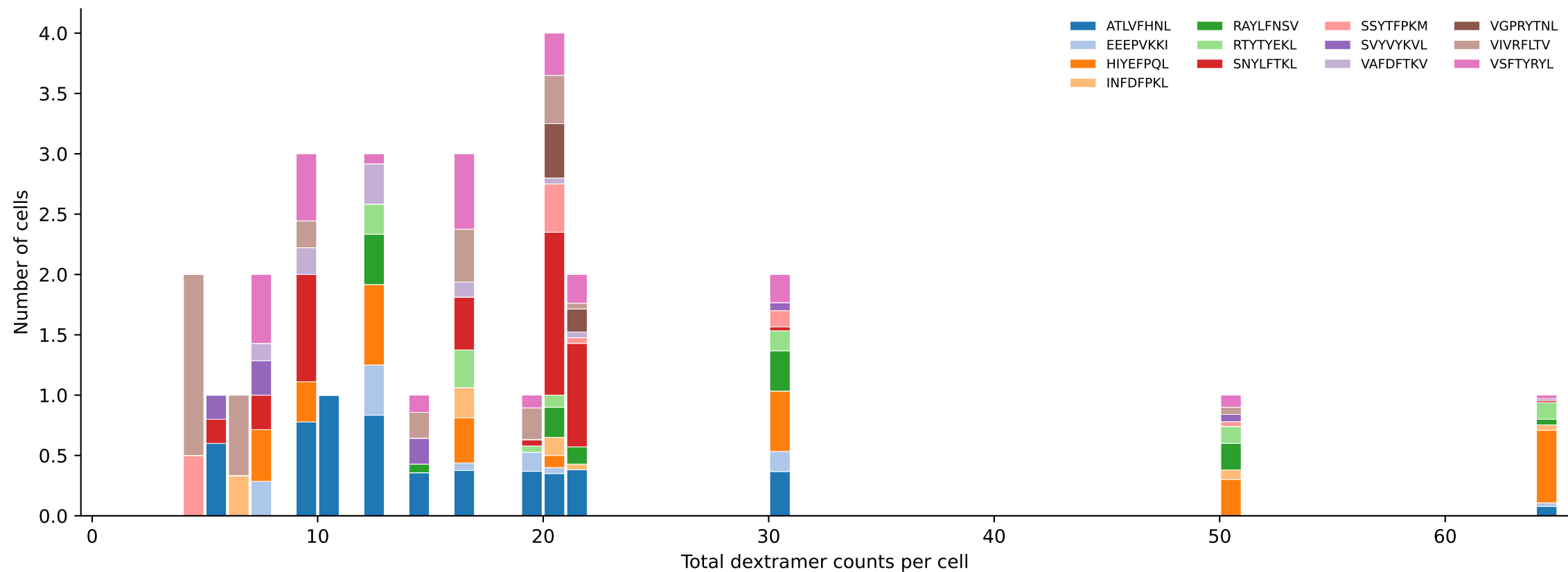
D7ABC_LL Combined | #64 AV6-4-CALVESGGSNAKLTF-AJ42_BV19-CASSMGVGNTEVFF-BJ1-1 (n=28) Total pMHC histogram — stacked by mean peptide proportion per bin [64/392]
