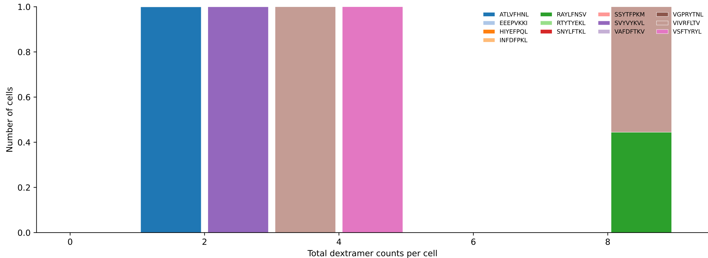
D7ABC_LL Combined | #388 AV10-CAASGDTNAYKVIF-AJ30_BV3-CASSLVRHPNSDYTF-BJ1-2 (n=5) Total pMHC histogram — stacked by mean peptide proportion per bin [388/392]
