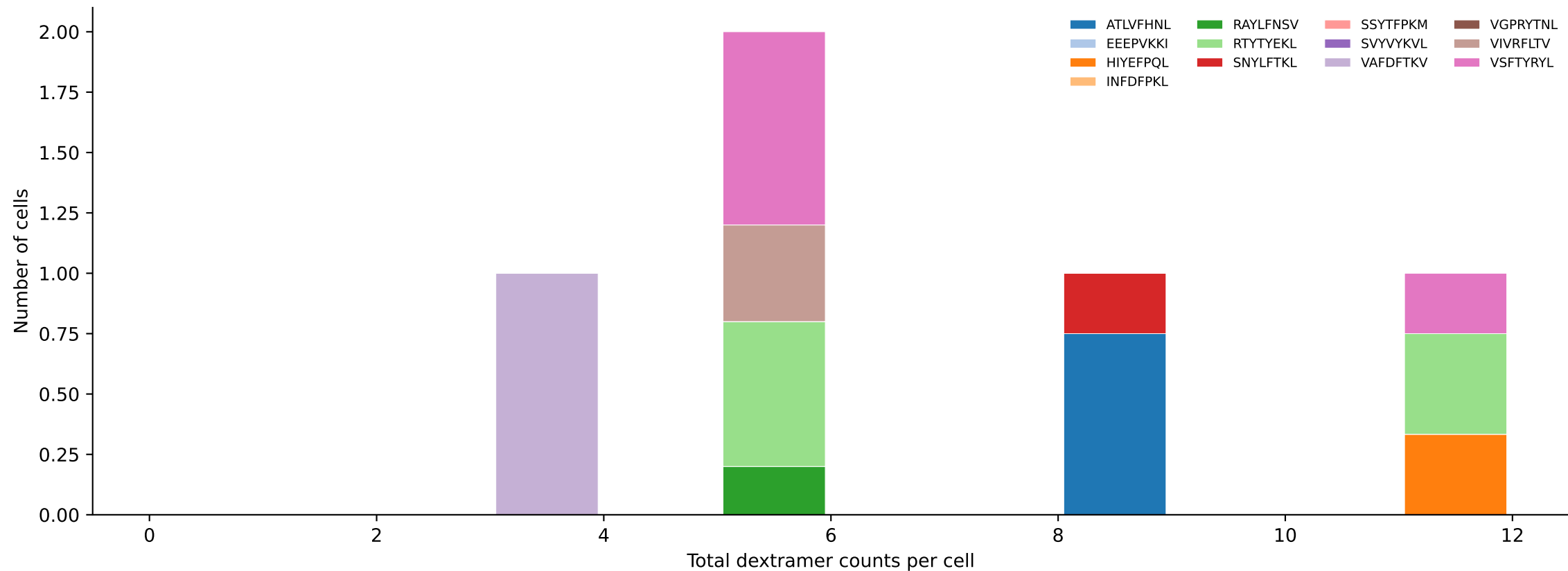
D7ABC_LL Combined | #385 AV14-2-CAASLASSGSWQLIF-AJ22_BV26-CASSWTGGAETLYF-BJ2-3 (n=5) Total pMHC histogram — stacked by mean peptide proportion per bin [385/392]
