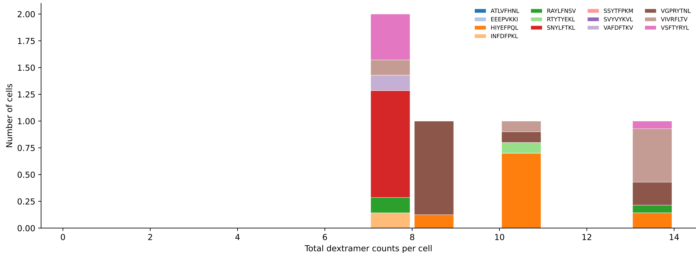
D7ABC_LL Combined | #330 AV8D-2-CATDGNSNNRIFF-AJ31_BV3-CASSIRDWEYEQYF-BJ2-7 (n=5) Total pMHC histogram — stacked by mean peptide proportion per bin [330/392]
