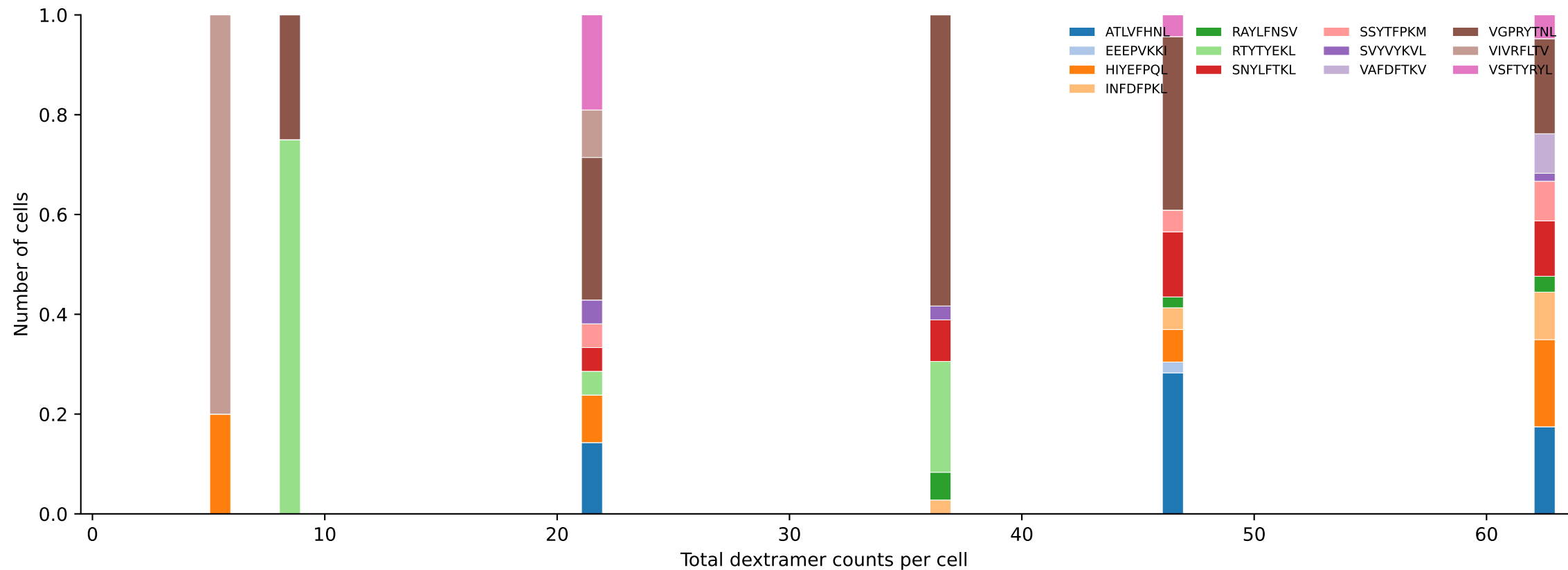
D7ABC_LL Combined | #180 AV12-1-CALRDYSNNRLTL-AJ7_BV3-CASSPGVDTQYF-BJ2-5 (n=6) Total pMHC histogram — stacked by mean peptide proportion per bin [180/392]
