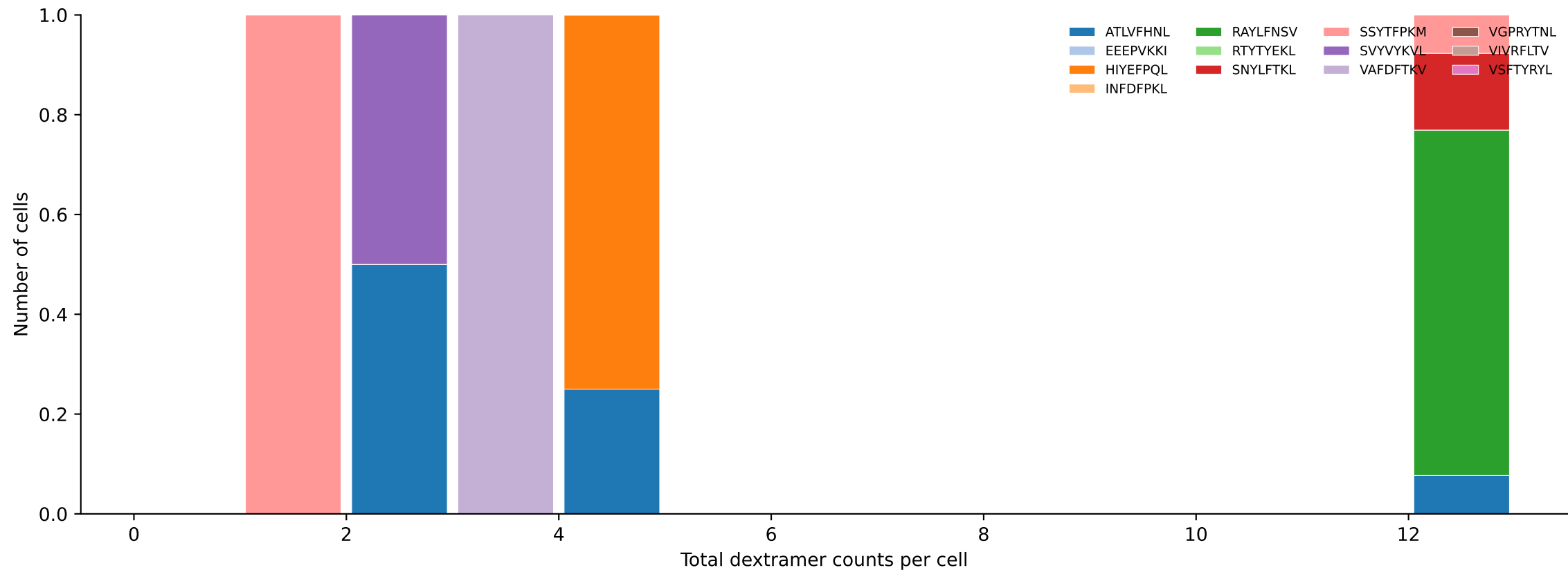
D7ABC_LL Combined | #392 AV16N-CAMREGDSNYQLIW-AJ33_BV13-2-CASGEAPSAETLYF-BJ2-3 (n=5) Total pMHC histogram — stacked by mean peptide proportion per bin [392/392]
