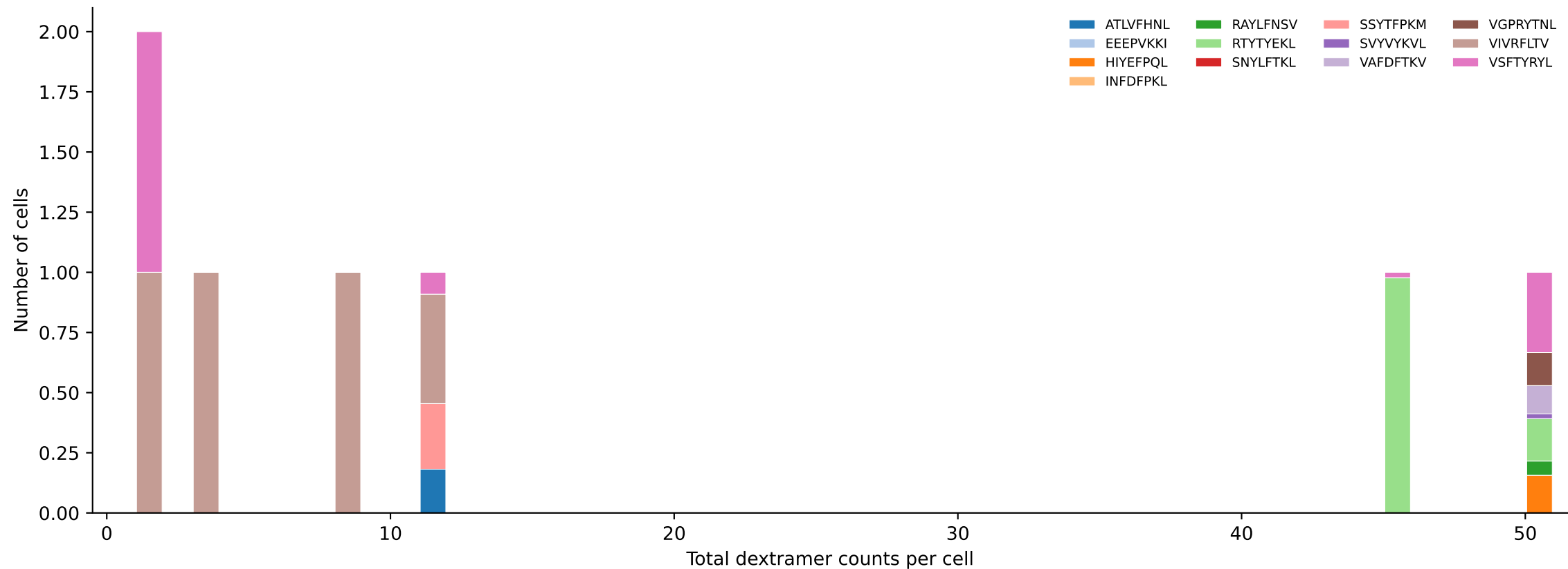
D7ABC_LL Combined | #269 AV8-1-CATDGGGRALIF-AJ15_BV3-CASSSTGVDAEQFF-BJ2-1 (n=7) Total pMHC histogram — stacked by mean peptide proportion per bin [269/392]
