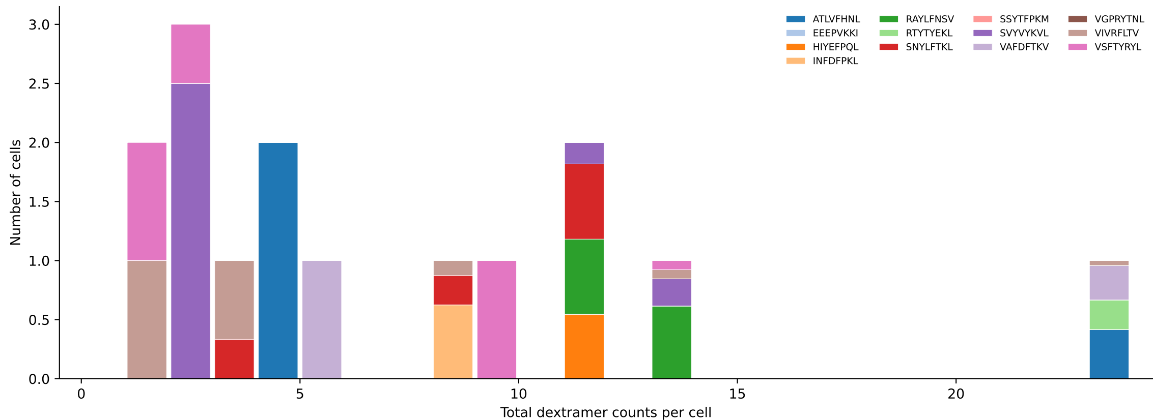
D7ABC_LL Combined | #376 AV14D-1-CAASSAGNTGKLIF-AJ37_BV31-CAWSARGSGNTLYF-BJ1-3 (n=15) Total pMHC histogram — stacked by mean peptide proportion per bin [376/392]
