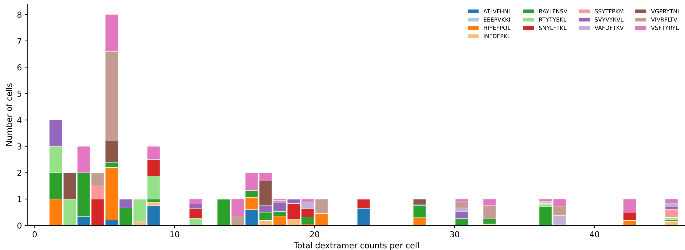
D7ABC_LL Combined | #143 AV7-2-CAAGNTGKLIF-AJ37_BV1-CTCSAVRVGYEQYF-BJ2-7 (n=43) Total pMHC histogram — stacked by mean peptide proportion per bin [143/392]
