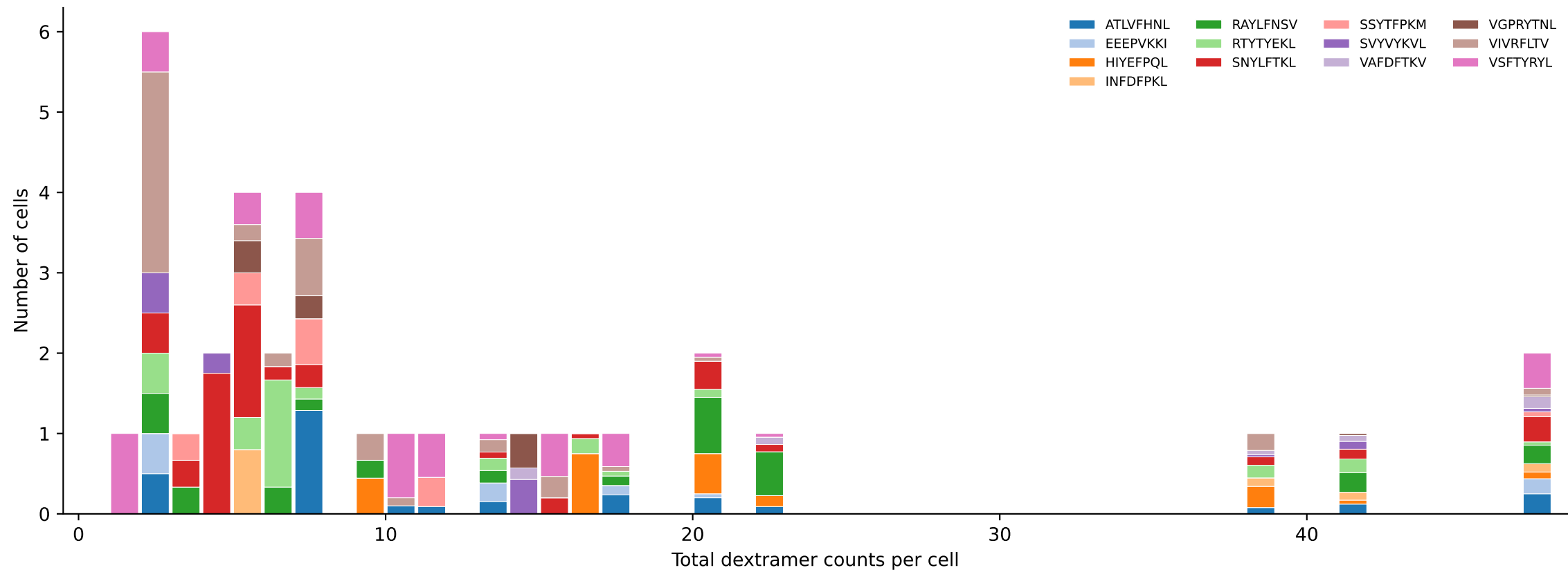
D7ABC_LL Combined | #111 AV16-CAMGTGSGGKLT-AJ44_BV1-CTCSTRGANERLFF-BJ1-4 (n=35) Total pMHC histogram — stacked by mean peptide proportion per bin [111/392]
