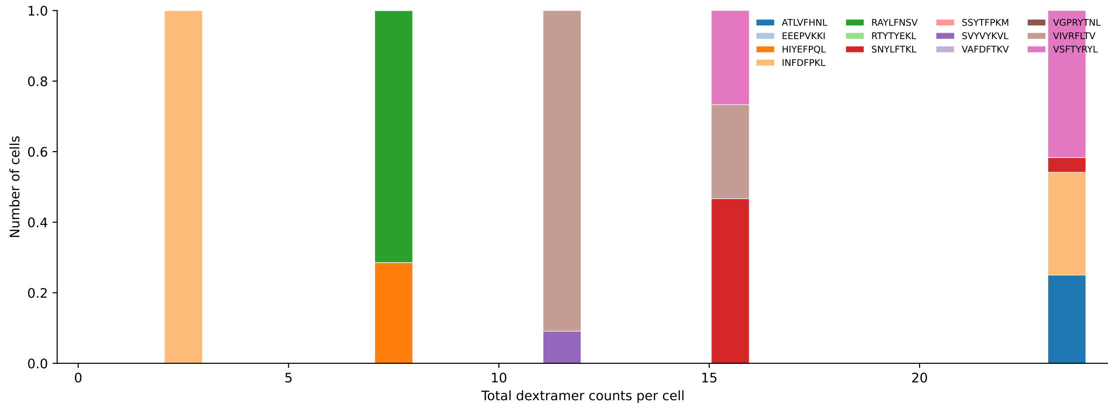
D7ABC_LL Combined | #374 AV3-1-CAVSATGNTGKLIF-AJ37_BV31-CAWDWTNTGQLYF-BJ2-2 (n=5) Total pMHC histogram — stacked by mean peptide proportion per bin [374/392]
