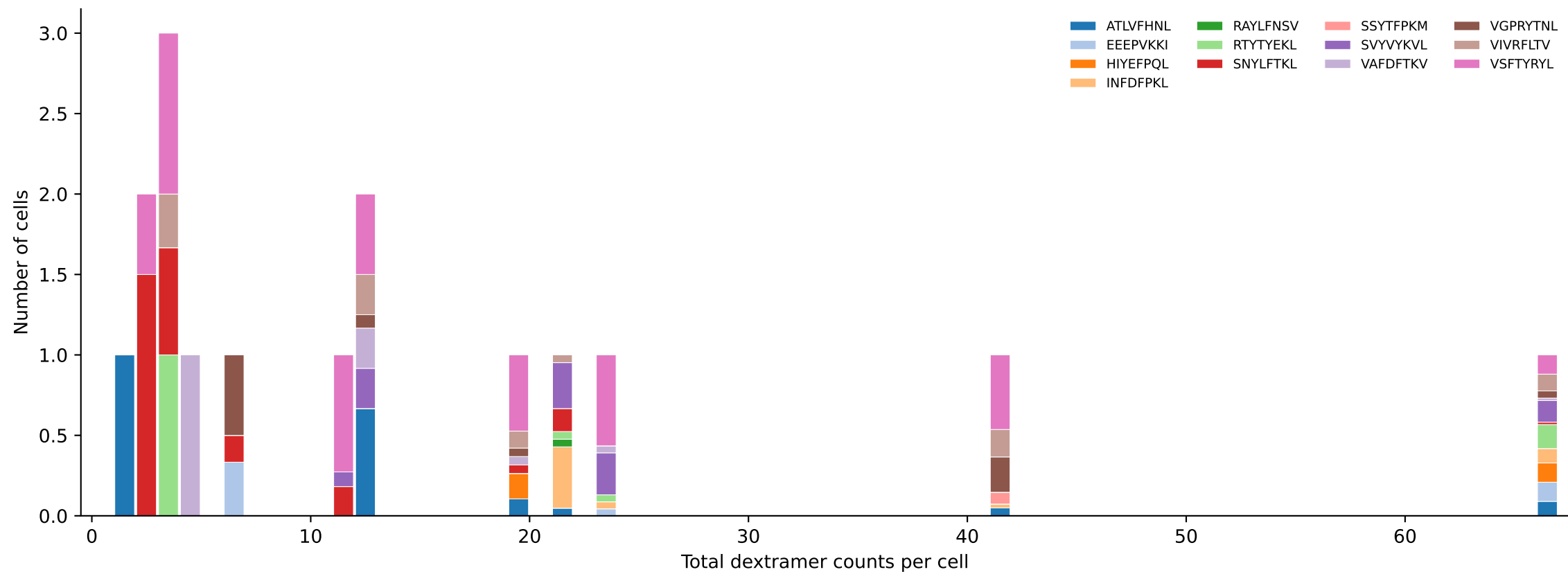
D7ABC_LL Combined | #93 AV14D-3/DV8-CAASASSGSWQLIF-AJ22_BV31-CAWSPLQGANTGVFF-BJ1-1 (n=16) Total pMHC histogram — stacked by mean peptide proportion per bin [93/392]
