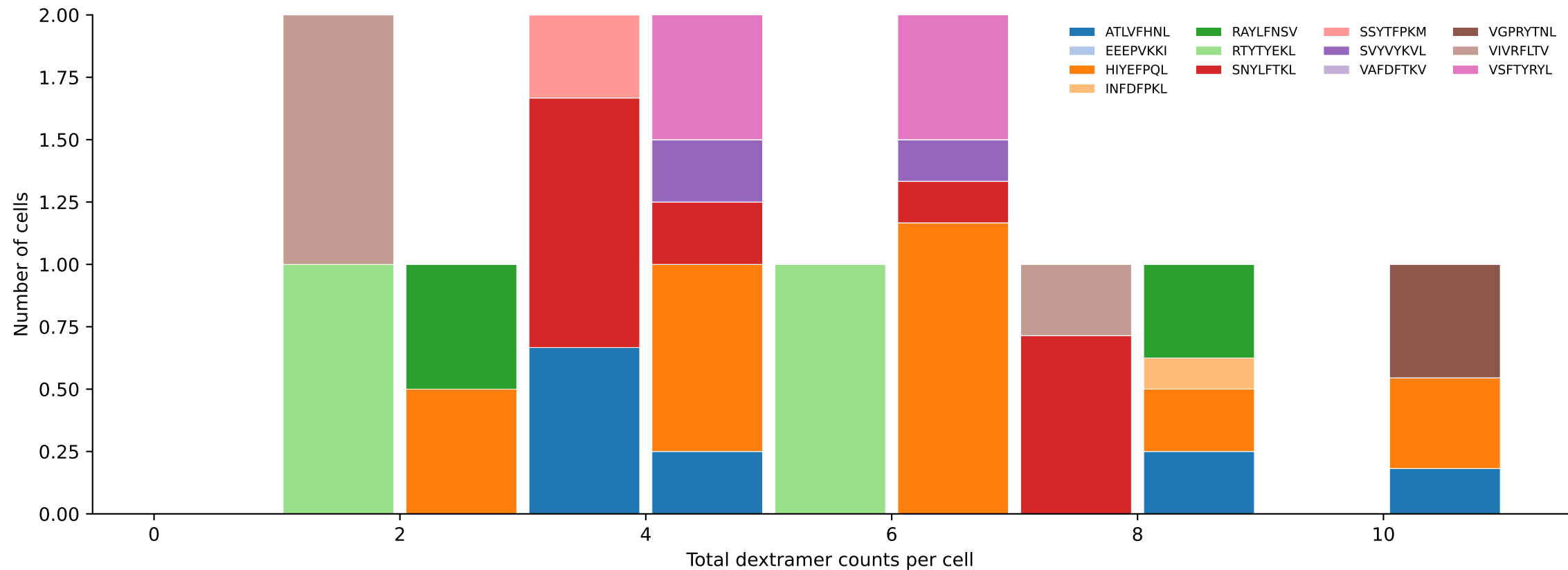
D7ABC_LL Combined | #148 AV10-CAASIDSNYQLIW-AJ33_BV19-CASSPSGTTNTEVFF-BJ1-1 (n=13) Total pMHC histogram — stacked by mean peptide proportion per bin [148/392]
