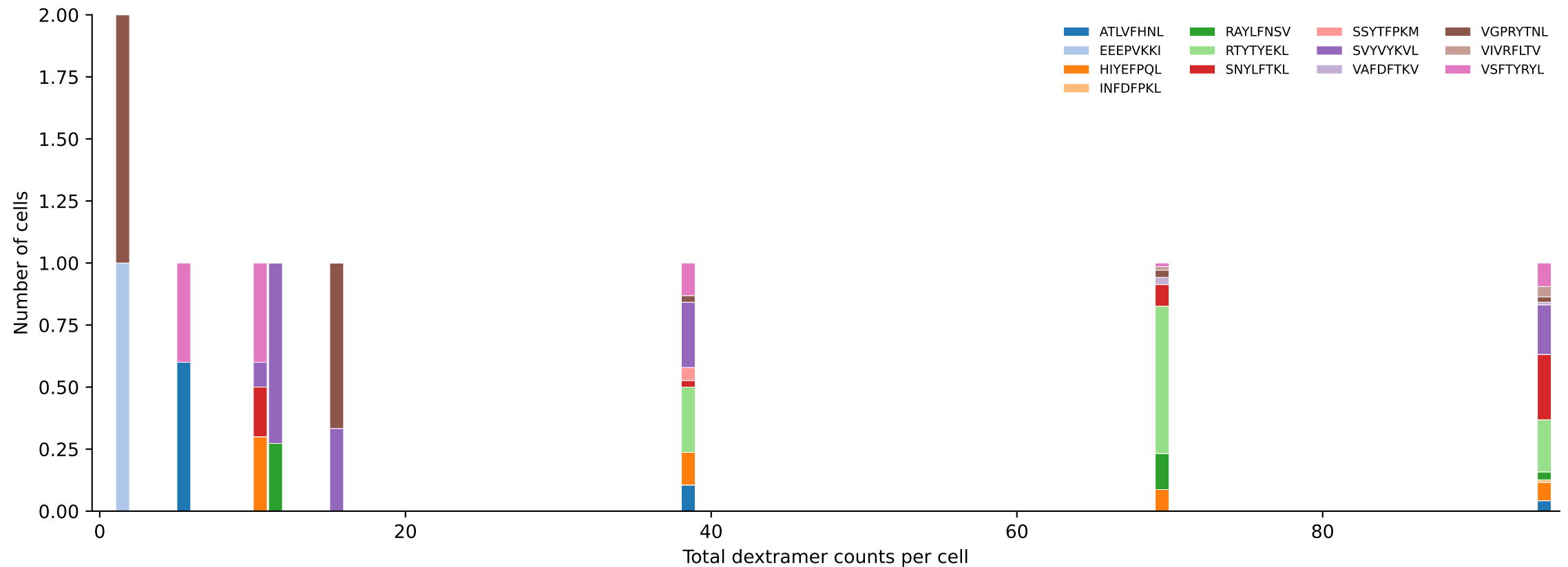
D7ABC_LL Combined | #326 AV16N-CAMREGGSNNRIFF-AJ31_BV13-2-CASGEGPANSDYTF-BJ1-2 (n=9) Total pMHC histogram — stacked by mean peptide proportion per bin [326/392]
