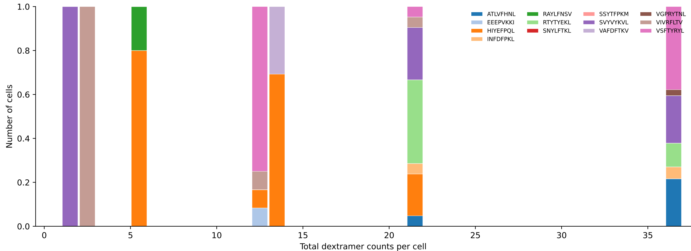
D7ABC_LL Combined | #334 AV7-5-CAVSLDSNYQLIW-AJ33_BV30-CSSWDRTNTGQLYF-BJ2-2 (n=7) Total pMHC histogram — stacked by mean peptide proportion per bin [334/392]
