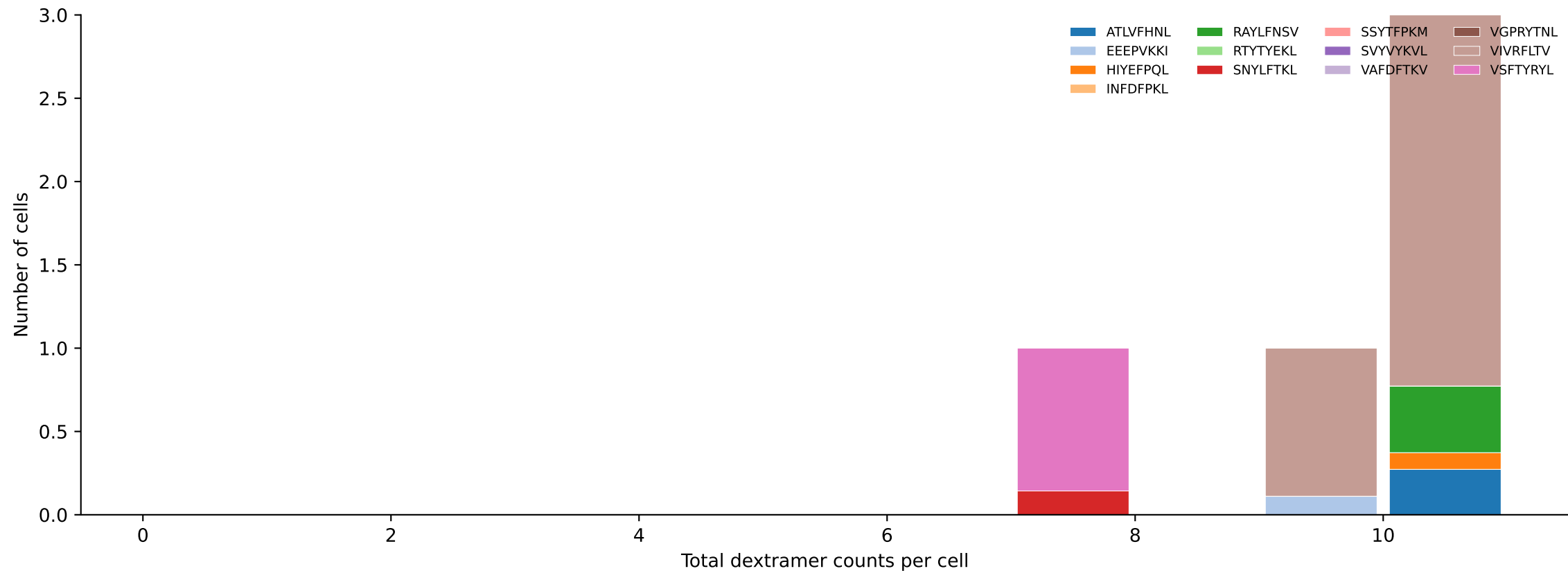
D7ABC_LL Combined | #225 AV13-4/DV7-CAMERDTGYQNFYF-AJ49_BV3-CASSLDWGGYEYF-BJ2-7 (n=5) Total pMHC histogram — stacked by mean peptide proportion per bin [225/392]
