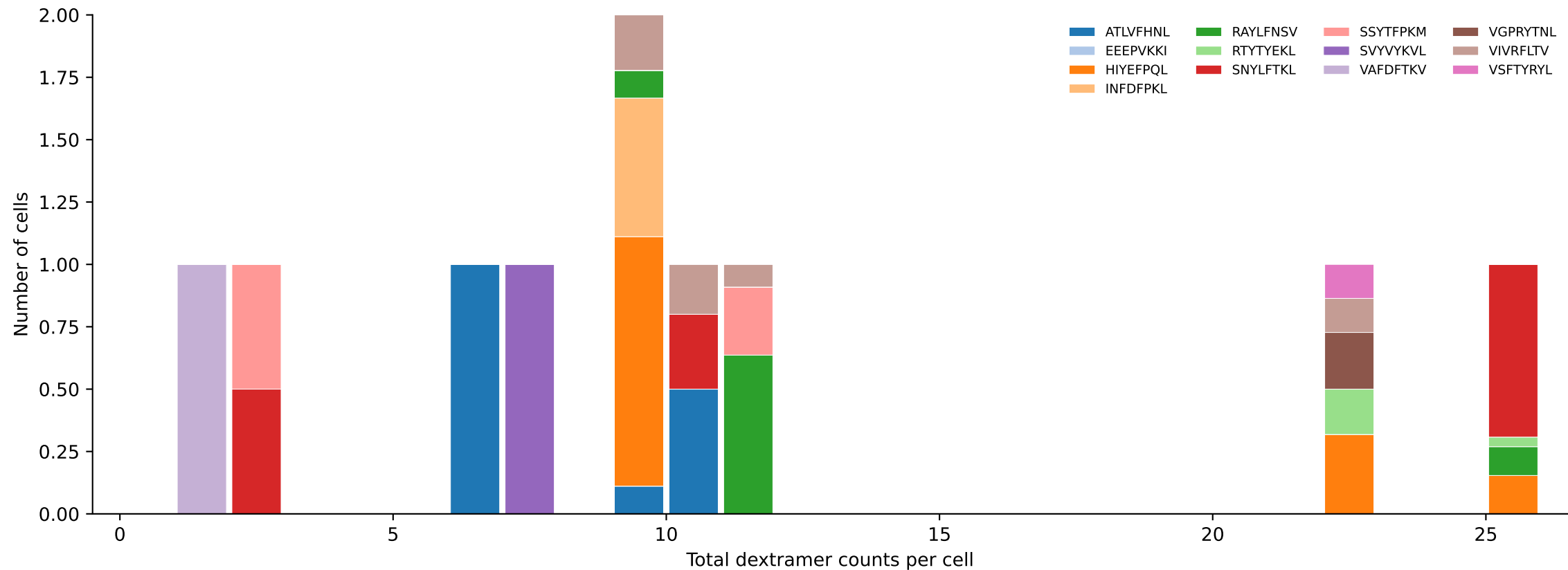
D7ABC_LL Combined | #161 AV19-CAAGVEQQGTGSKLSF-AJ58_BV12-1-CASSLGLNQDTQYF-BJ2-5 (n=10) Total pMHC histogram — stacked by mean peptide proportion per bin [161/392]
