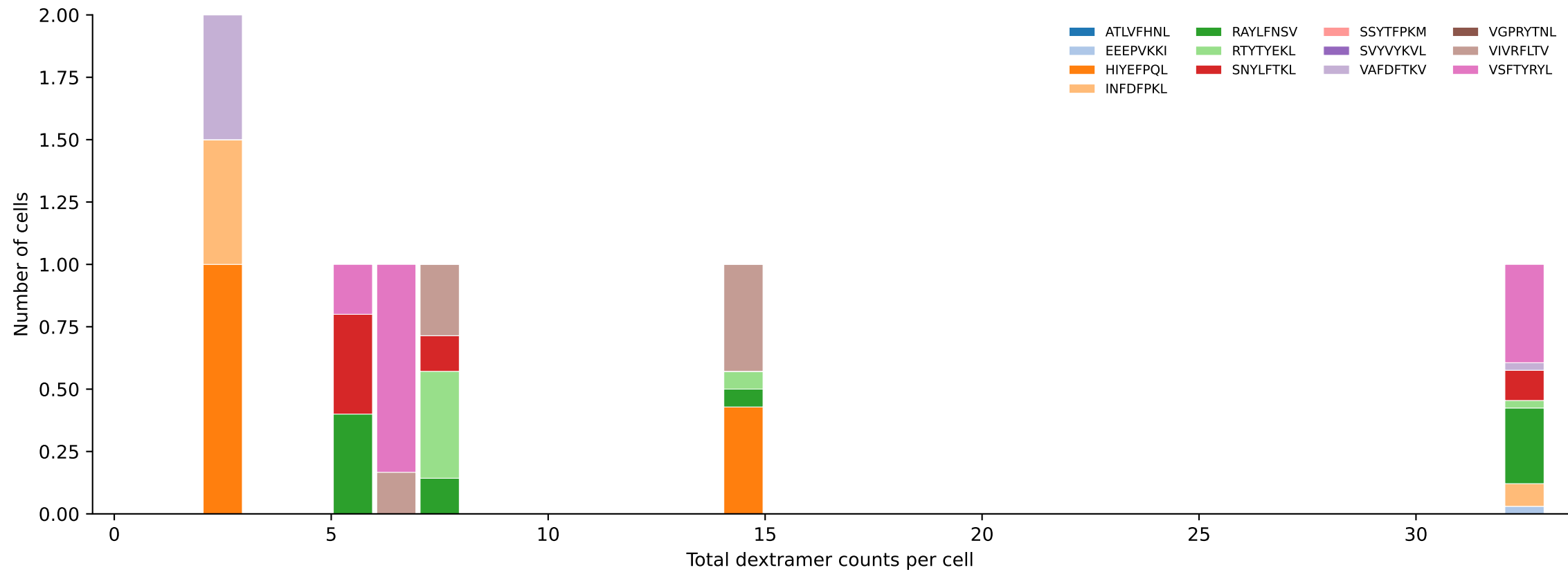
D7ABC_LL Combined | #336 AV6-6-CALGDSGGSNAKLTF-AJ42_BV19-CASSMGLSYNSPLYF-BJ1-6 (n=7) Total pMHC histogram — stacked by mean peptide proportion per bin [336/392]
