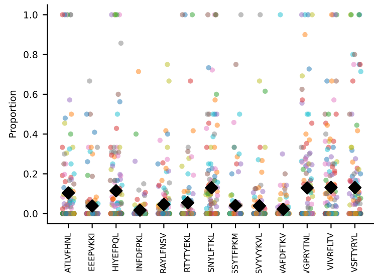
#90 AV17-CALEGSGYGNEKITF-AJ48_BV1-CTCSGDRVSYEQYF-BJ2-7 coh=0.240, n=12
