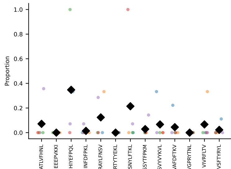
#95 AV16-CAMGTGSGGKLT-L-AJ44_BV1-CTCSTRGANERLFF-BJ1-4 coh=0.230, n=47
