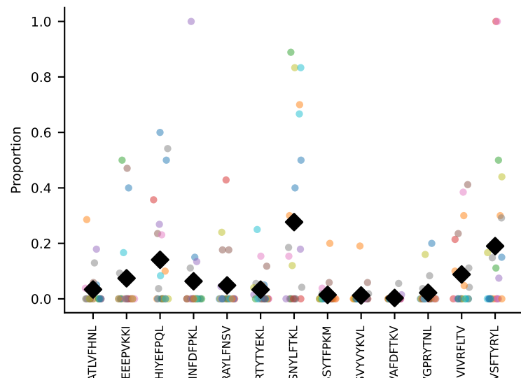
#47 AV12-2-CALSDRGSSSFSLVF-AJ50_BV1-CTCSGTNNQAPLF-BJ1-5 coh=0.319, n=6
