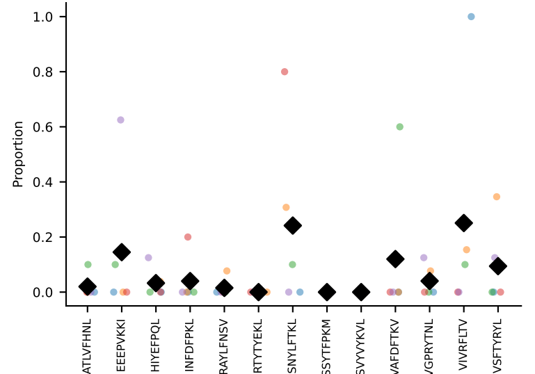
#120 AV3-1-CAVSGQGGRALIF-AJ15_BV13-1-CASRGATAYEQYF-BJ2-7 coh=0.168, n=5
