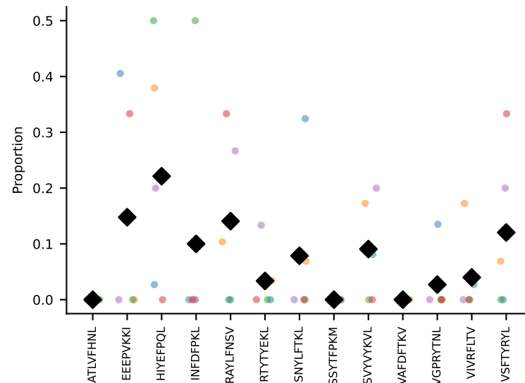
#54 AV12-2-CALRG TGNYKVVF-AJ40_BV1-CTCSASRPYNSPLYF-BJ1-6 coh=0.310, n=8
