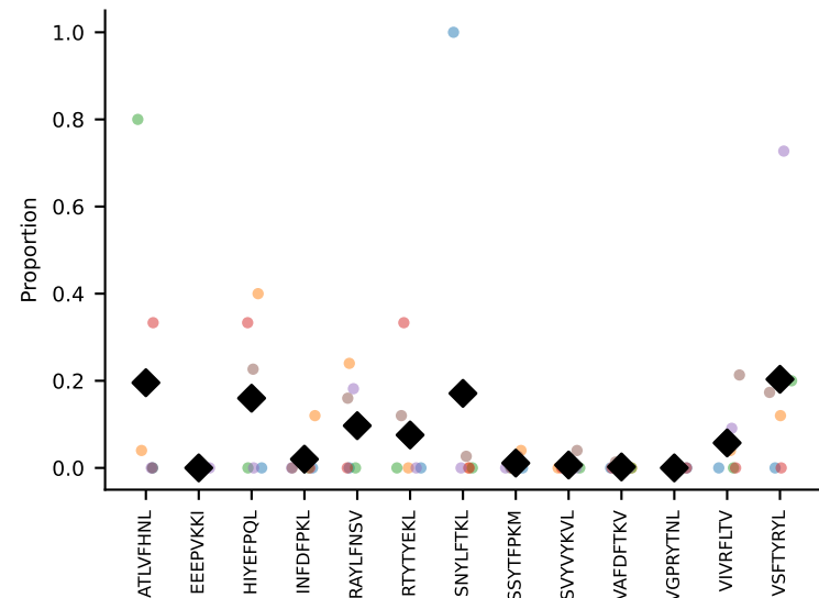
#89 AV16N-CAMREGNNAGAKLTF-AJ39_BV16-CASSSGQKNTEVFF-BJ1-1 coh=0.244, n=83
