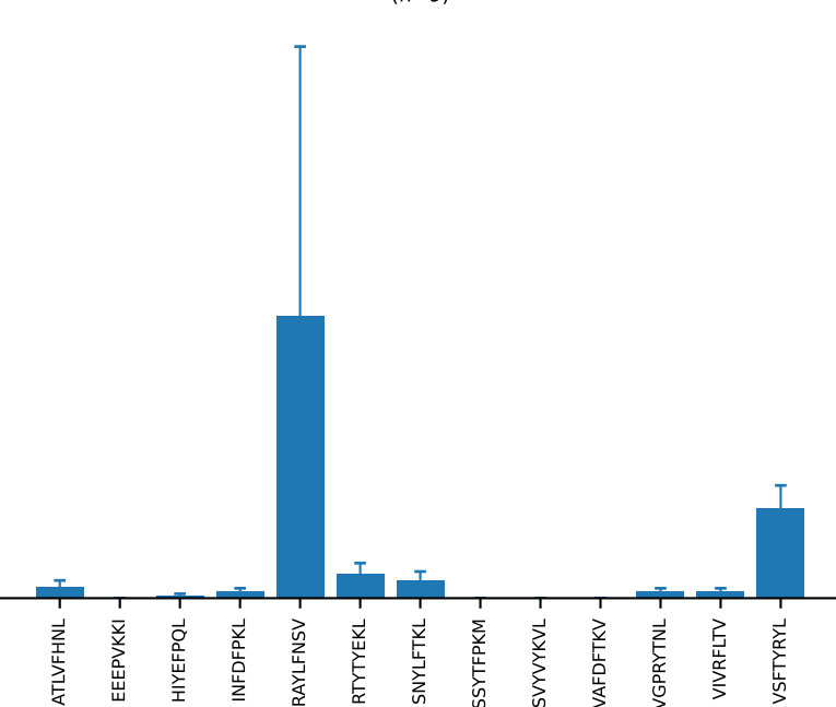
AV9-2-CVLSLNYGSSGNKLIF-AJ32_BV3-CASSPGYAEQFF-BJ2-1 (n=9)
