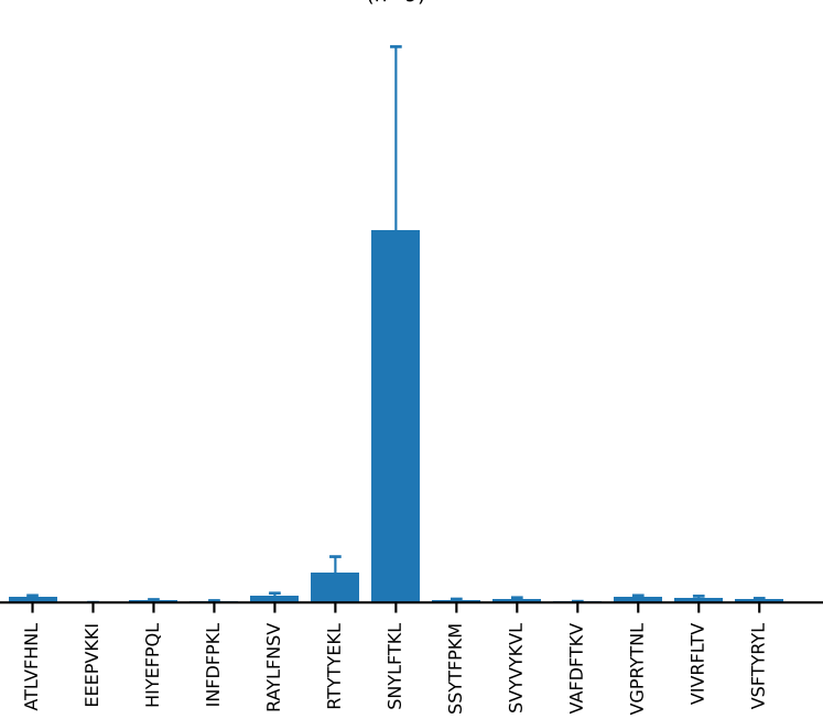
AV4-4/DV10-CAAENTGYQNFYF-AJ49_BV13-3-CASQNTLYF-BJ2-4 (n=9)
