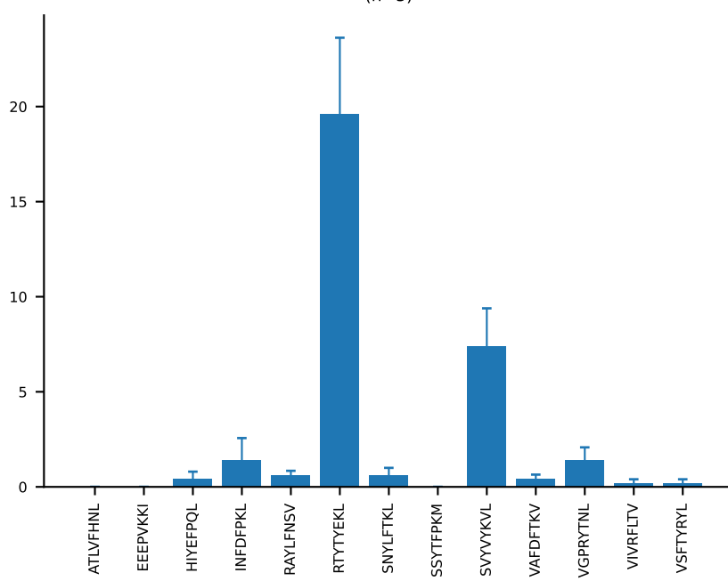
AV9D-3-CALVSNTNKVVF-AJ34_BV13-1-CASSDVNTEVFF-BJ1-1 (n=5)
