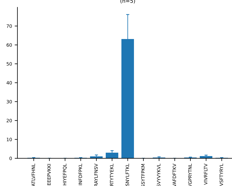
AV7-4-CAASDSSGSWLQIF-AJ22_BV13-1-CASSDAGYEQYF-BJ2-7 (n=5)
