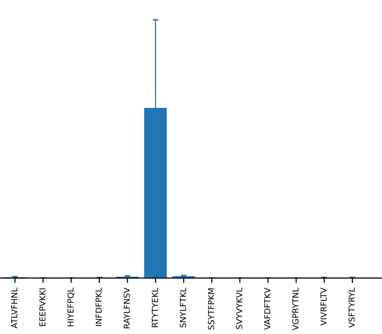
AV16N-CAMREVSNNVLYF-AJ21_BV13-2-CASGDQGSNTLYF-BJ1-3 (n=8)
