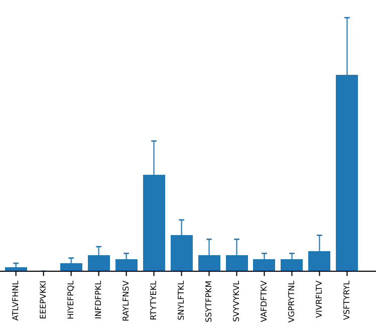
AV7D-3-CAVTGNYKYVF-AJ40_BV17-CASSPGQGYTGQLYF-BJ2-2 (n=8)
