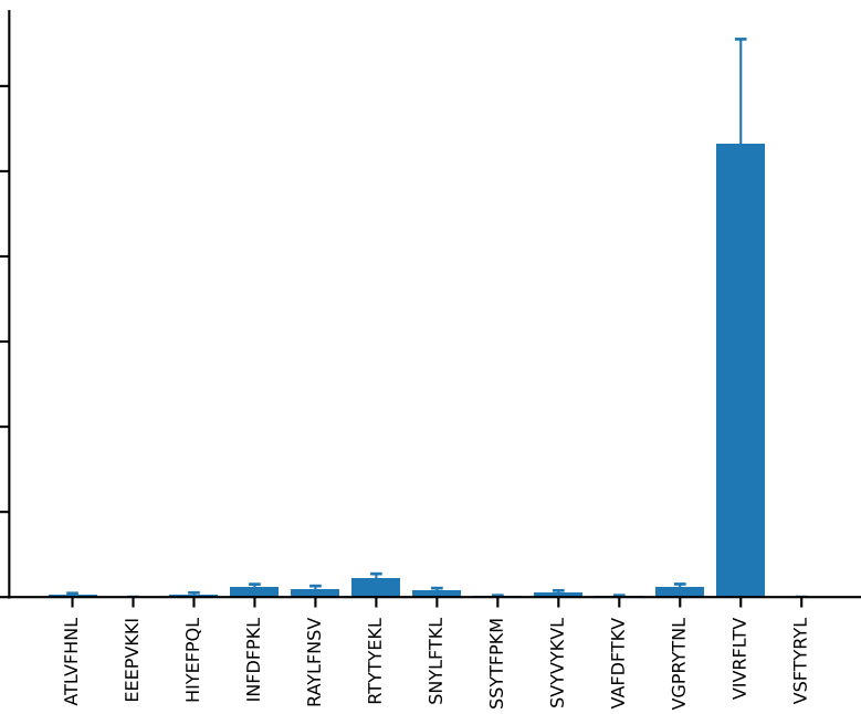
AV16N-CAMREGTGSNRLTF-AJ28_BV1-CTCSPNRVDTLVF-BJ2-4 (n=10)
