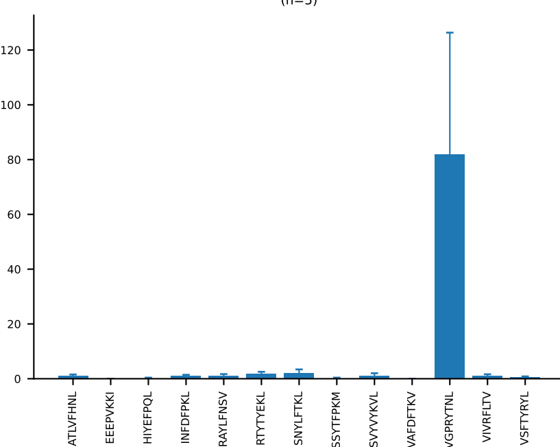
AV7-2-CAASRGDYANKMIF-AJ47_BV13-3-CASSARVEQYF-BJ2-7 (n=5)
