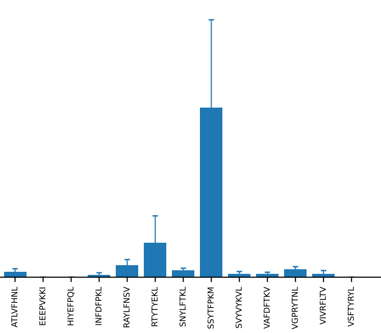
AV13D-1-CAMERSNNRIFF-AJ31_BV2-CASSQDRRGDTQYF-BJ2-5 (n=8)
