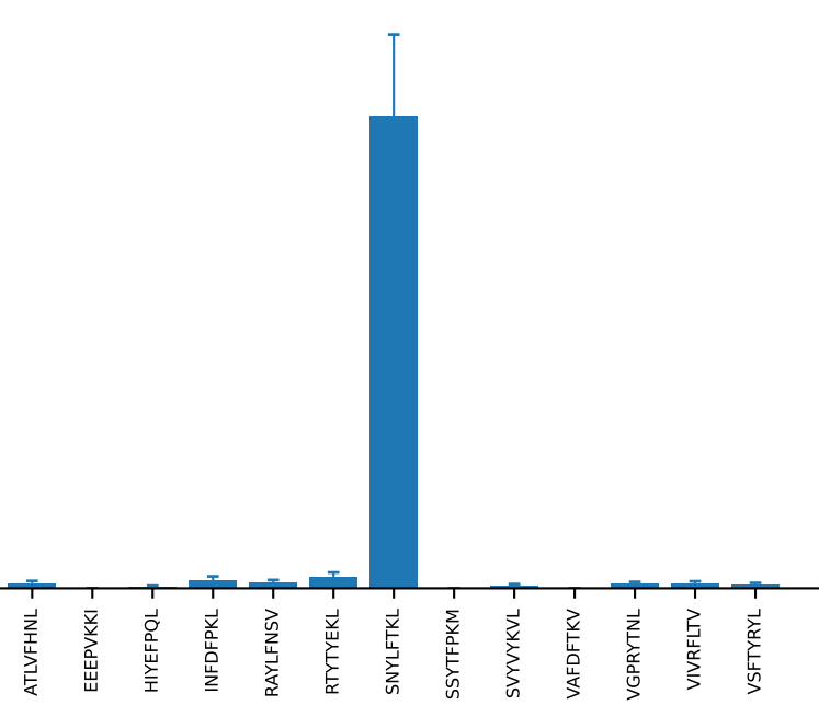
AV7-2-CAASKGGRALIF-AJ15_BV12-2-CASSSGGGISDYTF-BJ1-2 (n=8)
