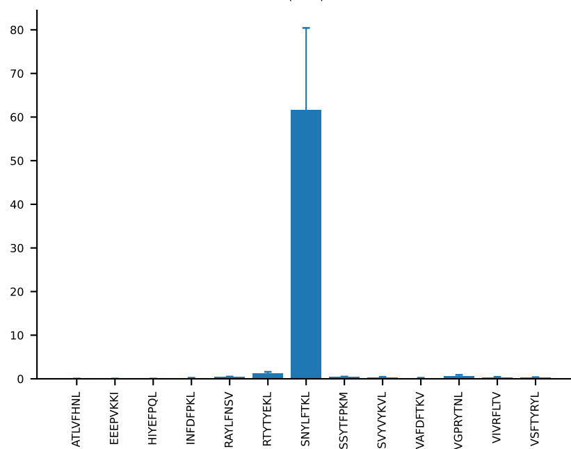
AV13-4/DV7-CAMERGGSNAKLTF-AJ42_BV13-2-CASGEGQGKNTLYF-BJ2-4 (n=9)
