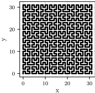
Hilbert curve
