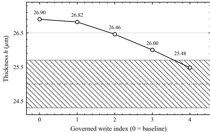
(a) hatched band: target 25.0 \pm 0.7 \mu\text{m}
