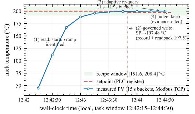
Fig. 6. Real-LLM closed loop on a live Modbus-TCP node (omp/glm-5.3-flash, archive 20260917044223–17h0): measured PV with the recipe window and setpoint step, annotated with the agent’s actions reconstructed from its transcript. The plotted ramp precedes the agent’s start (the line was already sampling); at 12:43:45 both a pre-write (199.32 °C) and a post-write (199.41 °C) reading exist in the trace, and the post-write series is plotted. After the governed write (record opened, readback 197.5 °C), a 1 s-bucket re-query returned a stale window; the agent switched to 15 s buckets before judging the record keep on the post-write series.
