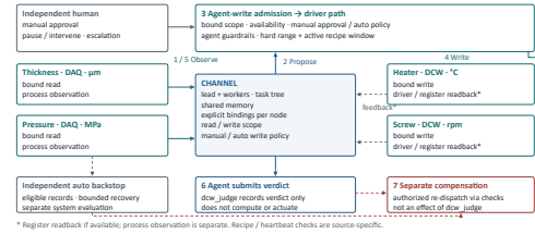
Fig. 3. The mechanisms in their organizational setting and closed loop. Steps 1 and 5 share the observation arrows. The channel coordinates agents that observe bound nodes, propose setpoints, and pass admission checks before write and readback. Step 6 is the agent's own verdict, the independent backstop is a second and separate judgment path, and step 7 is compensation that neither path performs. dcw_judge records a verdict only: it neither computes the conclusion from telemetry nor executes any action.
