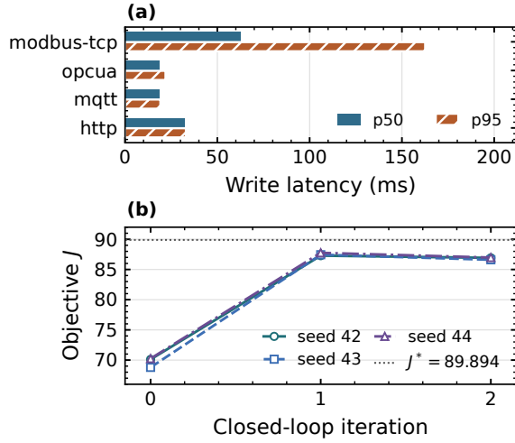
Fig. 5. Archive B. (a) Governed write latency p50 and p95 for the four writable stacks (numeric values in Table II); Modbus TCP carries the longest tail. (b) Fixed-controller objective J for seeds 42–44, sampled at the start and after each of two governed writes, against the archived finite-grid reference J^* = 89.894 . J is maximized. Each marker is one measured evaluation, so the third is the last one taken; it lies below the second because the second write raises defect rate. The archived J_{\text{end}} is a separate statistic, the mean of the last two evaluations, and is not plotted.
