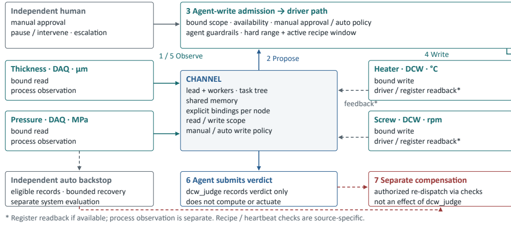
Fig. 3. The closed loop formed by the Section IV mechanisms. Numbered items are loop steps (steps 1 and 5 share the observation arrows), not the seven mechanism subsections of this section. The channel coordinates agents that observe bound nodes, propose setpoints, and pass admission checks before write and readback. Step 6 is the agent’s own verdict, the backstop a separate judgment path, and step 7 compensation that neither path performs. dcw_judge records a verdict only: it neither computes the conclusion from telemetry nor executes any action.
