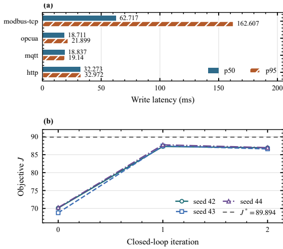
Fig. 5. Archive B . (a) Governed write latency p50 and p95 for the four writable stacks; Modbus TCP carries the longest tail. (b) Fixed-controller objective J for seeds 42–44, sampled at the start and after each of two governed writes, against the archived finite-grid reference J^* = 89.894 . J is maximized. Each marker is one measured evaluation, so the third is the last one taken; it lies below the second because the second write raises defect rate. The archived J_{\text{end}} is a separate statistic, the mean of the last two evaluations, and is not plotted.
