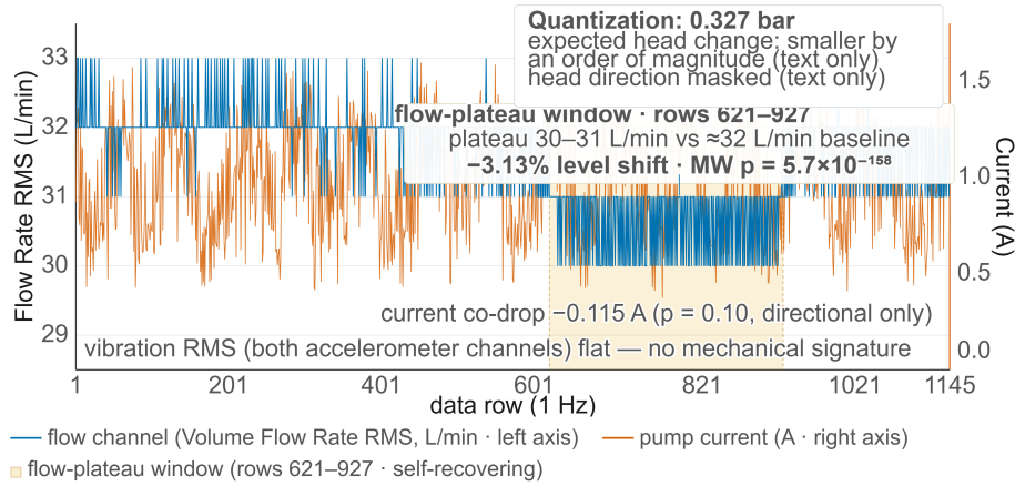
(b) Evidence chain from raw recording to capped verdict (levels L1 → L3 → L5 → survivors → verdict)
