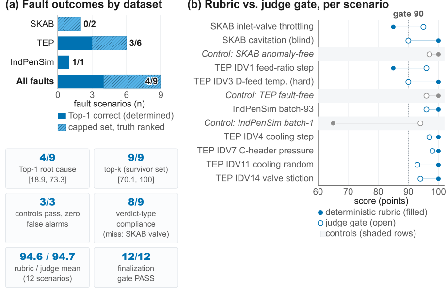
Figure 4: Benchmark outcomes under full-pipeline execution. (a) Fault outcomes by dataset: Top-1-correct DETERMINED verdicts (dark blue) and capped COMPETING_SET verdicts whose survivors rank the true mechanism (hatched sky blue)—no scenario’s survivors exclude the true mechanism. Bar length is proportional to the dataset’s fault count (the all-faults row, nine faults, is full scale); the printed fractions are keyword-instrument readings (Table 6 carries the identity-strict and recall-possible readings), and all three controls pass with zero false alarms (one of three blind; excluded from the bars). (b) Per-scenario deterministic rubric (filled markers) against the in-pipeline judge gate (open markers); dark blue = fault scenarios, shaded grey rows = controls; the dotted line is the judge’s 90-point gate. All 12 executions pass the finalization gate, and the artifact-consistency gate confirms that the evaluation is internally consistent.
