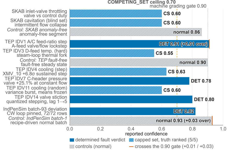
Figure 5: Reported confidence per scenario in the full-pipeline benchmark run. Solid dark blue bars are DETERMINED fault verdicts; hatched sky blue bars are the five capped COMPETING_SET verdicts (all with the true mechanism ranked among survivors); hatched grey bars are the three normal-operation controls; the dashed line is the 0.70 COMPETING_SET ceiling and the dotted line the machine grading gate’s flat 0.90 non-CS ceiling. The two bars crossing the dotted line (TEP IDV1 at 0.91, +0.01; IndPenSim control at 0.93, +0.03) mark the corpus’s one visible gap between the agent-side cap set (which documents no DET cap) and the machine gate (Section 4); the grading rubric records both as R4 calibration deductions. Each capped verdict names the discriminating measurement that would separate its surviving mechanisms; no conclusion is simultaneously DETERMINED and wrong (overconfidence 0).
