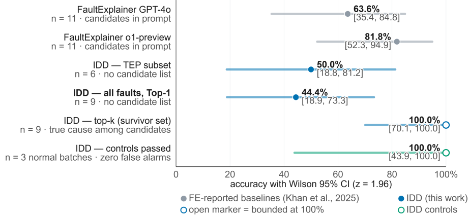
Figure 8: Register-A aggregate comparison with Wilson 95% intervals ( z=1.96 ). Grey: FaultExplainer-reported single-LLM baselines ( n=11 , candidates in prompt). Blue: IDD full-pipeline execution without candidate lists—the TEP subset (3/6), all nine faults Top-1 (4/9), and top- k (9/9, every fault’s survivors rank the true mechanism). Green: the three controls (3/3, no false alarms). Open markers mark the two readings bounded at 100% (top- k , controls), whose upper interval limits sit at the axis edge. Sets differ, so overlapping intervals are expected and no significance test is claimed; scenarios are purposive and non-exchangeable, so intervals are corpus-level measurement uncertainty (Section 9); the per-fault breakdown (Fig. 7; Table A1) is the finer-grained evidence.
