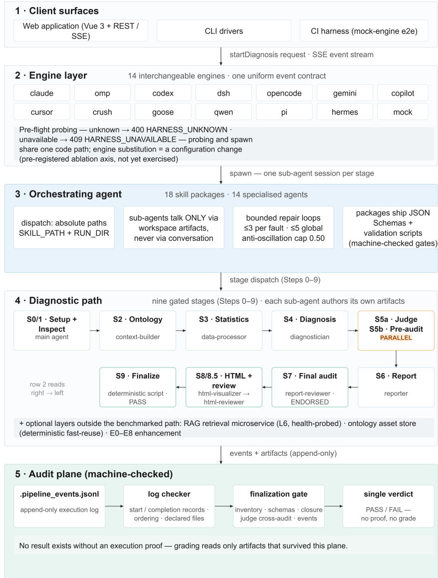
Figure 1: Skill execution architecture (diagram authored in draw.io; the .drawio source and the export script are released with the paper). Fourteen interchangeable engines expose one uniform event contract to the orchestrating agent, which dispatches the diagnostic path’s eight specialist sub-agents from 18 skill packages; sub-agents communicate only through workspace artifacts, and the audit plane’s log checker and finalization gate produce the execution proof the benchmark grader consumes.
