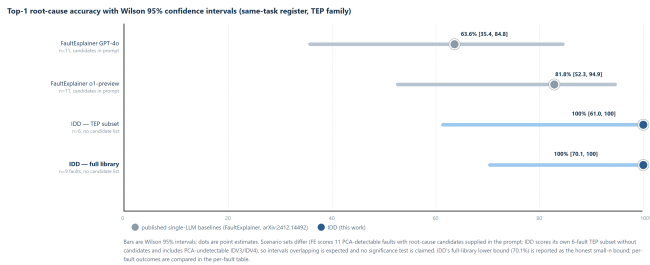
Fig. 5. Register-A aggregate comparison with Wilson 95% intervals. Grey: FaultExplainer-reported single-LLM baselines ( n=11 , candidates in prompt). Blue: IDD (no candidates). Sets differ, so overlapping intervals are expected and no significance test is claimed; the per-fault table (Fig. 4) is the finer-grained evidence.
