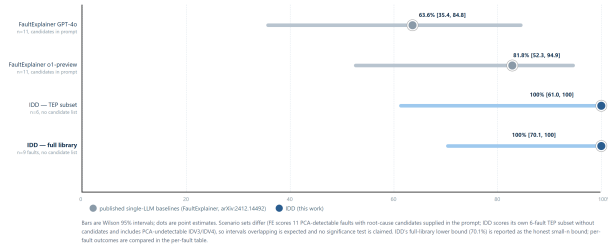
Top-1 root-cause accuracy with Wilson 95% confidence intervals (same-task register, TEP family)
