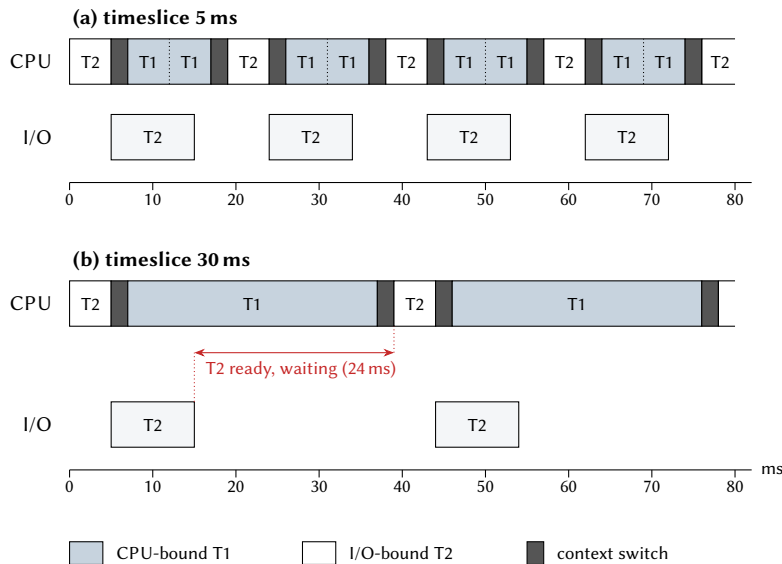
Figure 7.4: A CPU-bound task T1 and an I/O-bound task T2 under round robin (Example 7.16). When a timeslice of T1 expires while T2 is still waiting for its I/O, T1 simply continues.
