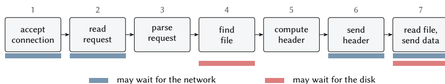
Figure 6.2: Processing steps of a simple web server for static content. Bars below a step show which resource it may have to wait for.
