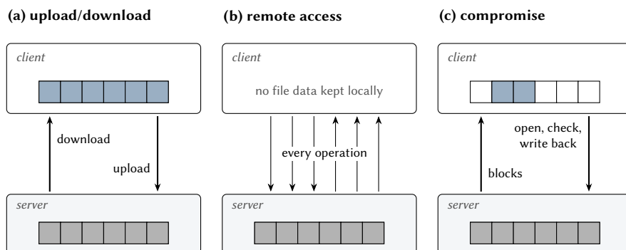
Figure 14.2: Remote file service. (a) The client downloads the whole file and uploads it when done. (b) The file stays at the server, which performs every operation. (c) The client caches some blocks but interacts with the server frequently.
