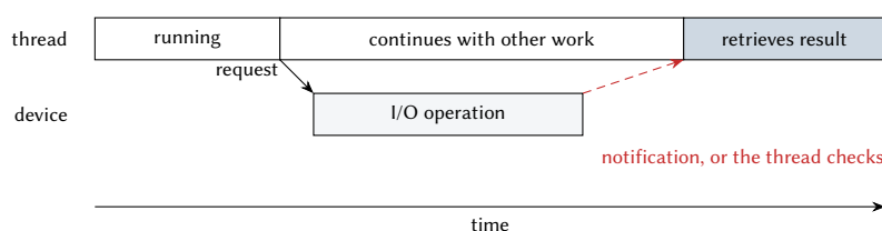
Figure 11.5: (a) With synchronous I/O the thread blocks until the device completes the operation. (b) With asynchronous I/O the thread continues and retrieves the result after being notified or after checking.
