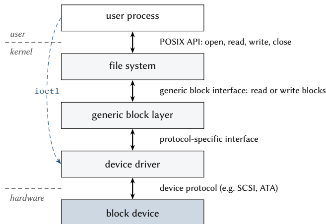
Figure 11.6: The block device stack. Each layer uses the interface shown below it; ioctl carries device-specific requests to the driver.
