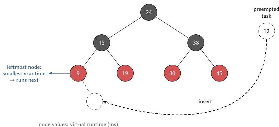
Figure 7.7: The runqueue of CFS, a red-black tree of the ready tasks ordered by virtual runtime (grey nodes are black, red nodes are red). The leftmost task runs next; a preempted task is inserted at the position given by its virtual runtime.
