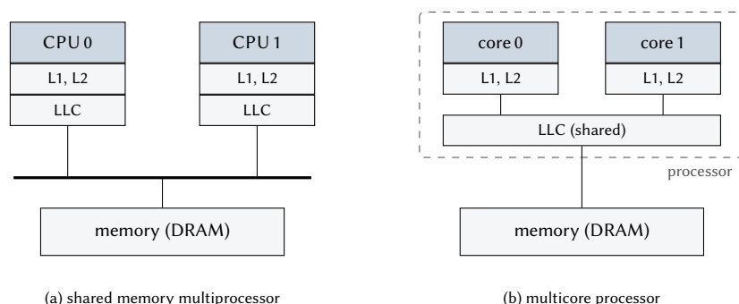
Figure 7.8: (a) A shared memory multiprocessor: every CPU has its own caches. (b) A multicore processor: the cores have private caches and share the last-level cache.
