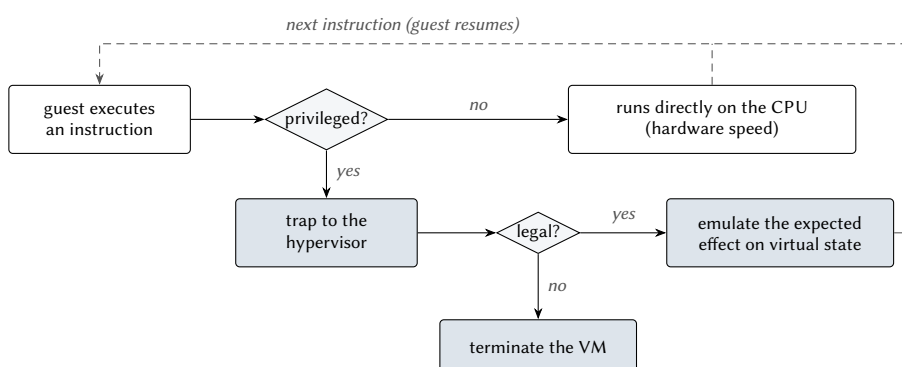
Figure 12.4: Trap-and-emulate. Only privileged instructions involve the hypervisor; legal ones are emulated on the virtual state of the VM.
