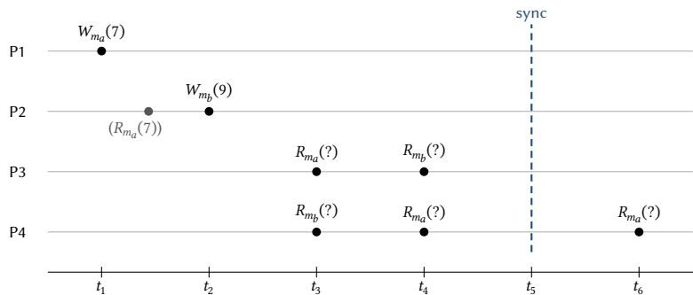
Figure 15.7: Operations of Example 15.15. P2's read of m_a (grey) occurs only in the variant in which P2's write depends on P1's. The dashed line is a synchronization point.
