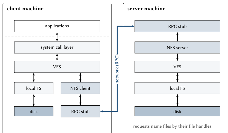
Figure 14.6: NFS. The client's VFS passes operations on NFS files to the NFS client, which sends them as RPC requests to the NFS server; the server performs them through its VFS and local file system.
