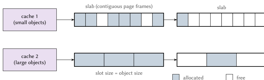
Figure 8.10: A slab allocator with a cache for small and a cache for large objects. Every slab is divided into slots of the object size.
