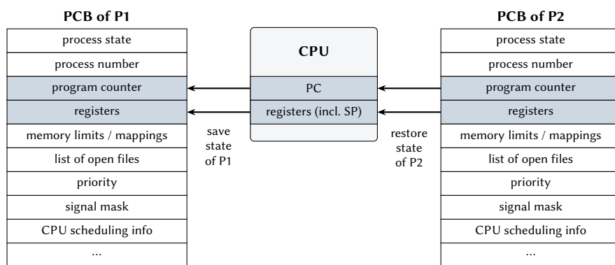
Figure 2.3: Process control blocks of P1 and P2. The shaded fields hold values that the CPU maintains in its registers while the process runs; they are saved into the PCB when the process stops running and restored from it when the process runs again.
