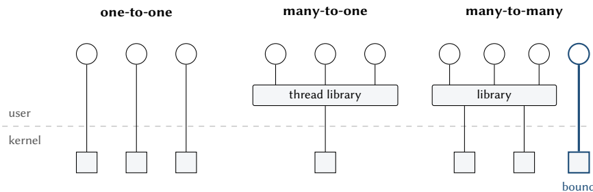
Figure 3.6: Multithreading models. Circles are user-level threads, squares kernel-level threads. In the many-to-many model a bound thread keeps a kernel-level thread of its own.
