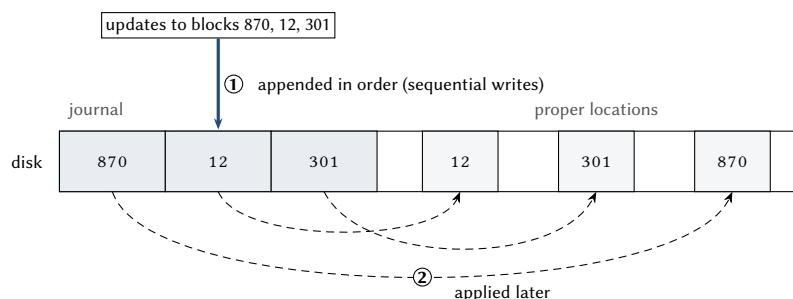
Figure 11.11: Journaling. Updates to scattered blocks are first appended in order to the journal and later applied to their proper locations.
