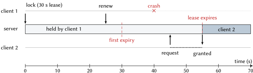
Figure 14.7: Lease-based locking. Client 1 renews its lease at 25 s and crashes at 40 s; when the lease expires at 55 s, the server grants the lock to client 2.
