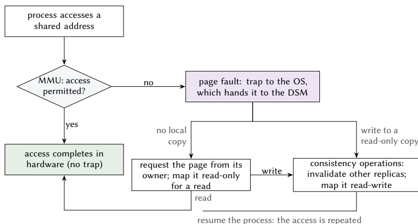
Figure 15.6: Intercepting accesses in a page-based DSM. Accesses permitted by the current mapping never leave the hardware; the others fault, and the DSM fetches the page or performs consistency operations before the access is repeated.
