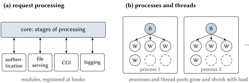
Figure 6.6: The Apache web server. (a) Modules register handlers at the stages of request processing that the core provides. (b) Several processes, each a boss (B) with a pool of workers (W); dashed circles are workers created as load increases.
