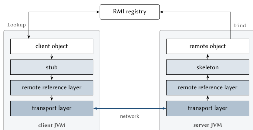
Figure 13.6: Java RMI. Invocations pass from the client through the stub, the remote reference layer and the transport layer to the server, where the skeleton delivers them to the remote object.
