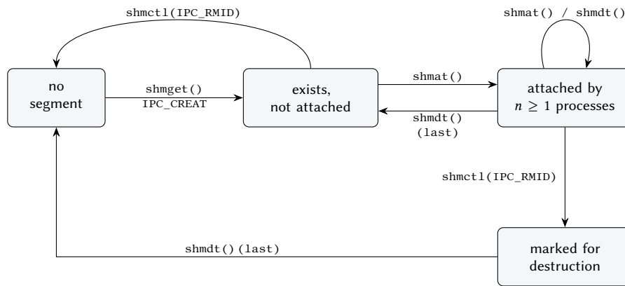
Figure 9.3: Life cycle of a System V shared memory segment. A segment outlives the processes that use it and is removed only by IPC_RMID ; a segment removed while still attached is destroyed when the last process detaches.
