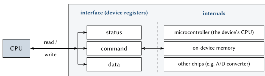
Figure 11.1: A basic I/O device. The CPU interacts with the device only through its command, status and data registers; the internals that carry out the commands are device-specific.
