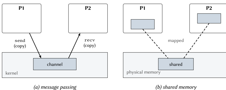
Figure 2.9: (a) Message passing copies every message into a channel in the kernel and out again. (b) With shared memory, the same physical pages are mapped into both address spaces.
