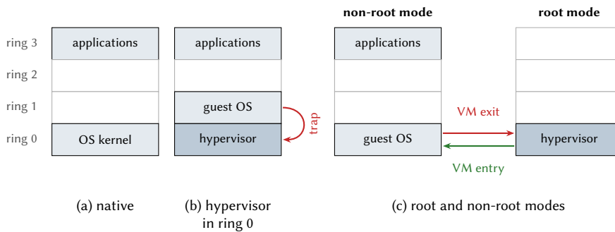
Figure 12.3: Use of the x86 protection rings. (a) Native execution. (b) Virtualization without hardware support: the guest OS is deprived to ring 1, and its privileged operations trap to the hypervisor. (c) Processors with virtualization support: the guest OS runs in ring 0 of non-root mode, and a VM exit transfers control to the hypervisor in root mode.
