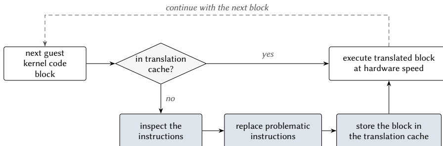
Figure 12.5: Dynamic binary translation with a translation cache. A block is inspected and translated only the first time it is about to run.
