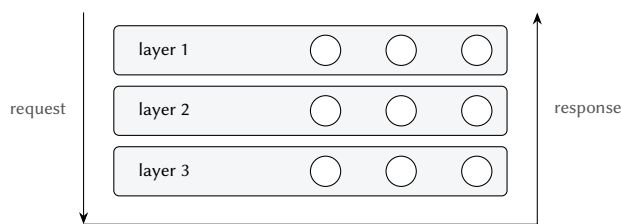
Figure 3.9: The layered pattern: each layer groups related subtasks and has its own threads; a request passes down through the layers and back up.
