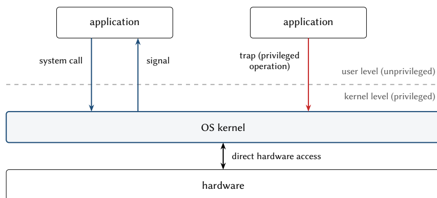
Figure 1.2: The user/kernel protection boundary. Only the kernel accesses the hardware; applications enter the kernel through system calls or traps, and the kernel notifies applications with signals.
