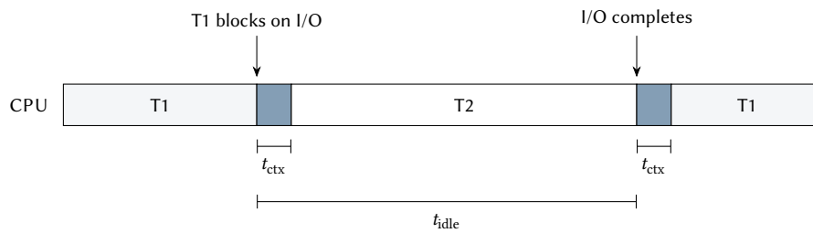
Figure 3.2: T1 blocks on I/O; instead of idling, the CPU switches to T2, and the completion of the I/O triggers the switch back. The switches pay off when they cost less than the idle time (Equation (3.1)).
