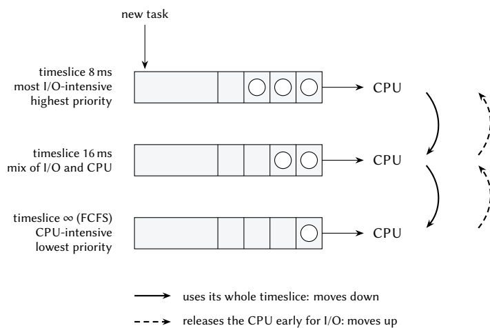
Figure 7.5: A multi-level feedback queue with three levels. Each level serves its tasks with its own timeslice; tasks move between levels according to how they use their timeslices.
