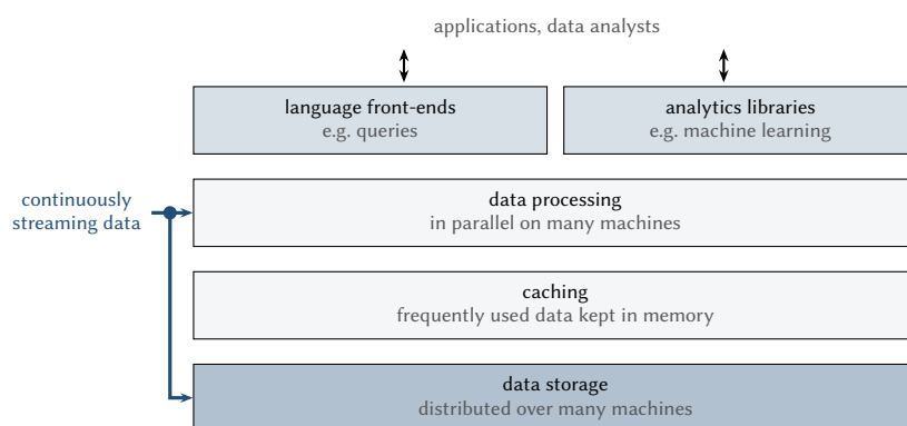
Figure 16.5: The layers of a big data engine. Streaming data enter the engine continuously; they are processed as they arrive and stored.
