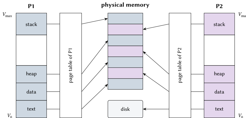
Figure 2.2: Two processes with the same range of virtual addresses. Their page tables map the allocated regions to different physical frames; the text of P2 is currently on disk, and the unallocated regions are not mapped at all.
