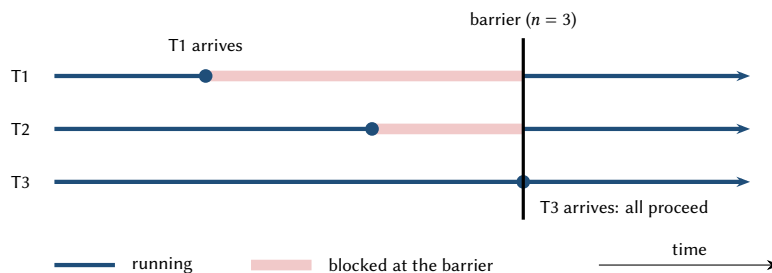
Figure 10.3: A barrier for three threads. T1 and T2 block when they reach the barrier; the arrival of T3 releases all three.
