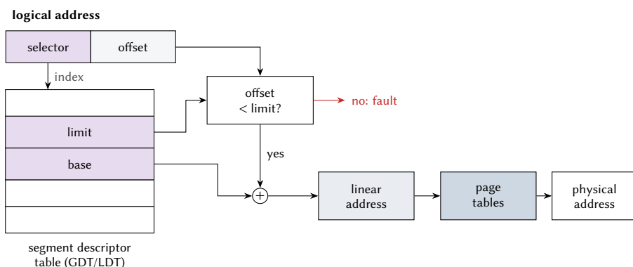
Figure 8.7: Segmentation combined with paging on x86. The selector indexes the segment descriptor table; an offset within the limit is added to the base, and the resulting linear address is translated by the page tables.
