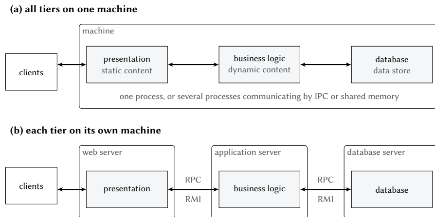
Figure 16.1: A three-tier Internet service. (a) All tiers run on one machine, in one process or in several processes. (b) Every tier runs on its own machine, and the tiers communicate by RPC or RMI.
