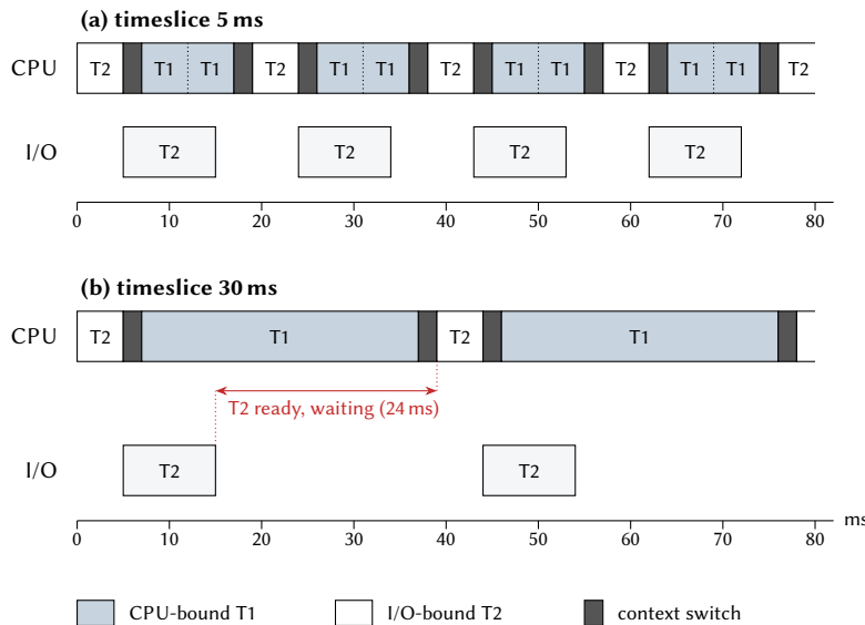
Figure 7.4: A CPU-bound task T1 and an I/O-bound task T2 under round robin (Example 7.16). When a timeslice of T1 expires while T2 is still waiting for its I/O, T1 simply continues.
