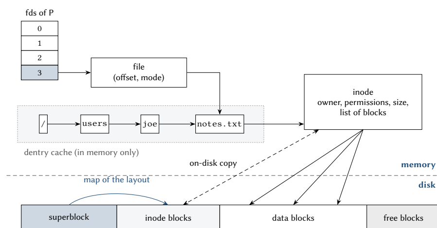
Figure 11.8: VFS abstractions. File descriptor 3 of process P refers to an open file, whose dentry leads to the inode; the dentries of the path exist only in memory. On disk, the superblock maps the blocks that hold inodes, data and free space.
