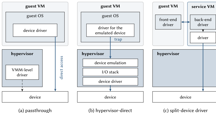
Figure 12.7: Device virtualization models. (a) The VM's own driver accesses the device directly. (b) The hypervisor intercepts device accesses and emulates them with its own I/O stack and driver. (c) A front-end driver in the guest passes requests to a back-end driver in the service VM, which drives the device.
