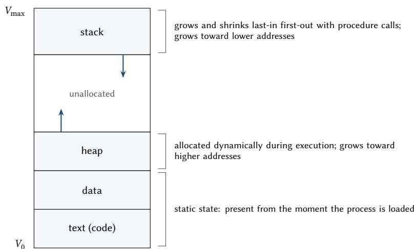
Figure 2.1: Address space of a process. The heap and the stack grow toward each other; the addresses between them are not allocated.
