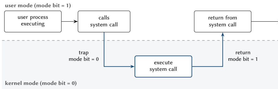
Figure 1.3: Execution of a system call: a trap switches to kernel mode, the kernel executes the call, and the return switches back to user mode. The mode bit follows the convention of Silberschatz et al. [2]: 0 in kernel mode, 1 in user mode.
