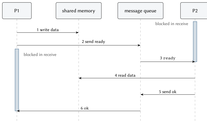
Figure 9.4: A message queue coordinates access to shared memory: P2 reads only after “ready”, and P1 continues only after “ok”.
