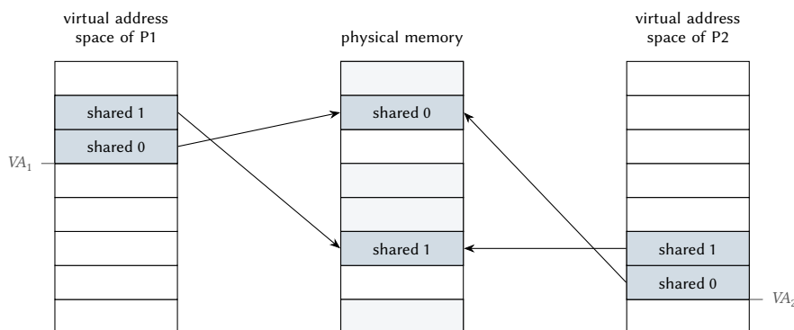
Figure 9.2: Shared memory. Two page frames are mapped into both address spaces; P1 sees the region at virtual address VA_1 , P2 at a different address VA_2 , and the frames are not adjacent in physical memory.
