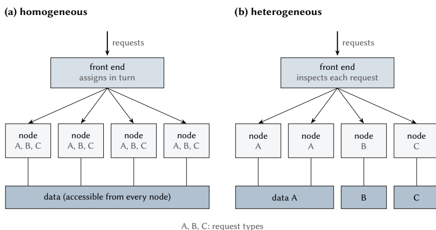
Figure 16.2: Scale-out architectures. (a) Every node processes requests of every type, and every node can access all data. (b) Nodes are specialized for request types, and the front end must inspect each request to choose a node.
