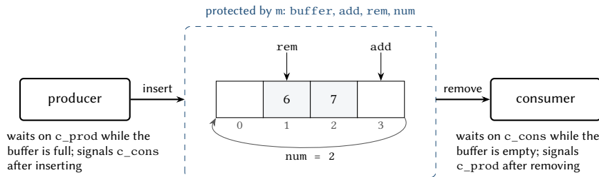
Figure 4.3: The producer-consumer program with BUF_SIZE = 4 : one mutex protects all buffer state, and each thread waits on its own condition variable.
