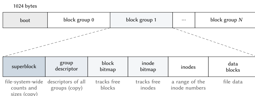
Figure 11.9: Layout of an ext2 partition. After the space reserved for booting, the partition is divided into block groups, each with a copy of the superblock and of the group descriptor table, its own bitmaps, and its inodes and data blocks.
