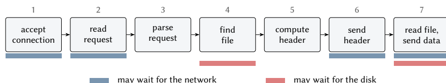
Figure 6.2: Processing steps of a simple web server for static content. Bars below a step show which resource it may have to wait for.
