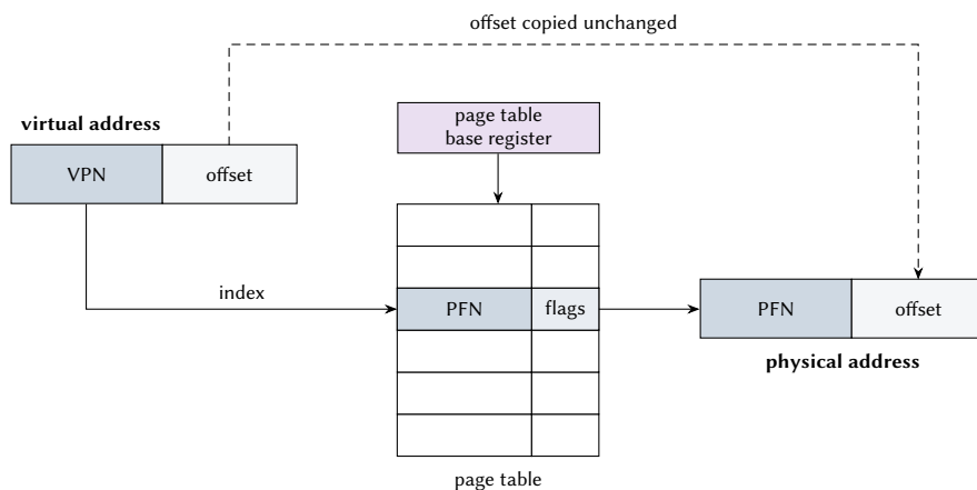
Figure 8.3: Address translation with a page table. The VPN selects the entry of the page table of the running process; its PFN, combined with the unchanged offset, forms the physical address.
