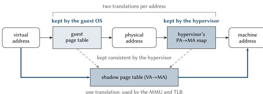
Figure 12.6: Memory virtualization. Translating through the guest page table and then through the hypervisor's mapping takes two steps; the shadow page table combines them into one mapping that the MMU uses directly. Hardware with extended page tables performs the two-step translation itself (Section 12.11).
