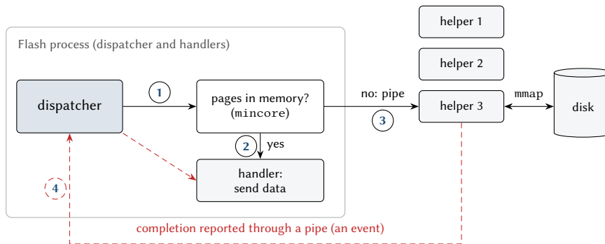
Figure 6.5: Serving file data in Flash. (1) The dispatcher tests with mincore whether the data are in memory. (2) If they are, a handler sends them directly. (3) Otherwise a helper is asked through a pipe to access the pages, reading them from disk. (4) Its completion report is an event, after which the handler sends the data.
