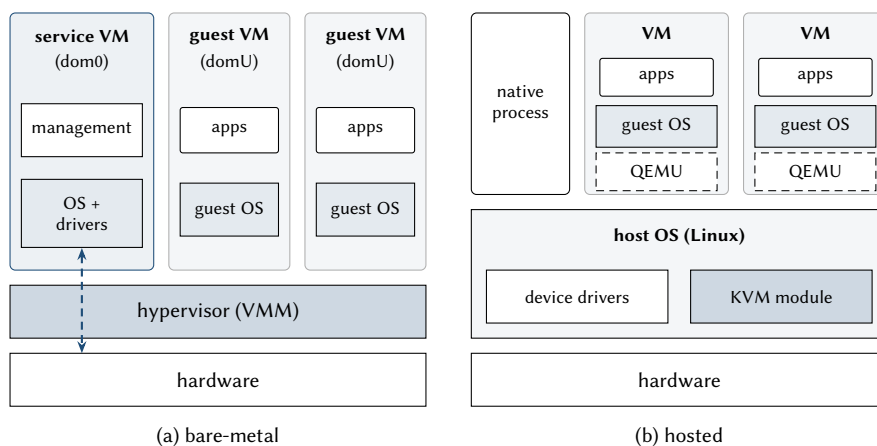
Figure 12.2: Virtualization models. (a) A bare-metal hypervisor with a privileged service VM that owns the device drivers, as in Xen. (b) A hosted hypervisor: a module of the host OS, as KVM in Linux; each VM is a host process in which QEMU emulates the devices.
