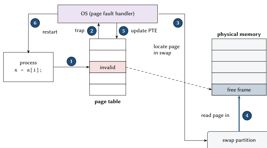
Figure 8.11: Demand paging: the steps taken when a process references a page that is in the swap partition.
