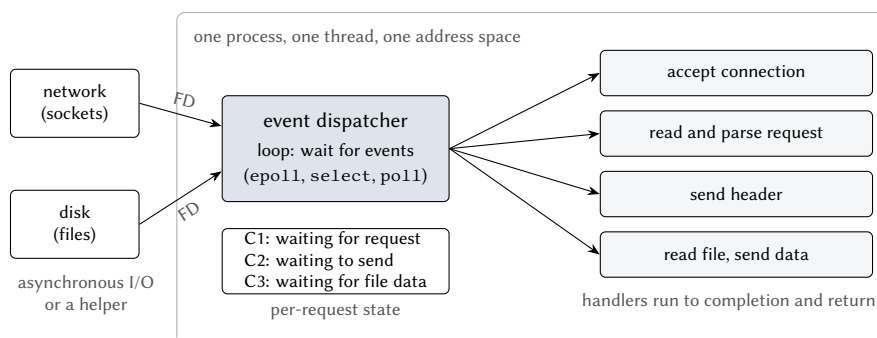
Figure 6.4: An event-driven web server. The dispatcher waits for events on file descriptors (FDs)—sockets that are ready, and disk reads whose completion is reported by asynchronous I/O or by a helper (Section 6.6)—and invokes the handler for each event. The state of every request in progress is kept in an explicit record.
