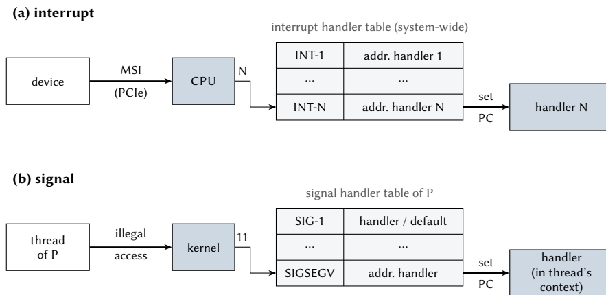
Figure 5.5: (a) An interrupt raised by a device selects a handler from the system-wide interrupt handler table. (b) An illegal memory access makes the kernel raise SIGSEGV, which selects a handler from the signal handler table of the process.
