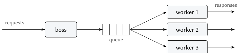
Figure 3.7: Boss-workers with a work queue: the boss only enqueues requests; every worker takes a request from the queue and performs the entire task.
