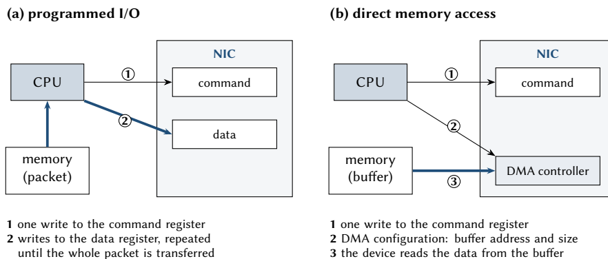
Figure 11.3: Sending a packet. (a) With programmed I/O the CPU copies the packet into the data register piece by piece. (b) With DMA the CPU only writes the command and configures DMA; the device reads the packet from memory.
