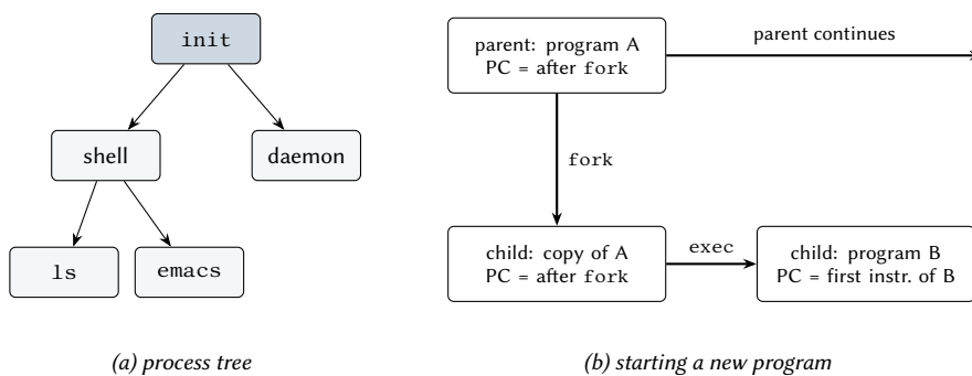
Figure 2.6: (a) Processes form a tree rooted in the initial process. (b) A child created by fork is a copy of its parent; exec replaces its program with a new one.
