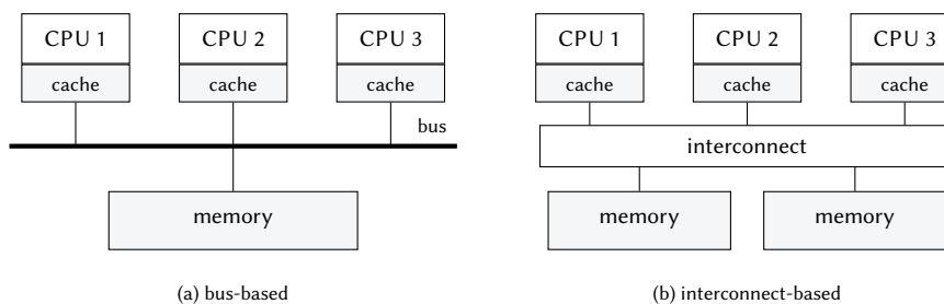
Figure 10.4: Shared memory multiprocessor configurations. In both, every CPU has its own cache and all CPUs can access all memory.
