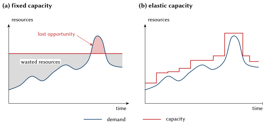
Figure 16.3: Capacity and demand over time. (a) A fixed capacity wastes resources while demand is low and loses requests during a surge. (b) An elastic capacity follows the demand.
