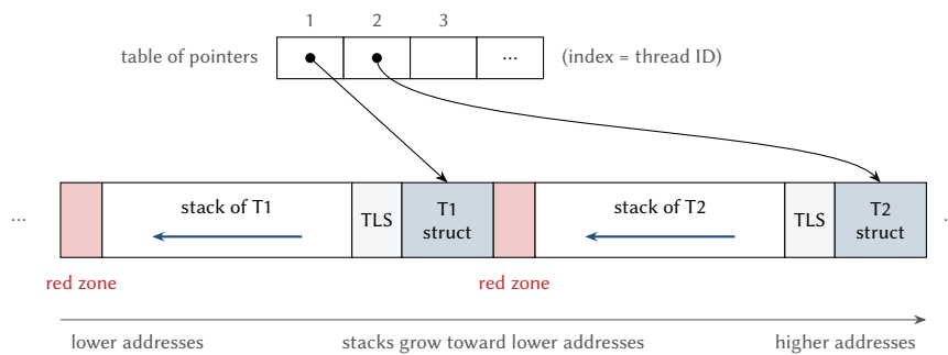
Figure 5.3: User-level thread data structures allocated contiguously. The thread identifier indexes a table of pointers to the structures. An overflow of the stack of T2 runs into the red zone before it can reach the structure of T1.
