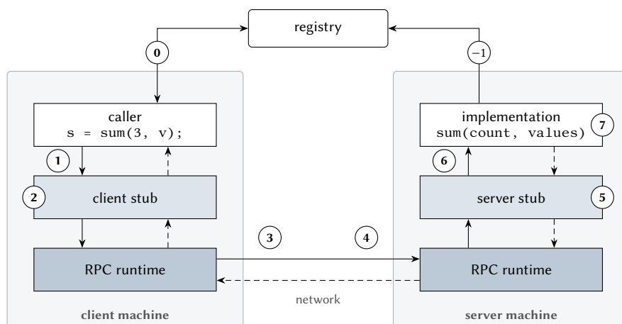
Figure 13.1: Structure of an RPC system and the steps of a call. Solid arrows: the call; dashed arrows: the return of the result. Steps –1 and 0 take place before the first call.
