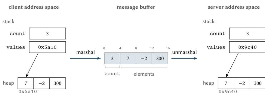
Figure 13.2: Marshalling and unmarshalling the arguments of sum(3, v) . The buffer contains the values of the arguments, including the array to which the pointer refers, but not the pointer itself; the numbers above it are byte offsets.
