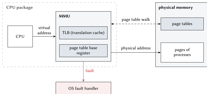
Figure 8.2: Hardware support for memory management. The MMU translates virtual addresses with the help of its TLB, walks the page tables in physical memory when a translation is not cached, and raises a fault to the operating system when an access is not possible.
