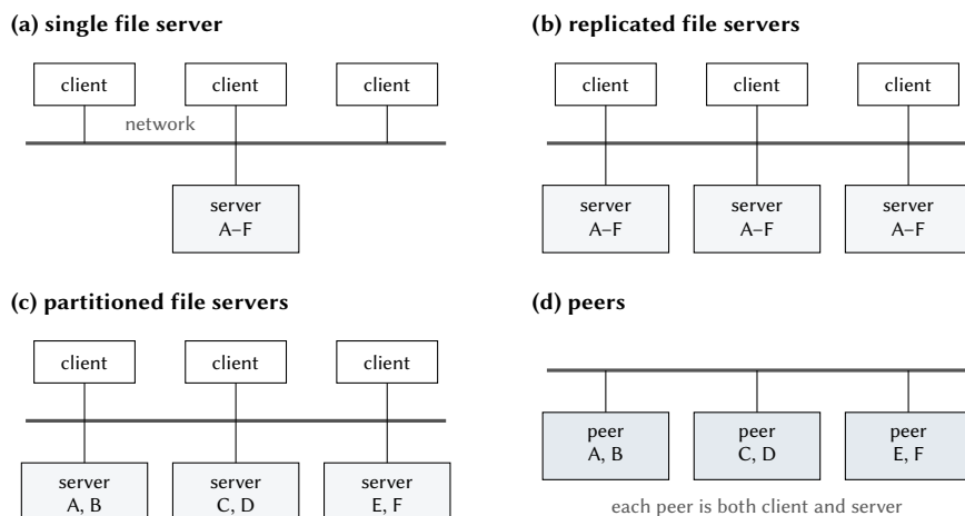
Figure 14.1: DFS models. (a) A single server stores all files. (b) Every server of a replicated file server holds all files. (c) Each server of a partitioned file server holds some of the files. (d) All machines are peers that store files and serve them.
