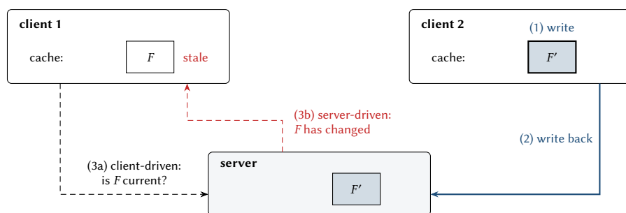
Figure 14.3: Client 2 modifies its cached copy of F and writes it back. Client 1 learns that its copy is stale either by asking the server (client-driven) or by being notified (server-driven).
