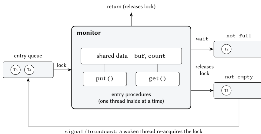
Figure 10.2: A monitor. Threads enter only through entry procedures, which acquire the monitor's lock implicitly; a thread that waits on a condition variable releases the lock and, with the Mesa semantics shown here, must re-acquire it after being woken.
