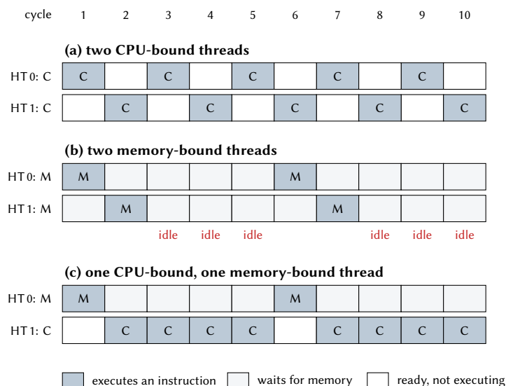
Figure 7.10: Co-scheduling two threads on the hardware threads (HT) of one SMT CPU, with C for a CPU-bound and M for a memory-bound thread. Each column is a cycle of the shared pipeline.
