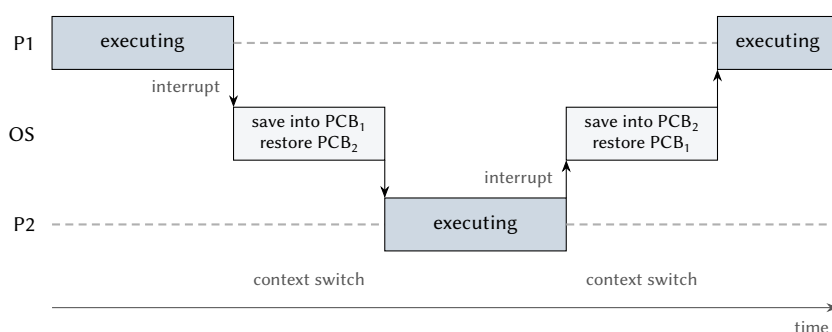
Figure 2.4: Two context switches between P1 and P2. Each process is idle (dashed) while the other runs, and its state waits in its PCB.
