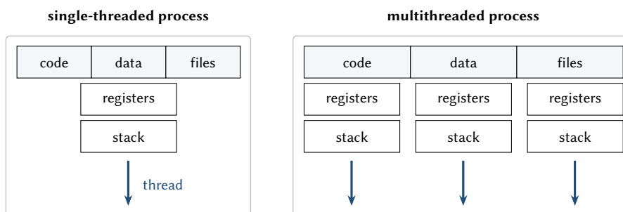
Figure 3.1: A single-threaded and a multithreaded process. The shaded state (code, data and open files) is shared by all threads; every thread has its own registers—including PC and SP—and its own stack.
