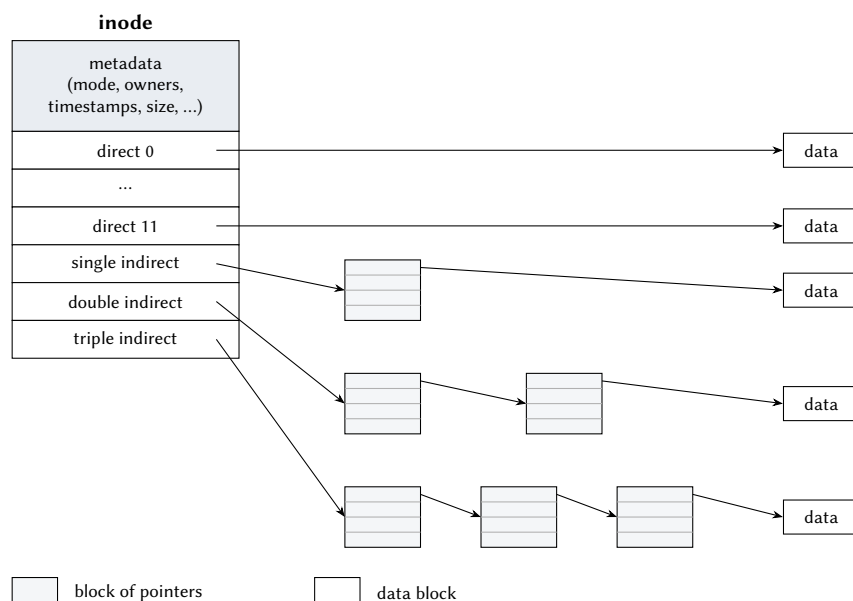
Figure 11.10: An inode with 12 direct pointers and single, double and triple indirect pointers. Each level of indirection multiplies the number of reachable data blocks by the number of pointers per block.
