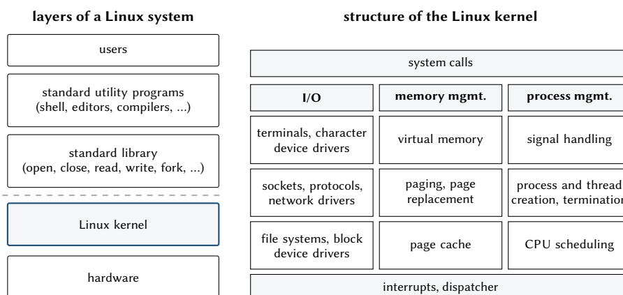
Figure 1.5: Left: the layers of a Linux system; the dashed line is the user/kernel boundary. Right: the components of the Linux kernel (after Tanenbaum and Bos [5]).
