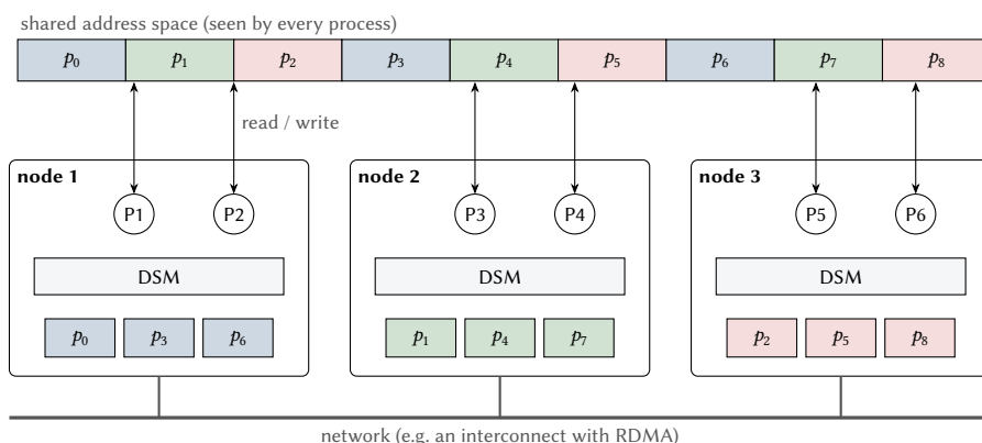
Figure 15.1: Distributed shared memory. Every page p_i of the shared address space resides in memory contributed by one of the nodes; the DSM layer of each node serves accesses to local pages and obtains remote pages over the network.
