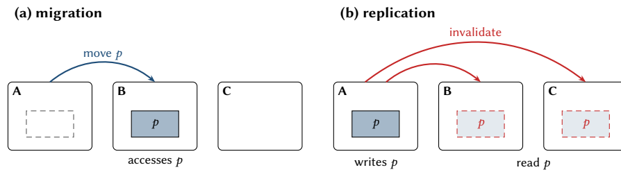
Figure 15.3: Bringing page p to the nodes that access it. (a) Migration moves the single copy. (b) Replication keeps copies on several nodes, which read p locally; a write by the owner A invalidates the replicas on B and C (dashed).
