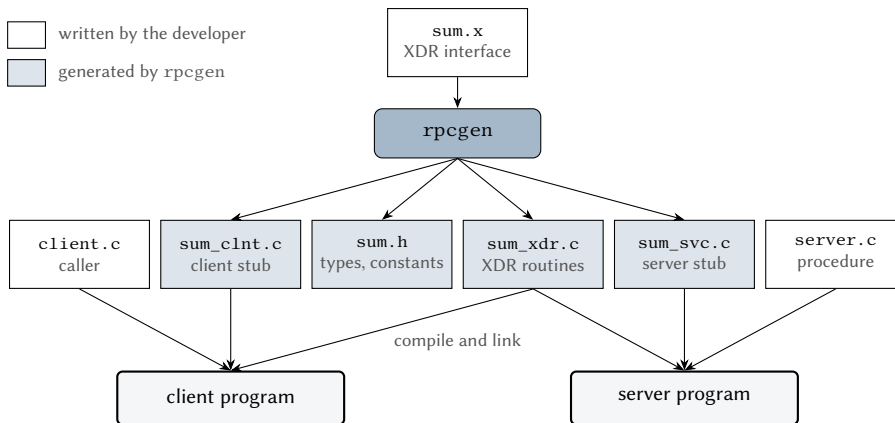
Figure 13.4: Building a Sun RPC client and server. The developer writes the interface, the client program and the implementation of the procedure; rpcgen generates the rest. sum.h is included by all C files.
