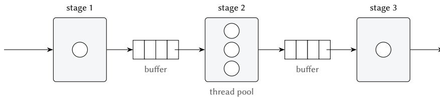
Figure 3.8: A three-stage pipeline. Stages exchange requests through buffers; the slow second stage is a pool of three threads.
