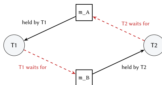
Figure 3.5: Wait graph of the deadlock: following the edges from T1 leads through m_B , T2 and m_A back to T1.
