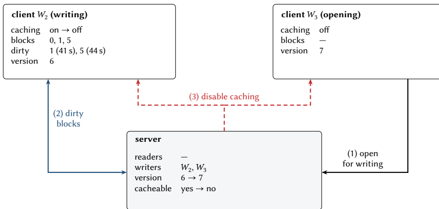
Figure 14.8: Per-file state in Sprite. When W_3 opens the file that W_2 has open for writing (1), the server collects W_2 's dirty blocks (2) and disables caching on both clients (3).
