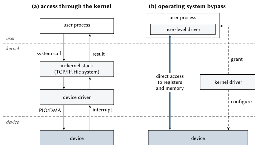
Figure 11.4: (a) A typical device access passes through the system call, the in-kernel stack and the device driver. (b) With operating system bypass the process accesses the device through a user-level driver; the kernel only configures and controls the access.
