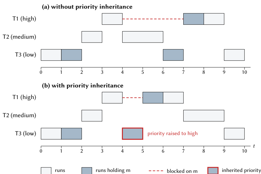
Figure 7.3: T1 and T3 share mutex m . (a) While T1 is blocked on m , the medium-priority T2 runs to completion ahead of it. (b) With priority inheritance, T3 runs at the priority of T1 until it unlocks m , and T1 completes before T2.
