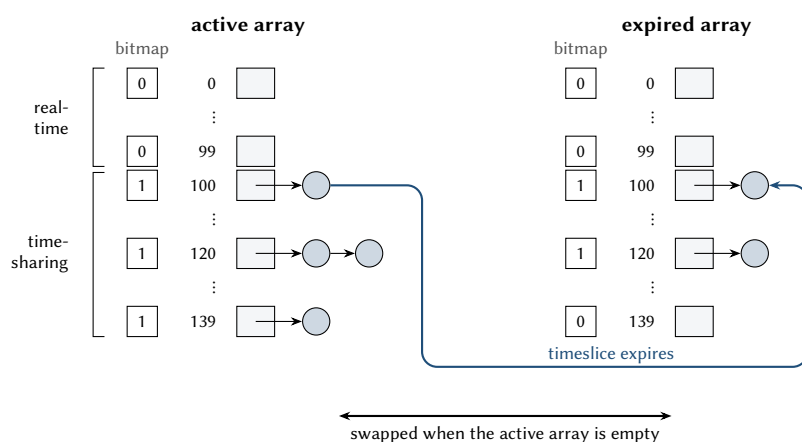
Figure 7.6: The runqueue of the O(1) scheduler. Each array has one list per priority level and a bitmap of the non-empty lists. A task whose timeslice expires moves to the expired array; when the active array is empty, the two arrays are swapped.
