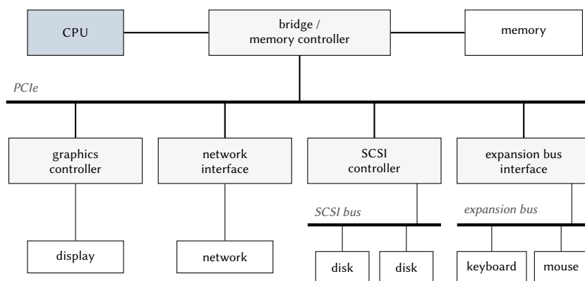
Figure 11.2: A typical platform interconnect. Device controllers are attached to PCIe; disks and keyboards are attached to further buses behind their own controllers. PCIe is drawn as a bus for simplicity; each controller is in fact attached through its own point-to-point link.
