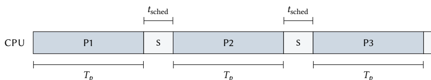
Figure 2.7: Processes run for T_p each; the scheduler (S) runs for t_{\text{sched}} between them.
