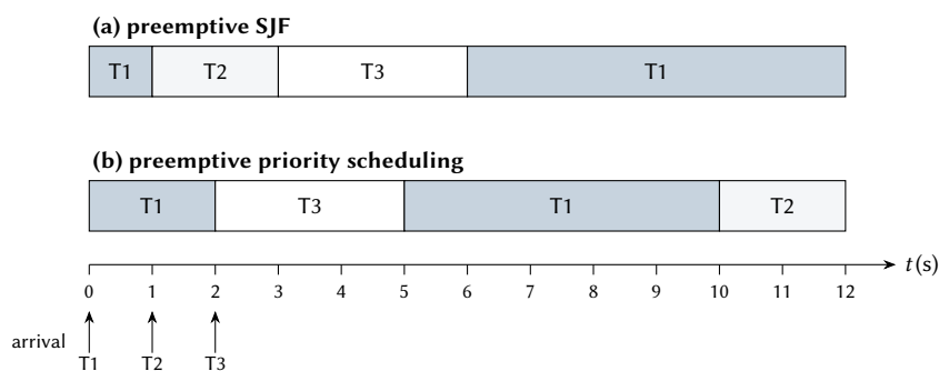
Figure 7.2: The tasks of Example 7.8 under (a) preemptive SJF and (b) preemptive priority scheduling.
