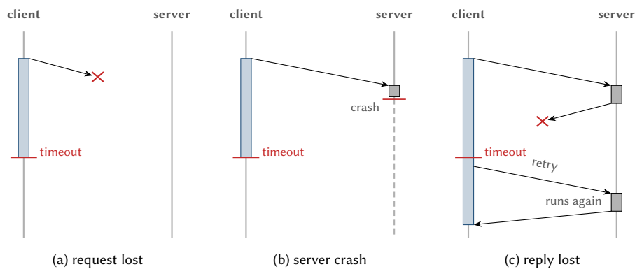
Figure 13.3: Three partial failures that the client cannot distinguish. The shaded bar marks the time during which the client is blocked, grey boxes the execution of the procedure, and a cross a lost message. (a) The request is lost; (b) the server crashes while executing the call; (c) the reply is lost, and the retry executes the procedure a second time.
