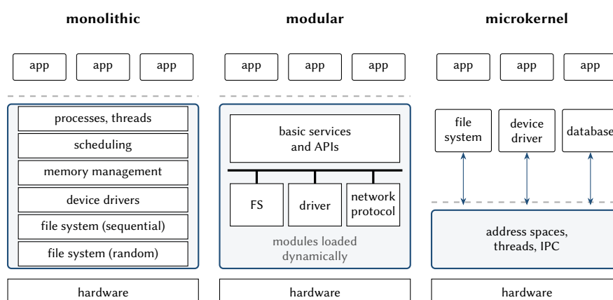
Figure 1.4: Three organizations of an operating system. The dashed line is the user/kernel boundary. A monolithic kernel contains every service; a modular kernel adds services as modules through a common interface; a microkernel keeps only address spaces, threads and IPC, and runs all other services at user level.
