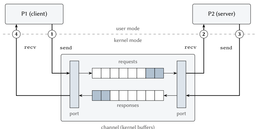
Figure 9.1: A request-response exchange over message-based IPC. Each numbered crossing of the user/kernel boundary is one system call and one copy between a process's address space and the kernel's channel.
