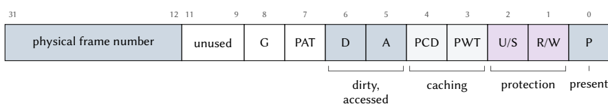
Figure 8.4: A 32-bit x86 page table entry. The global bit G and the page attribute bit PAT are not discussed here.
