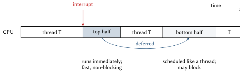
Figure 5.6: Interrupt handling divided into a top half, which interrupts thread T, and a bottom half, which the scheduler runs later.
