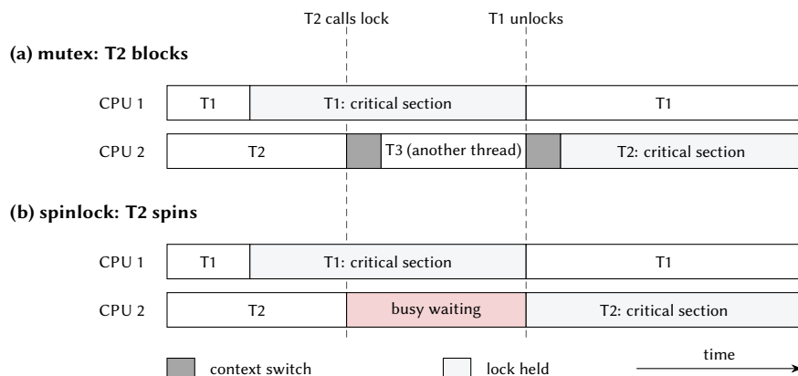
Figure 10.1: Thread T2 requests a lock held by T1 on another CPU. (a) On a mutex, T2 blocks, the CPU runs another thread, and T2 is switched back in after the unlock. (b) On a spinlock, T2 busy-waits and enters the critical section as soon as T1 unlocks.
