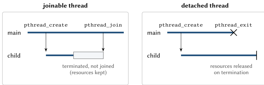
Figure 4.1: Left: a joinable child that terminates before it is joined keeps its resources until pthread_join collects its status. Right: a detached child releases its resources itself; the main thread ends with pthread_exit , which leaves the process running whether the remaining threads are joinable or detached.
