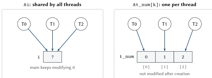
Figure 4.2: Left: all threads receive the address of the loop variable i , whose value changes while they start. Right: each thread receives the address of its own array element, which does not change after the thread has been created.
