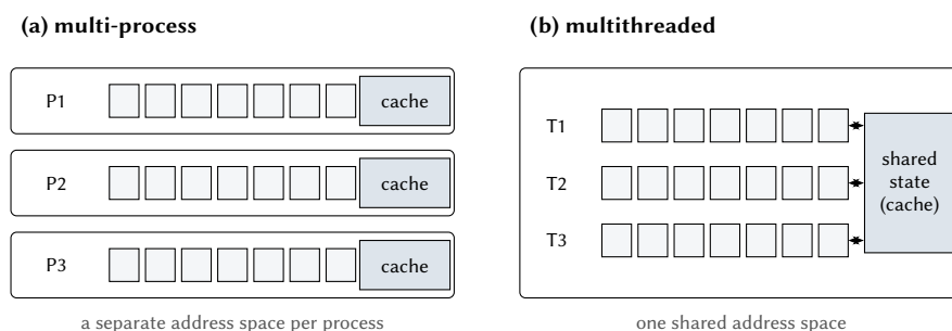
Figure 6.3: (a) The multi-process model: every process executes all processing steps (cells) of one request and keeps its own copy of state such as a cache. (b) The multithreaded model: threads in one address space execute the steps and share the state.
