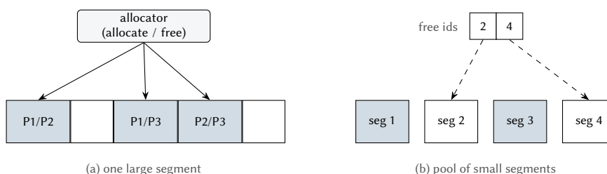
Figure 9.5: Organizing shared memory for several pairs of processes: (a) one large segment whose portions an allocator hands out; (b) a pool of small segments whose free identifiers are kept in a queue.
