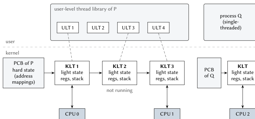
Figure 5.1: Thread data structures at scale. The PCB of a process keeps the state shared by all its threads and a list of its kernel-level threads (KLTs); each KLT keeps its own state and, while it runs, is linked to a CPU. Dashed lines show which user-level threads (ULTs) the library has currently placed on which KLTs. Back pointers from KLTs to PCBs are omitted.
