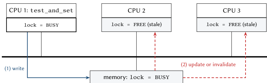
Figure 10.5: CPU 1 sets lock to BUSY . The copies in the caches of CPU 2 and CPU 3 become stale; on a cache-coherent platform the hardware updates or invalidates them.
