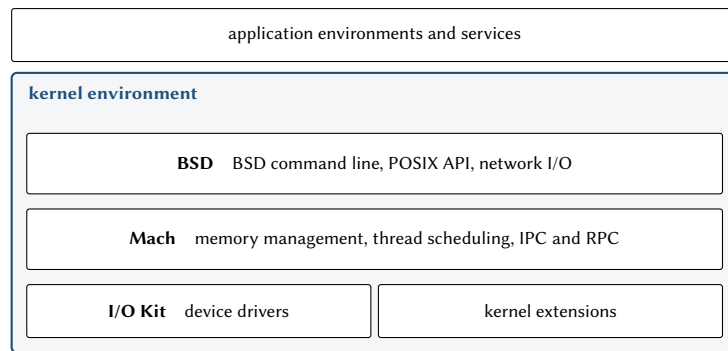
Figure 1.6: The structure of Mac OS X: the Mach microkernel with a BSD layer, the I/O Kit and kernel extensions, all of which run in kernel mode.
