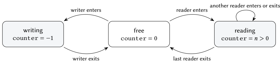
Figure 3.4: The states of the shared resource and the corresponding values of the proxy variable; counter is short for resource_counter .
