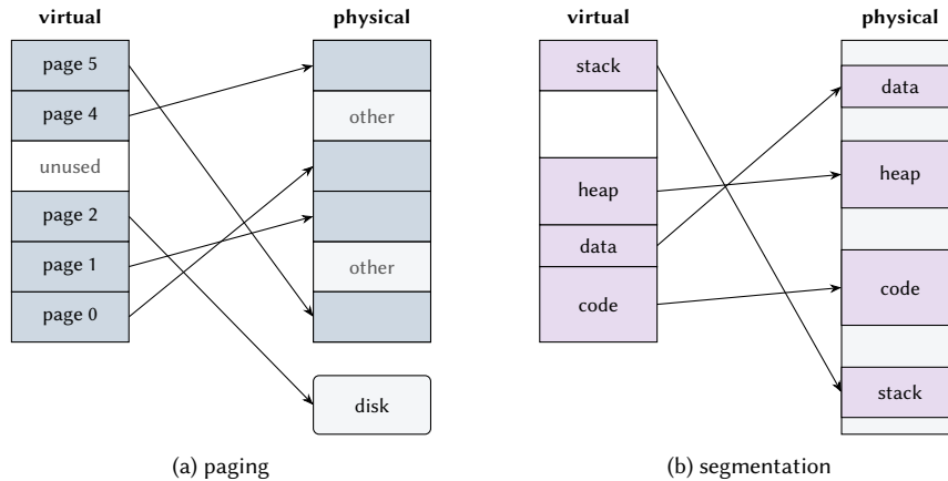
Figure 8.1: (a) Paging maps fixed-size pages to page frames; page 2 is on disk, and the unused page has no mapping. (b) Segmentation maps segments of different sizes to regions of physical memory of the same sizes.
