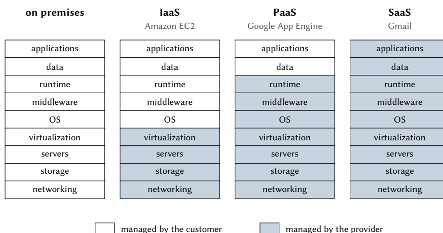
Figure 16.4: Cloud service models, with an example of each. The shaded layers are managed by the provider, the others by the customer.
