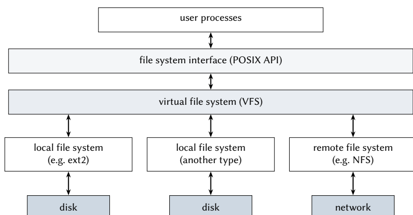
Figure 11.7: The virtual file system maps the operations of the file system interface to the concrete local and remote file systems.
