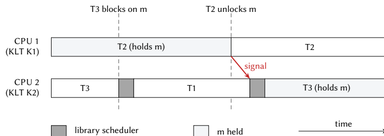
Figure 5.4: User-level threads with priorities T3 > T2 > T1 on two CPUs. When T2 unlocks m , the library on CPU 1 signals K2 so that the library on CPU 2 preempts T1 in favour of T3.
