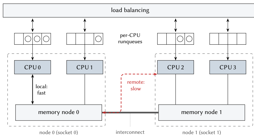
Figure 7.9: Hierarchical scheduling on a NUMA system. Every CPU schedules tasks from its own runqueue, and load balancing moves tasks between the runqueues. A CPU reaches the memory of its own node directly and the memory of the other node through the interconnect.
