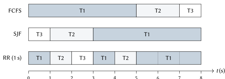
Figure 7.1: Three tasks that arrive at time 0 in the order T1, T2, T3, with execution times of 5 s, 2 s and 1 s, under FCFS, SJF and round robin with a timeslice of 1 s (Section 7.5). Dotted lines separate consecutive timeslices of the same task.
