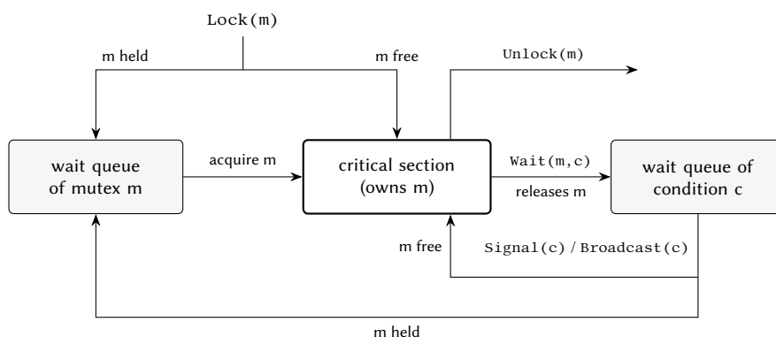
Figure 3.3: A thread waiting on condition c releases mutex m . When it is signalled it must first re-acquire m ; if m is held, it moves to the wait queue of the mutex.
