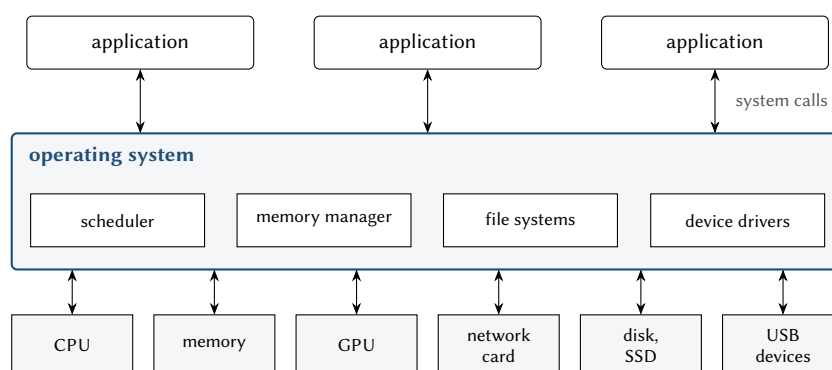
Figure 1.1: The operating system between applications and hardware. Applications request services through system calls; components such as the scheduler, the memory manager, file systems and device drivers carry them out on the hardware.
