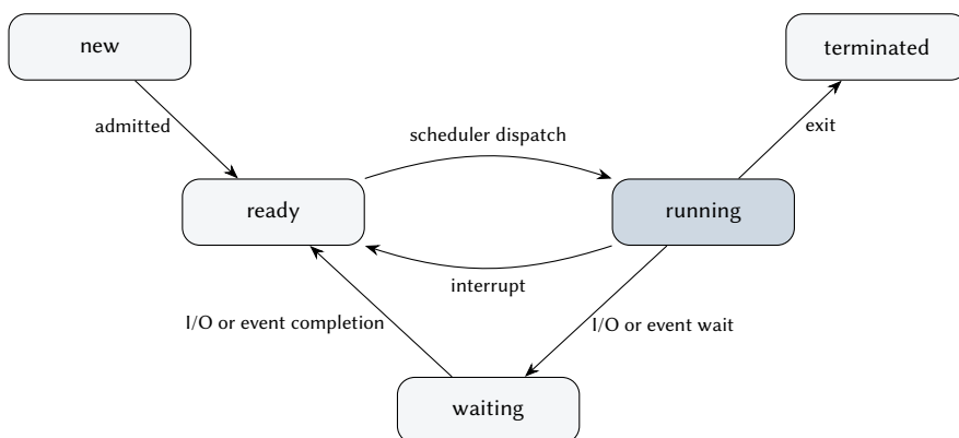
Figure 2.5: Process states and the transitions between them.
