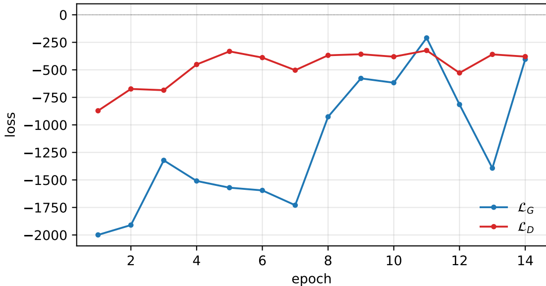
cDCGAN losses (incomplete: 14/50 epochs)
