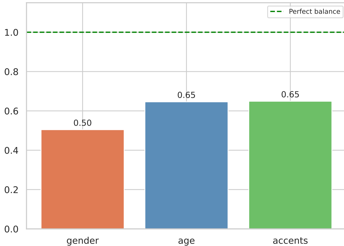
Normalised Entropy (↑ better)
