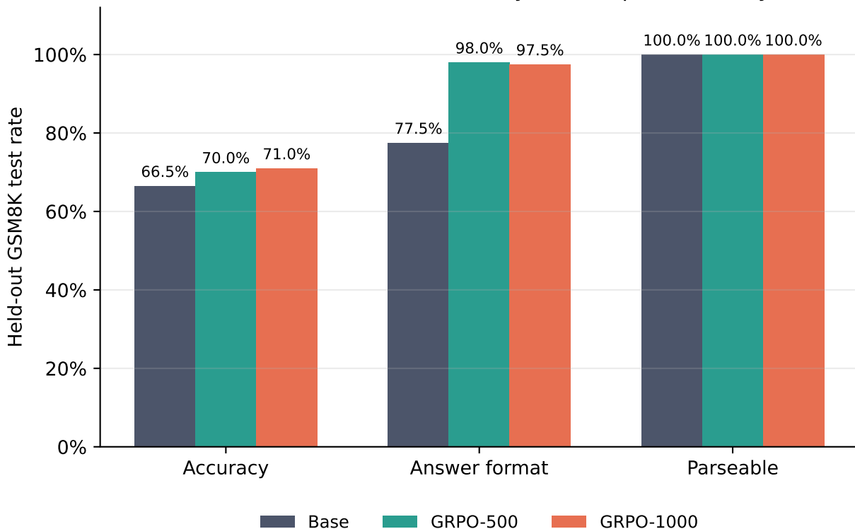
Held-out evaluation: accuracy and output reliability
