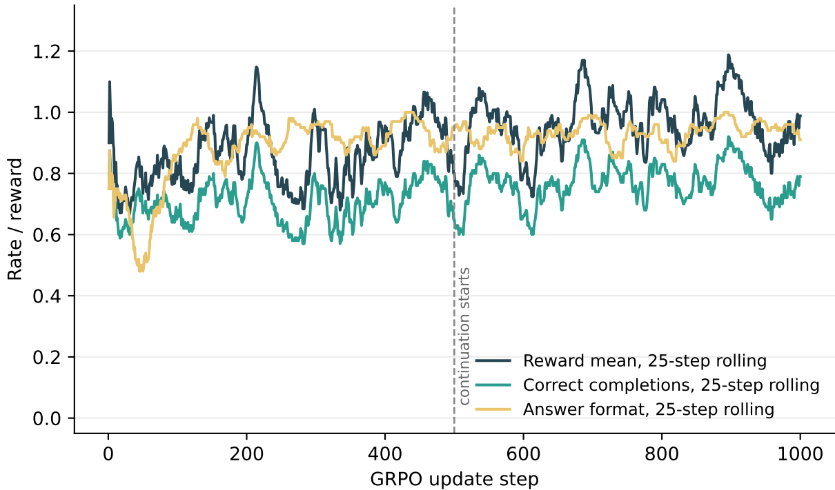
Training dynamics across 1000 updates
