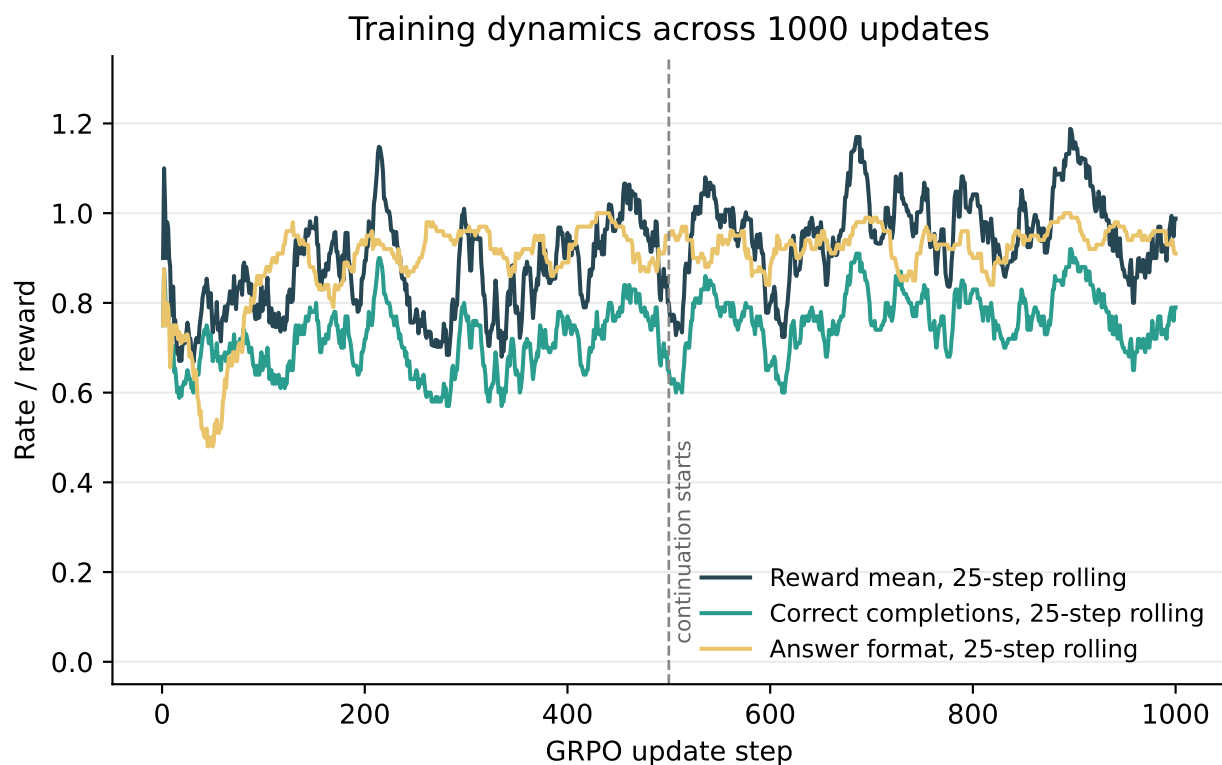
Figure 4: Rolling training curves across 1000 updates. The vertical line marks the transition from the first stage to continuation training.
