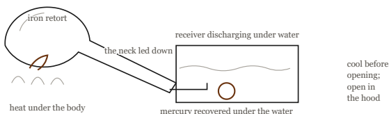
FIG. 1 — THE CLOSED RETORT TRAIN FOR AMALGAM RECOVERY. The apparatus the procedure above describes, drawn as a working diagram: the charge of stiff amalgam in an iron retort, heat under the body, the neck led downward into a receiver that discharges under water, and the mercury condensing to be caught there — closed being the whole point. The alternative, heating the amalgam in the open and breathing what comes off, is the exact mechanism the Warning above names as the direct cause of chronic mercury poisoning in artisanal mining communities today. The vessel is allowed to cool before it is opened, and it is opened in the hood. Drawn for this book from the procedure in the text.
