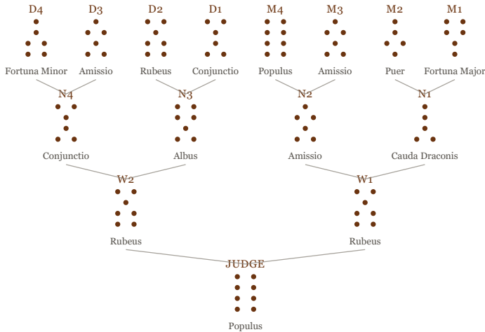
FIG. 3 — A SHIELD, WORKED. Four Mothers cast for illustration — Fortuna Major, Puer, Amissio, Populus — and everything below them computed by the rules above. The Daughters transpose the Mothers' rows; each Niece adds a pair; the Witnesses and Judge fold the rest down. The Judge here is Populus, the crowd: an answer of "as things commonly go," with the right Witness Rubeus warning where the querent's own conduct sits in it. Every figure below the top row is forced — redo the arithmetic and you must get the same chart. The generating code for this diagram computed it the same way, so the figure is correct by construction.
