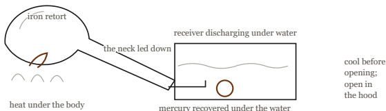
FIG. 1. THE CLOSED RETORT TRAIN FOR AMALGAM RECOVERY. The apparatus the procedure above describes, drawn as a working diagram: the charge of stiff amalgam in an iron retort, heat under the body, the neck led downward into a receiver that discharges under water, and the mercury condensing to be caught there: closed being the whole point. The alternative, heating the amalgam in the open and breathing what comes off, is the exact mechanism the Warning above names as the direct cause of chronic mercury poisoning in artisanal mining communities today. The vessel is allowed to cool before it is opened, and it is opened in the hood. Drawn for this book from the procedure in the text.
